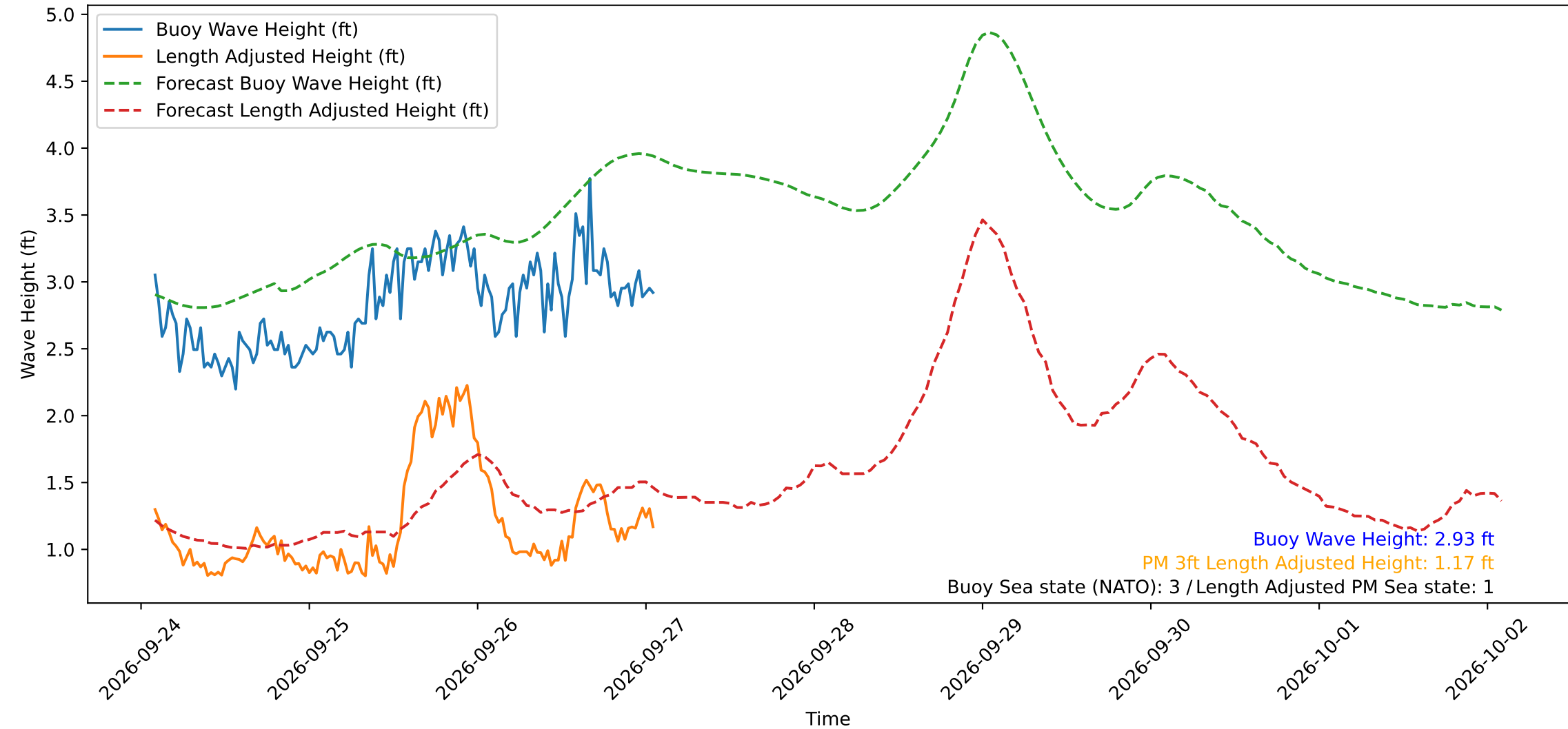
Wave Heights over Time for Oceanside Harbor at 2026-09-27 02:00:29
