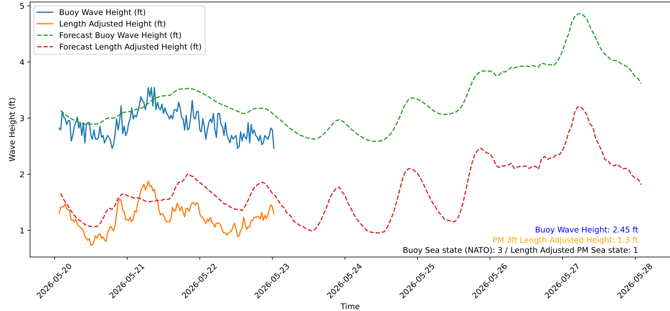
Wave Heights over Time for Green Beach at 2026-05-23 01:31:14
