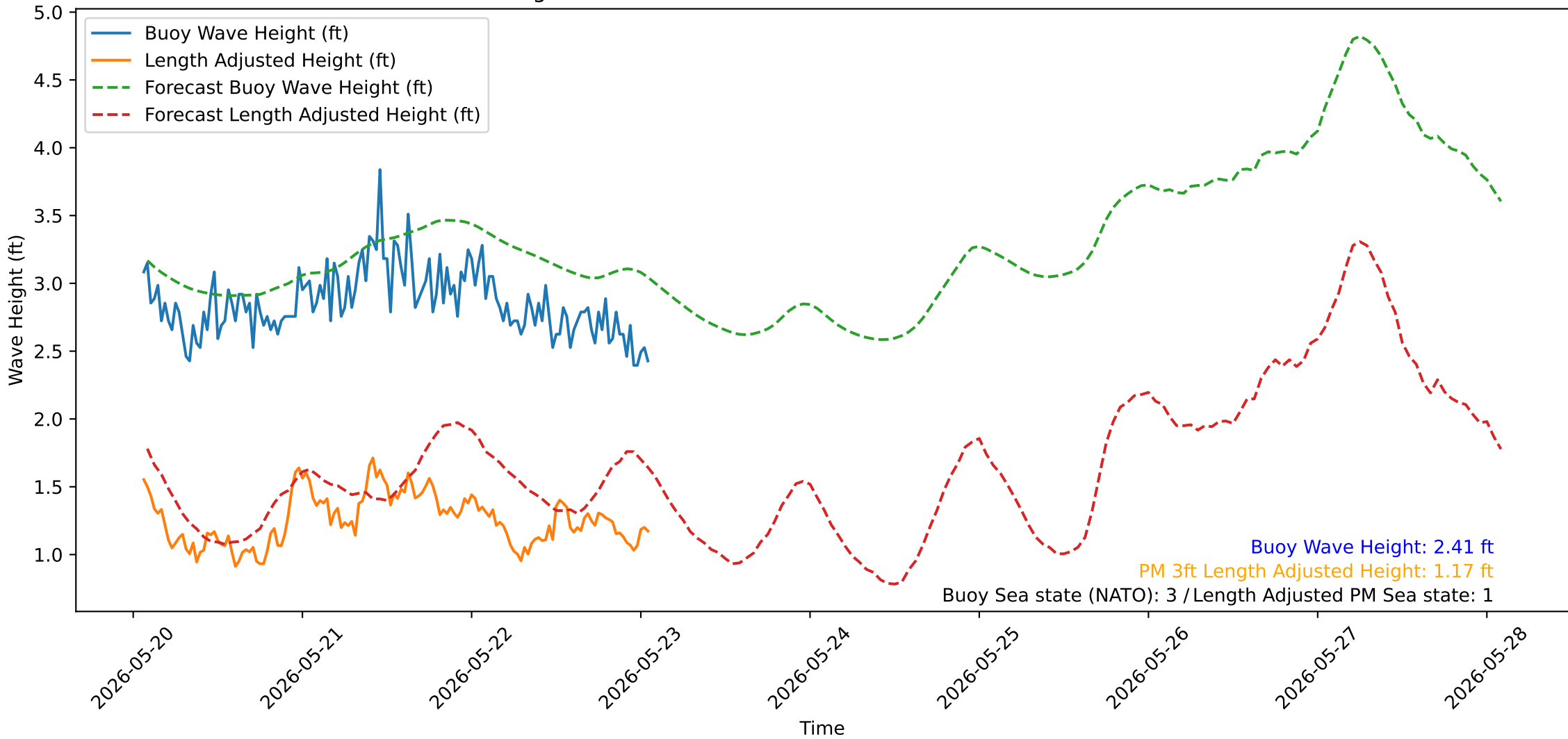
Wave Heights over Time for Oceanside Harbor at 2026-05-23 01:30:32
