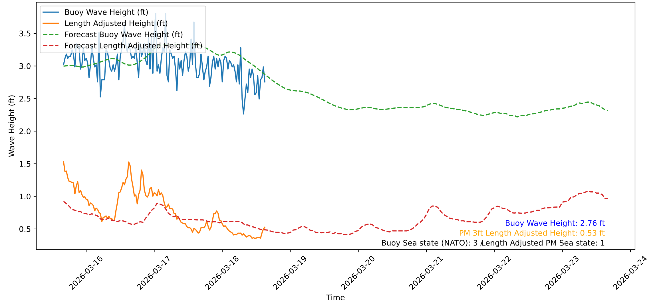
Wave Heights over Time for Red Beach at 2026-03-18 15:50:48
