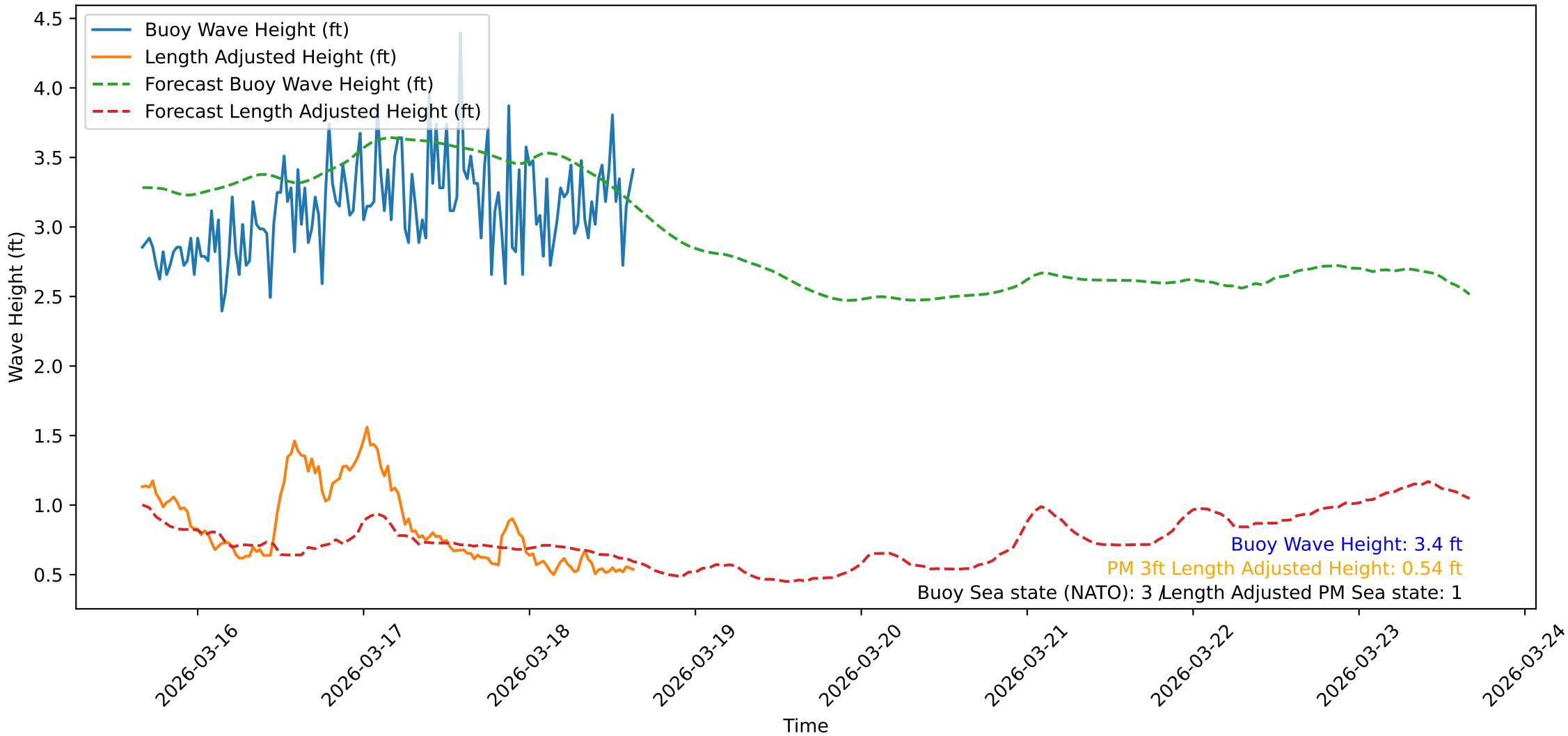
Wave Heights over Time for Oceanside Harbor at 2026-03-18 15:50:32
