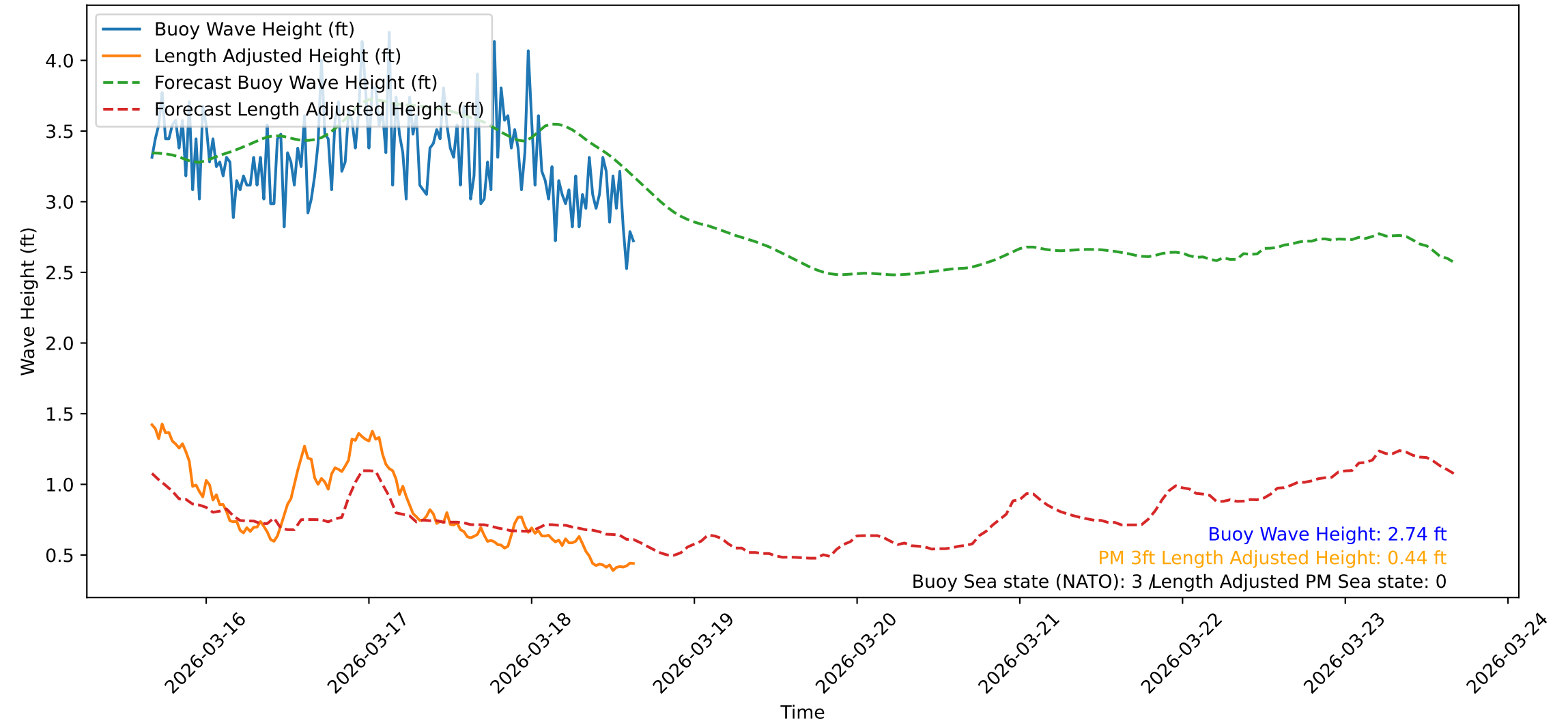
Wave Heights over Time for Green Beach at 2026-03-18 15:51:11
