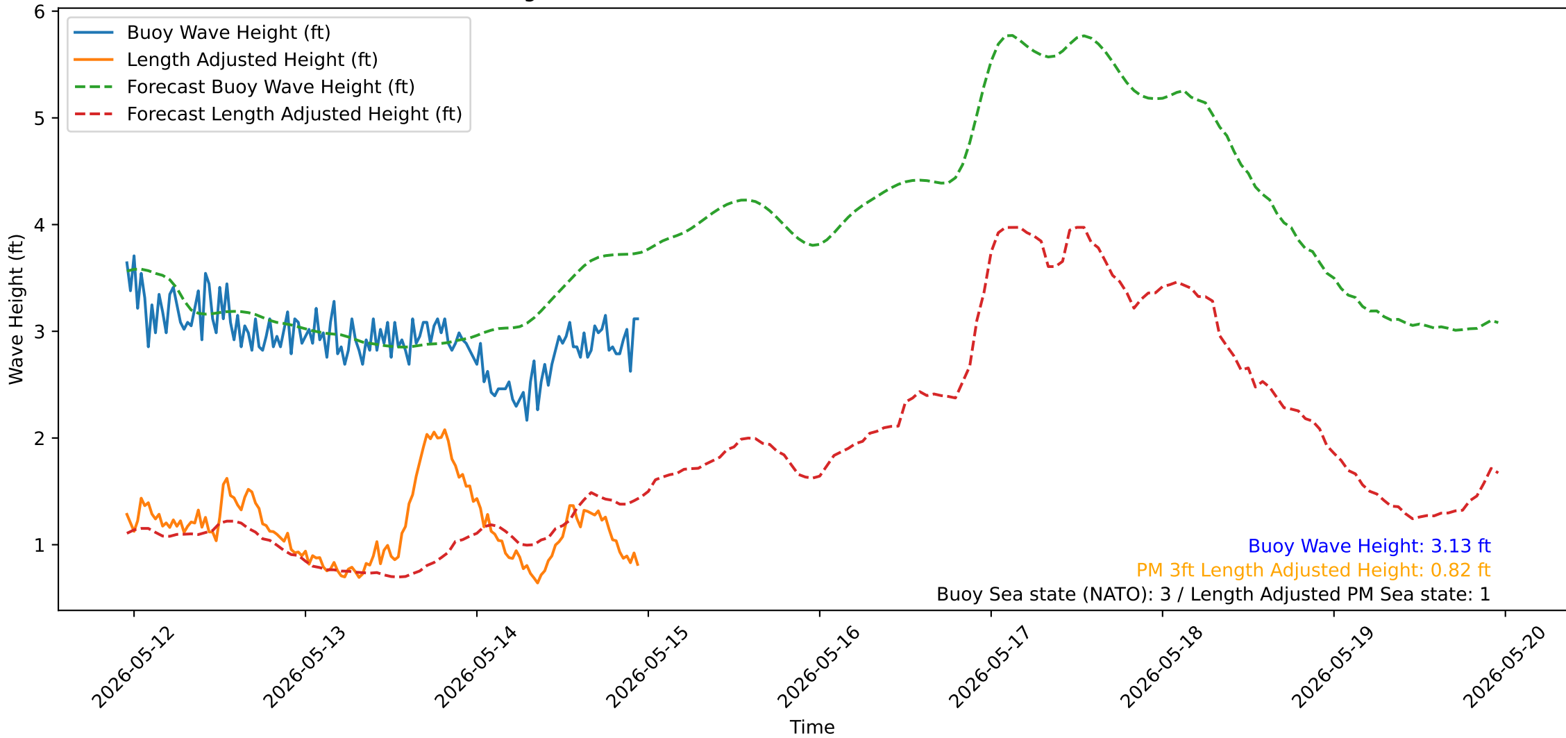
Wave Heights over Time for Oceanside Harbor at 2026-05-14 23:00:32
