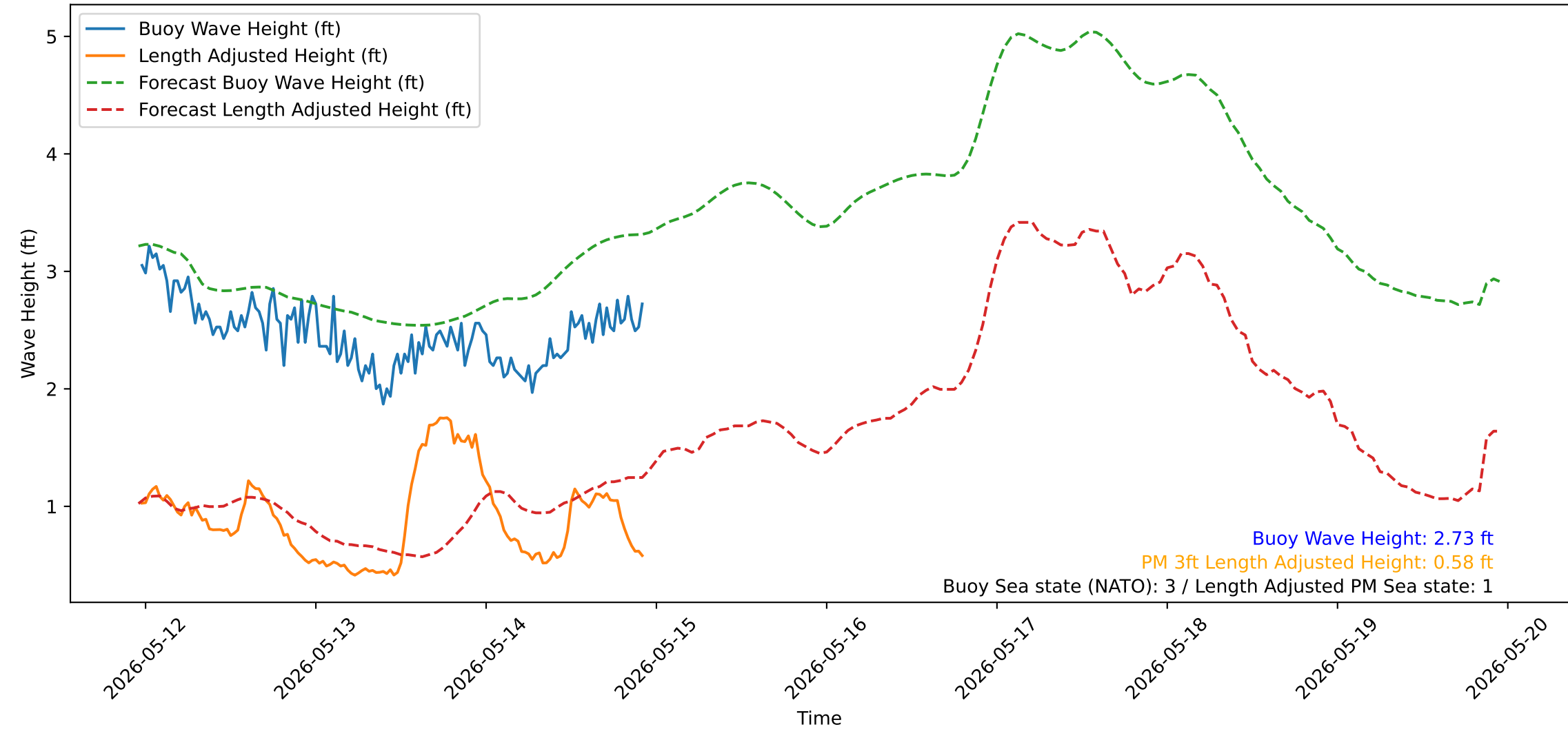
Wave Heights over Time for Red Beach at 2026-05-14 23:00:52
