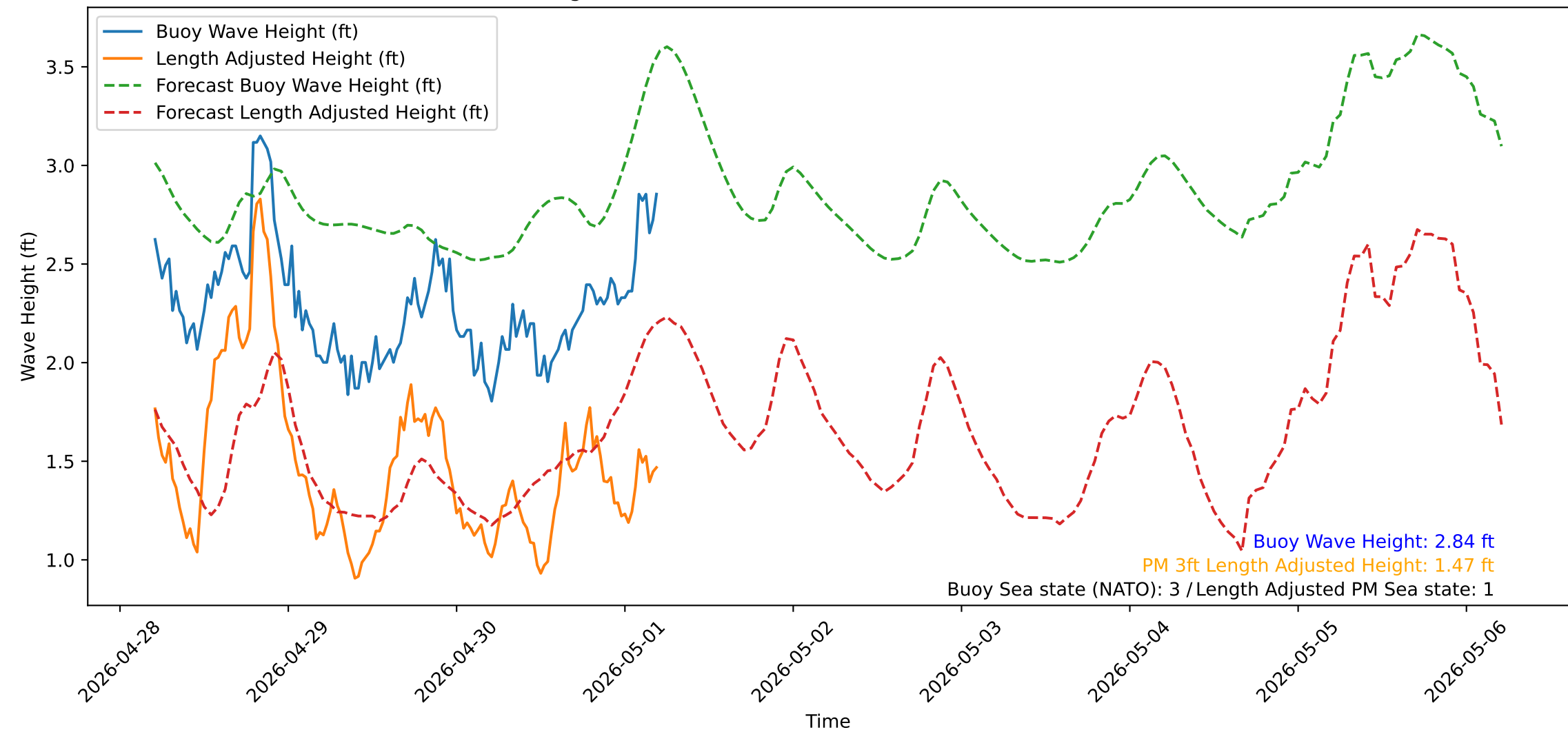
Wave Heights over Time for Green Beach at 2026-05-01 05:11:12
