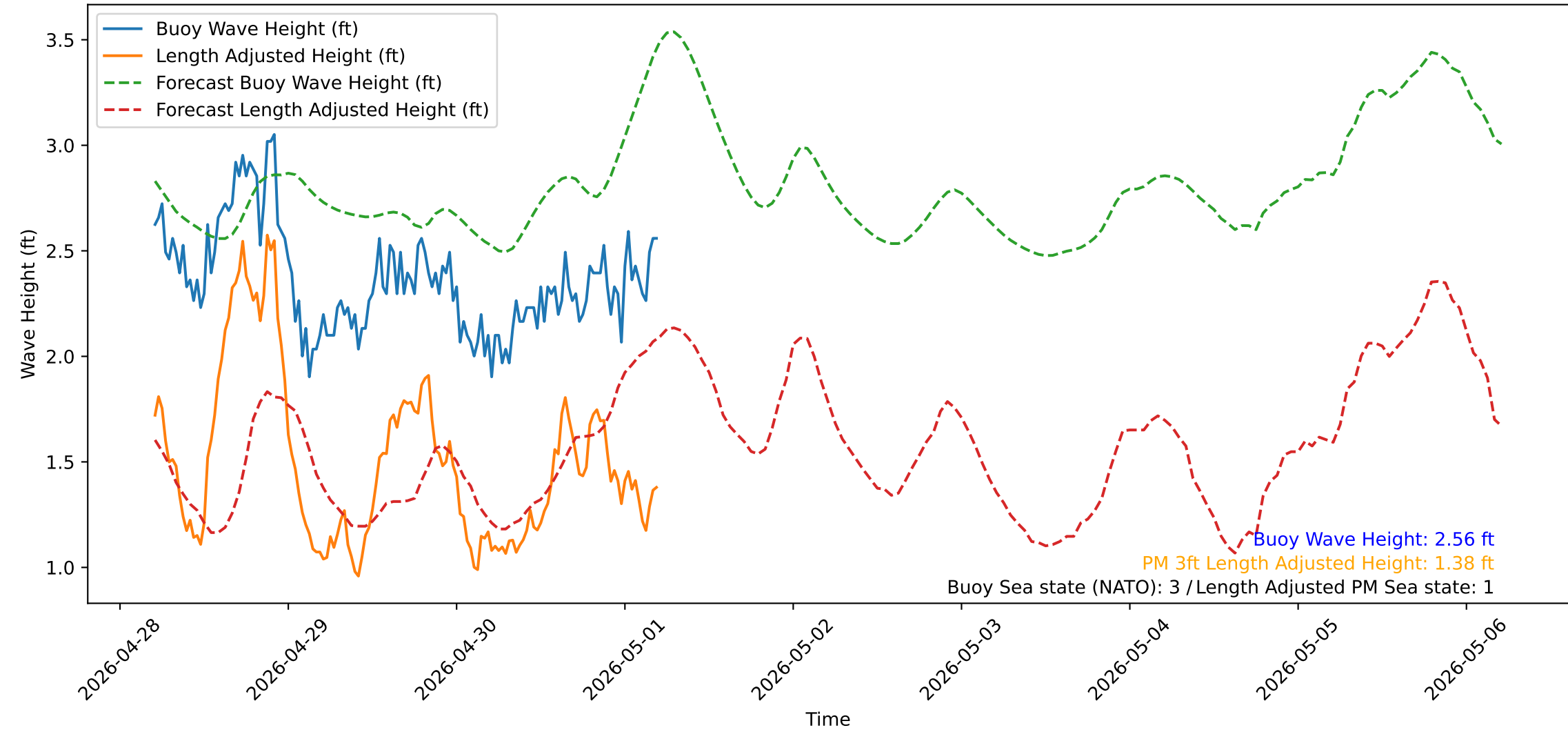
Wave Heights over Time for Oceanside Harbor at 2026-05-01 05:10:31
