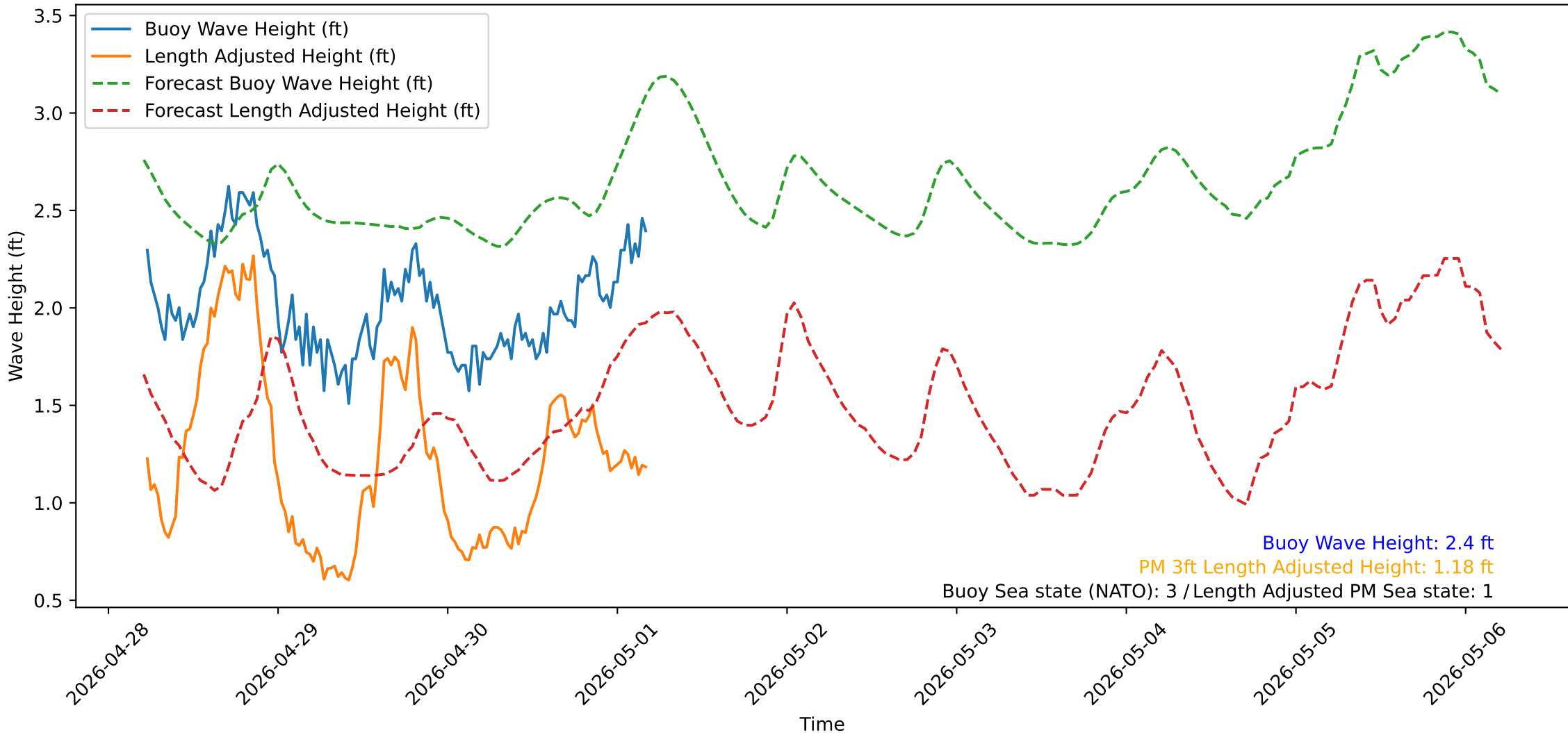
Wave Heights over Time for Red Beach at 2026-05-01 05:10:50
