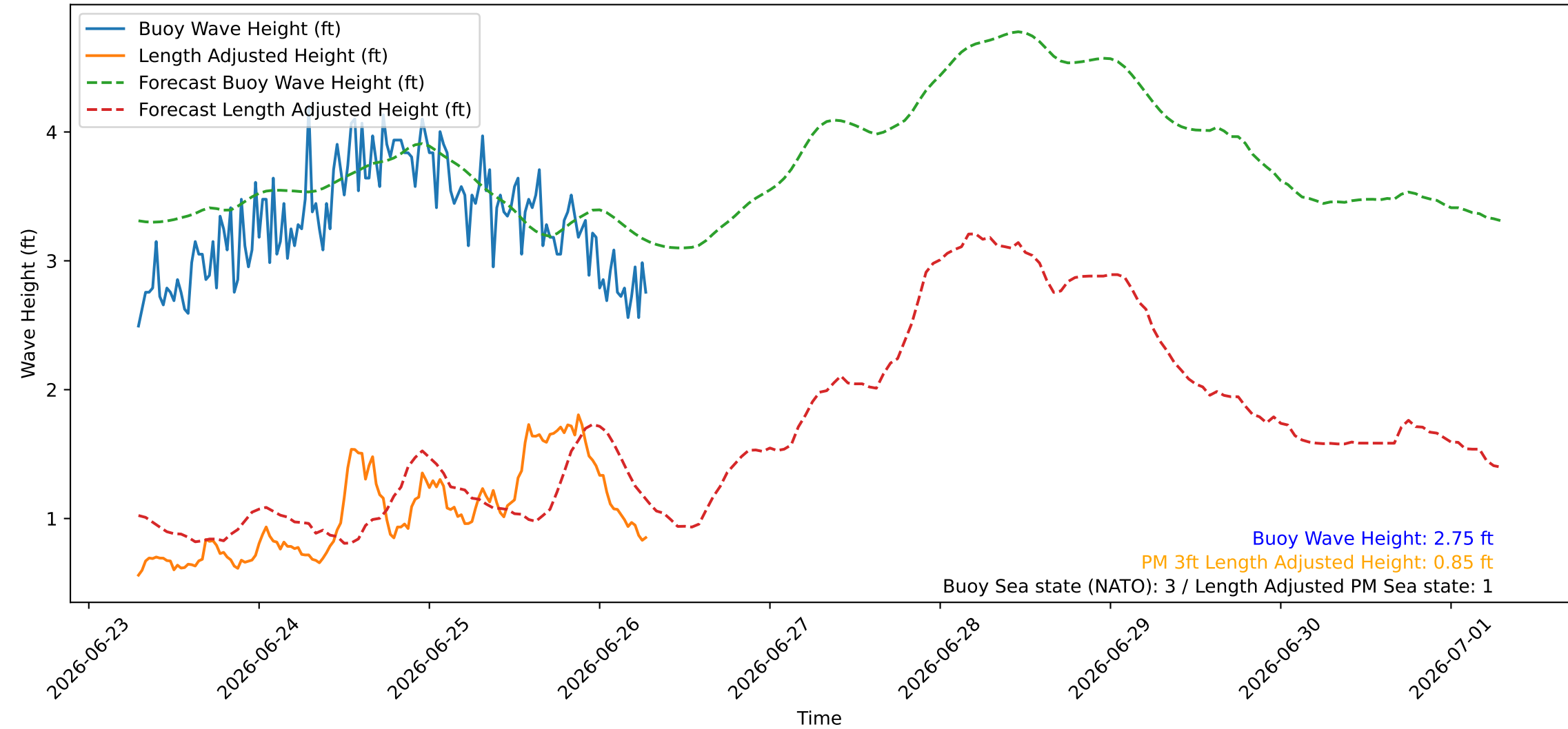
Wave Heights over Time for Green Beach at 2026-06-26 07:11:08
