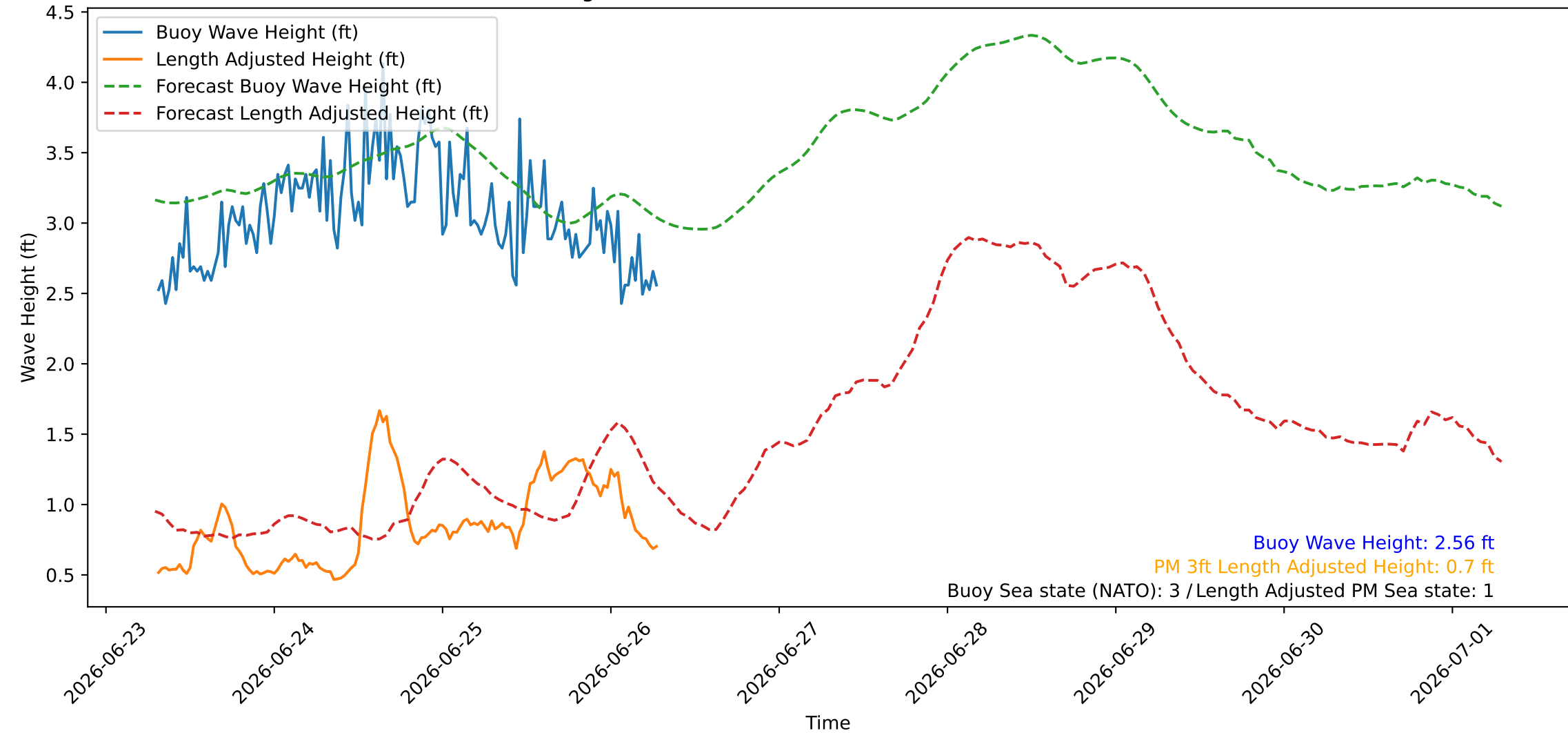
Wave Heights over Time for Red Beach at 2026-06-26 07:10:45
