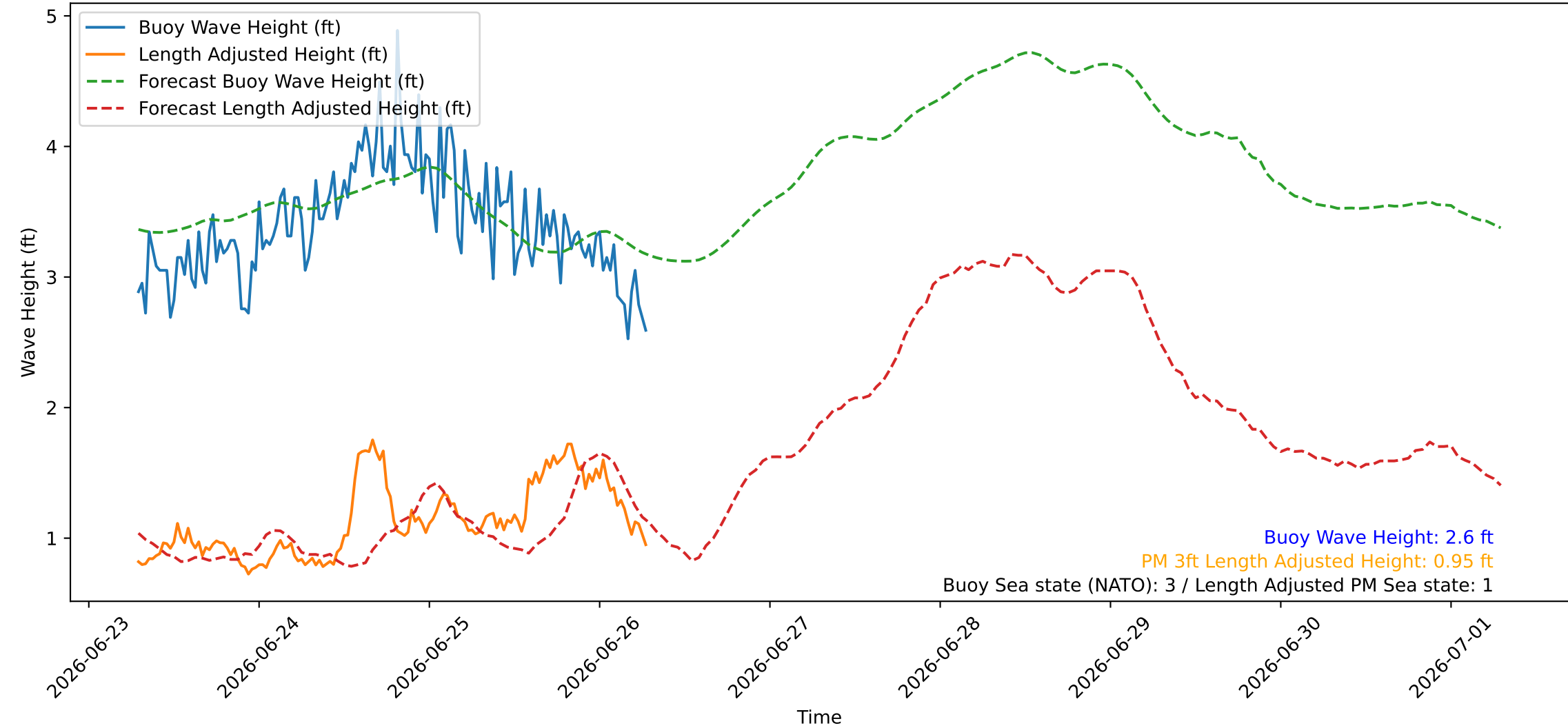
Wave Heights over Time for Oceanside Harbor at 2026-06-26 07:10:26
