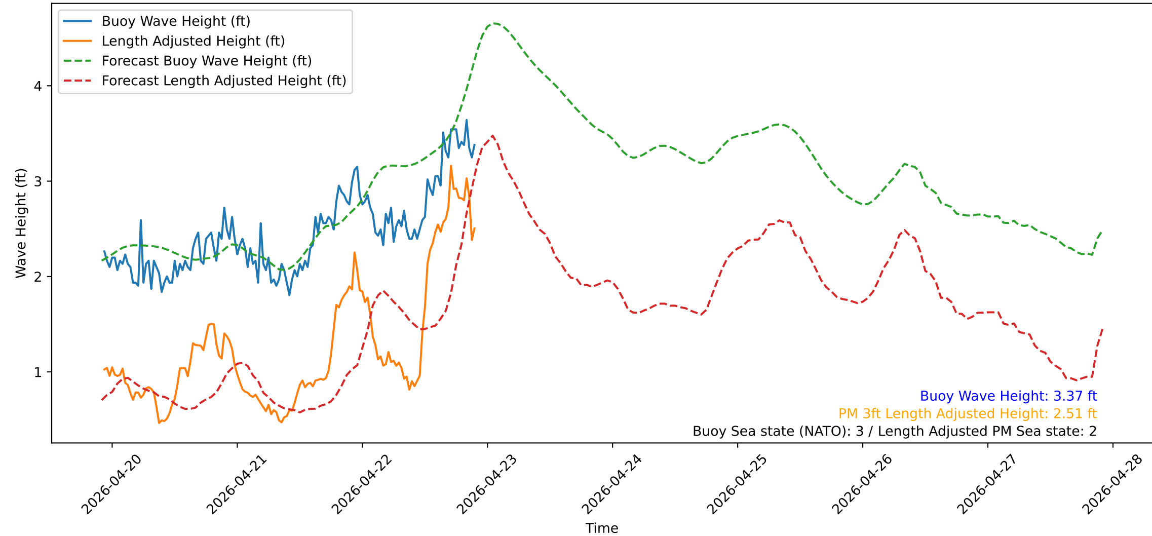
Wave Heights over Time for Red Beach at 2026-04-22 22:20:51
