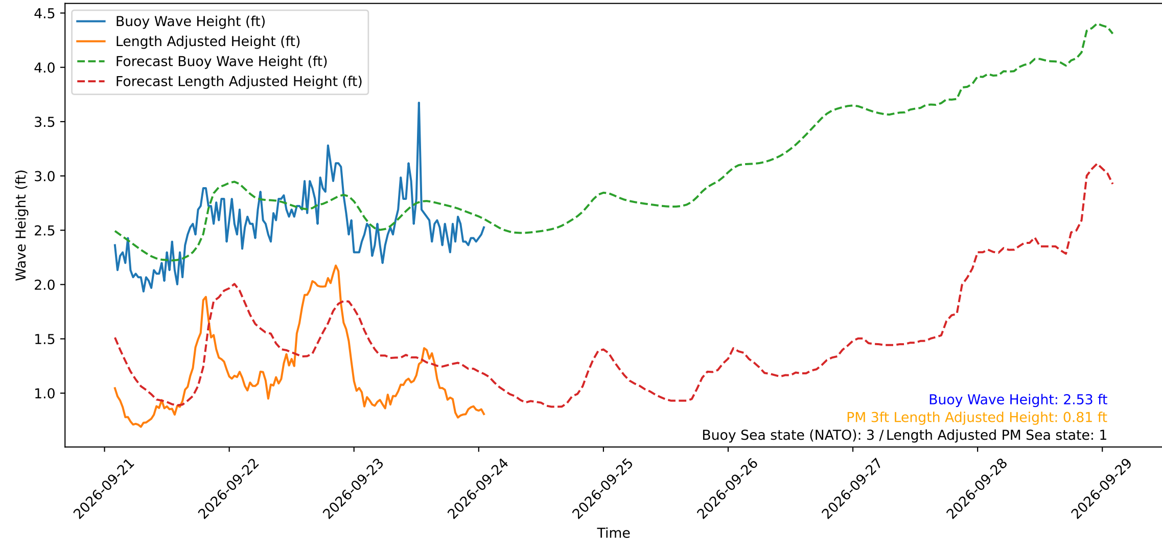
Wave Heights over Time for Red Beach at 2026-09-24 01:40:49
