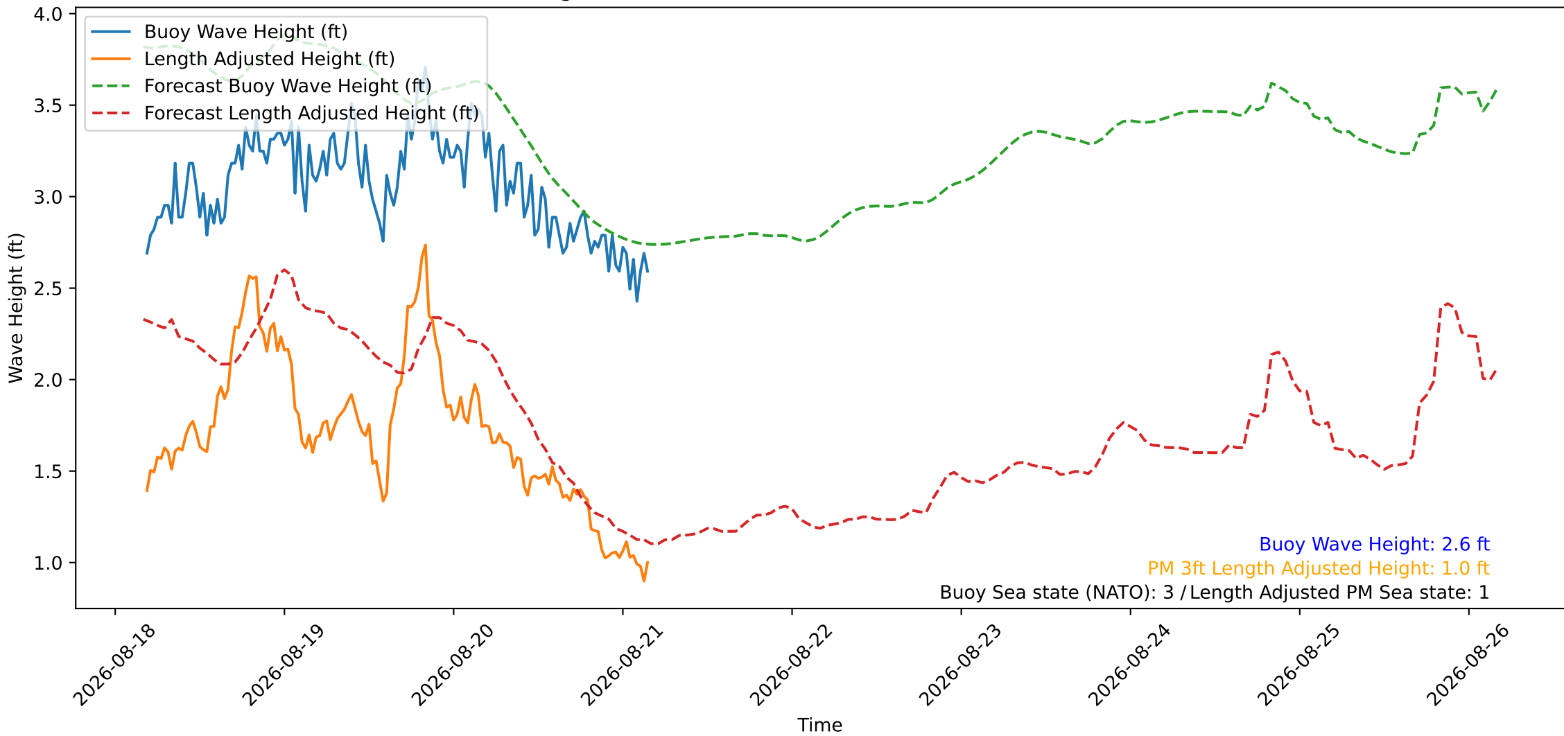
Wave Heights over Time for Green Beach at 2026-08-21 04:21:11
