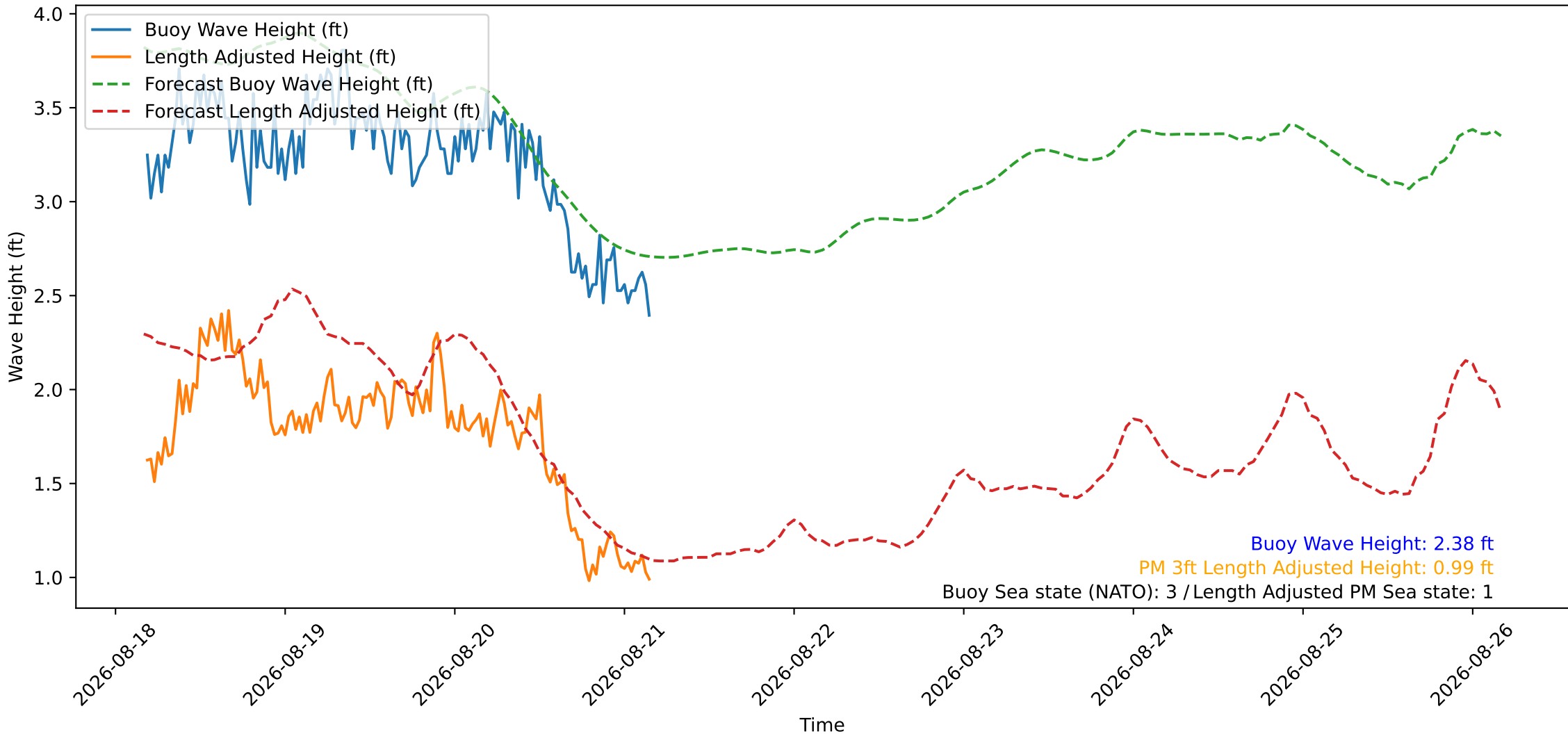
Wave Heights over Time for Oceanside Harbor at 2026-08-21 04:20:26
