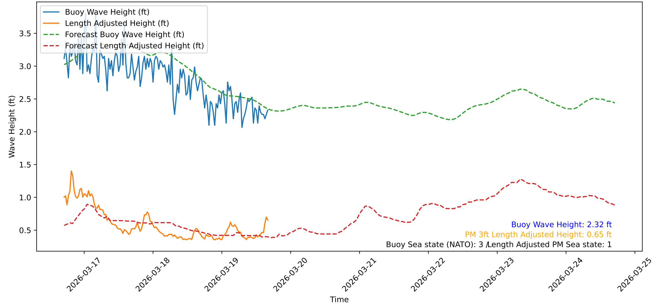
Wave Heights over Time for Red Beach at 2026-03-19 16:40:47
