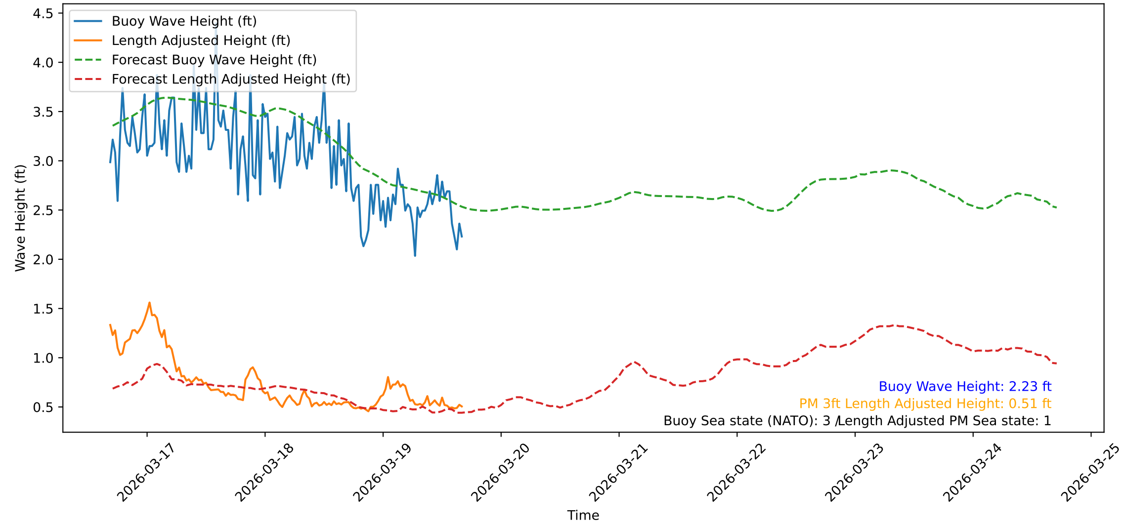
Wave Heights over Time for Oceanside Harbor at 2026-03-19 16:40:31
