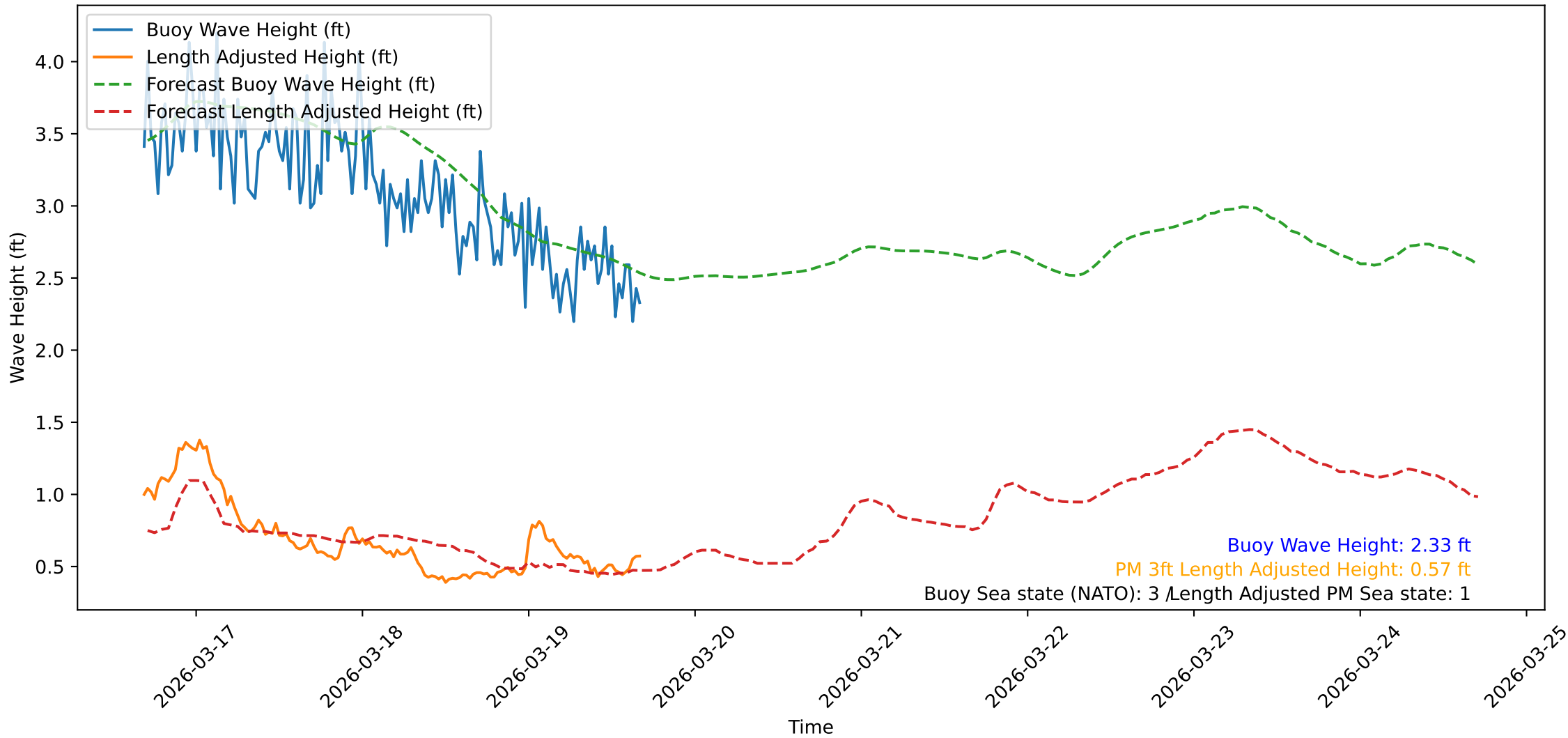
Wave Heights over Time for Green Beach at 2026-03-19 16:41:09
