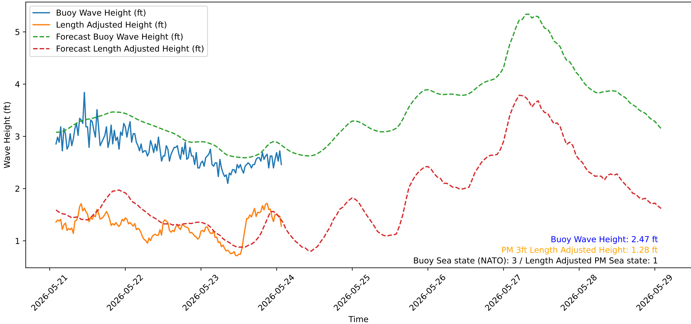
Wave Heights over Time for Oceanside Harbor at 2026-05-24 02:00:32
