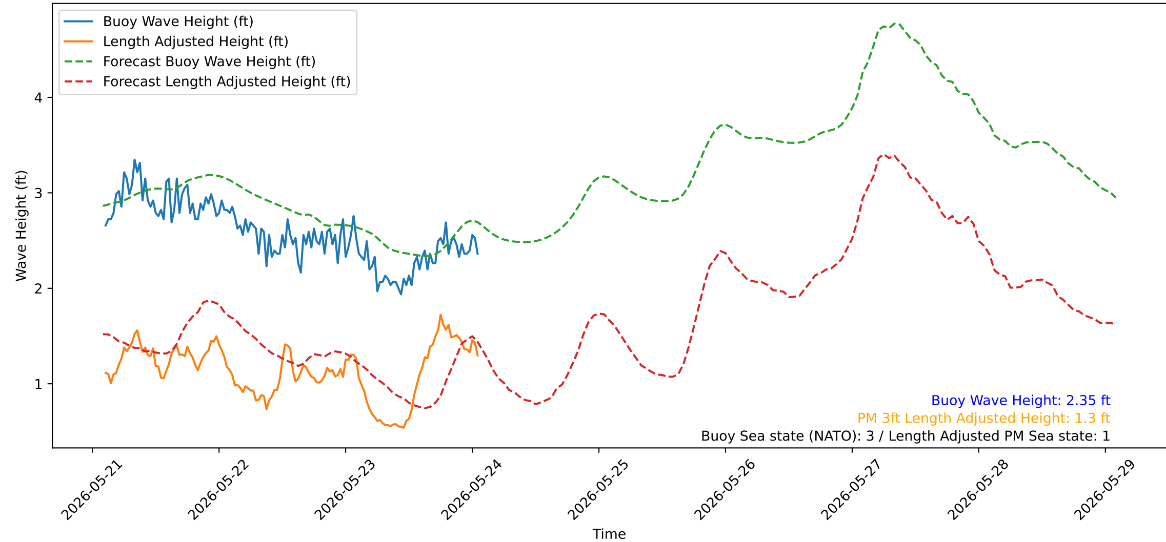
Wave Heights over Time for Red Beach at 2026-05-24 02:00:52
