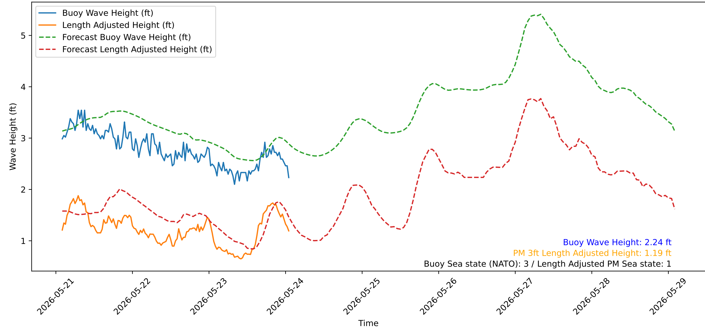
Wave Heights over Time for Green Beach at 2026-05-24 02:01:14
