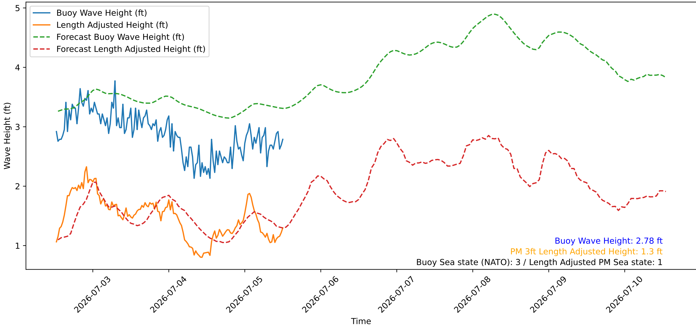
Wave Heights over Time for Oceanside Harbor at 2026-07-05 12:30:28
