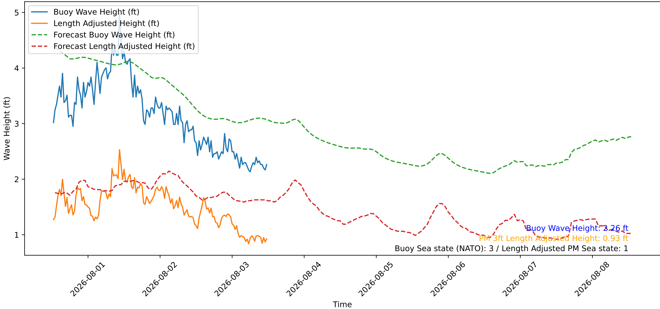
Wave Heights over Time for Green Beach at 2026-08-03 12:31:07
