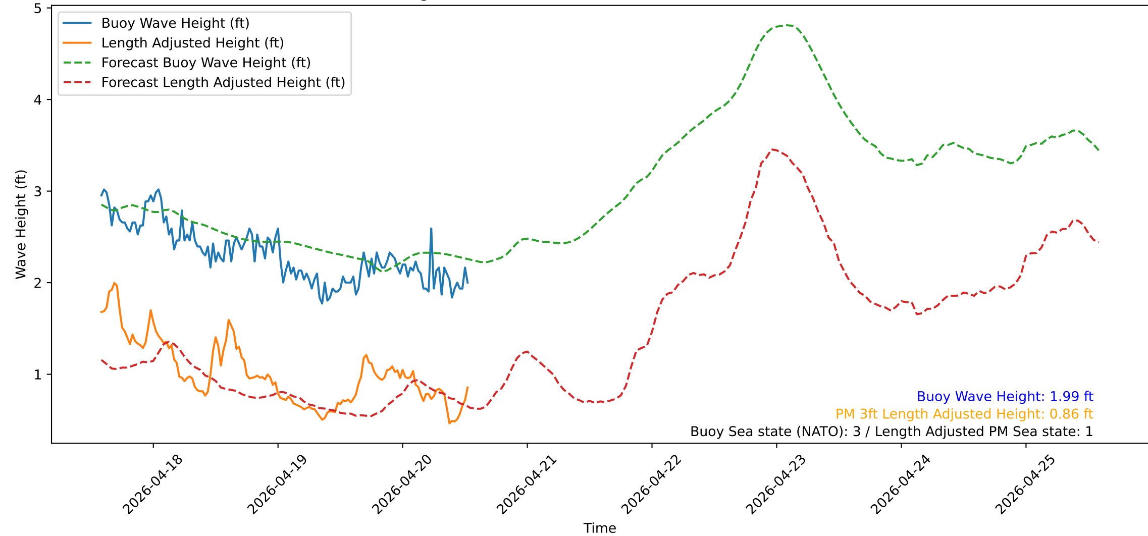
Wave Heights over Time for Red Beach at 2026-04-20 13:40:50
