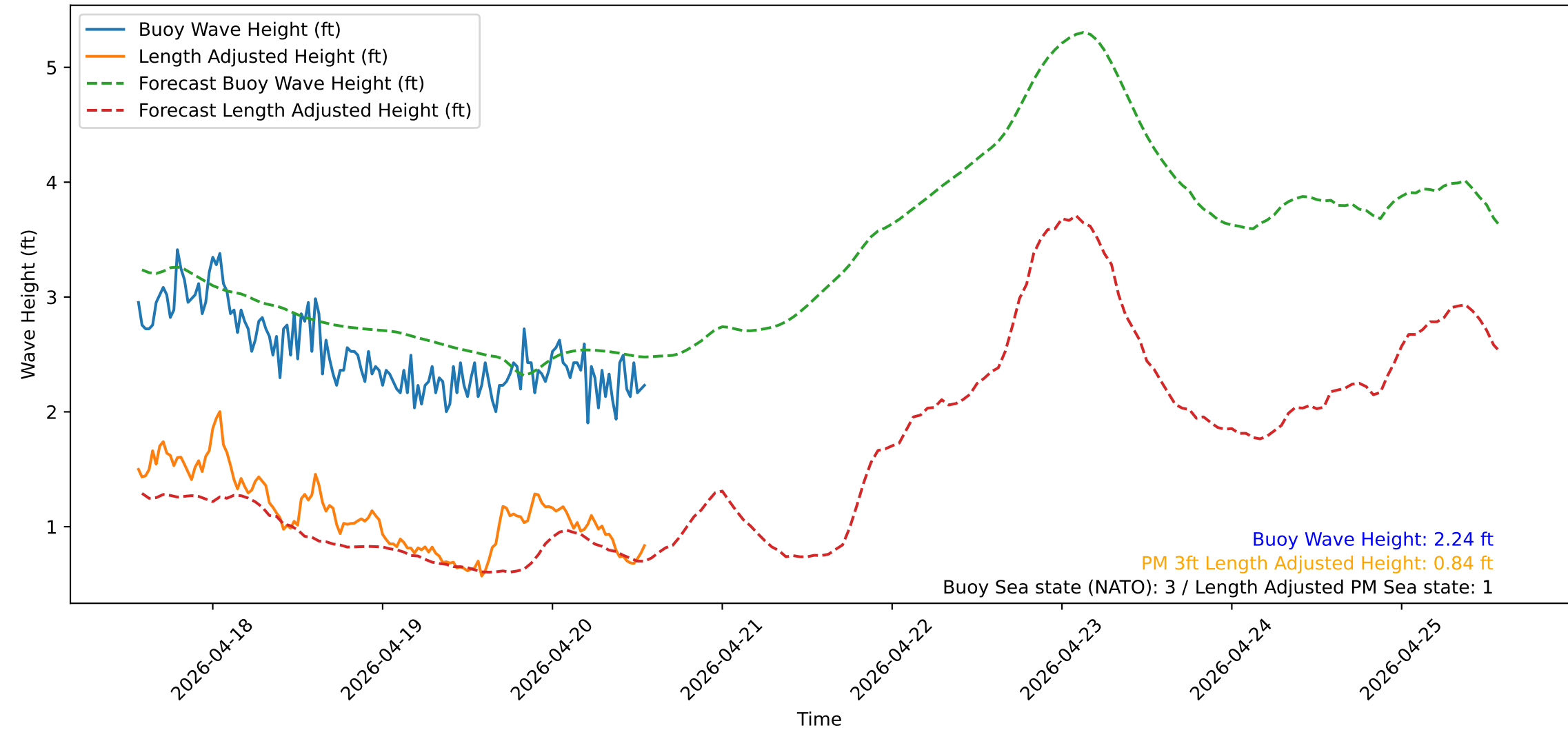
Wave Heights over Time for Oceanside Harbor at 2026-04-20 13:40:31
