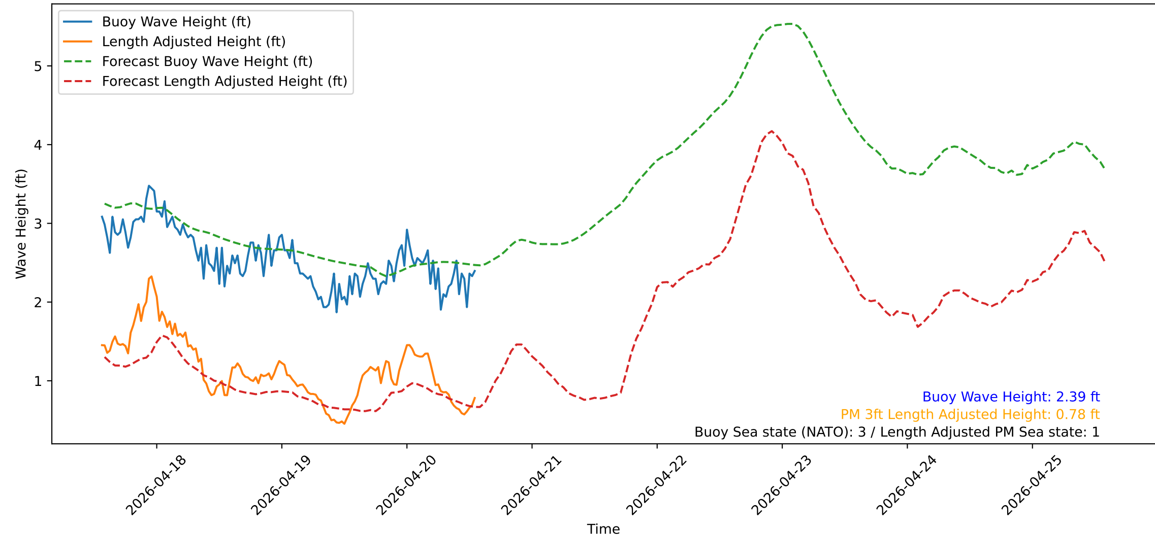
Wave Heights over Time for Green Beach at 2026-04-20 13:41:13
