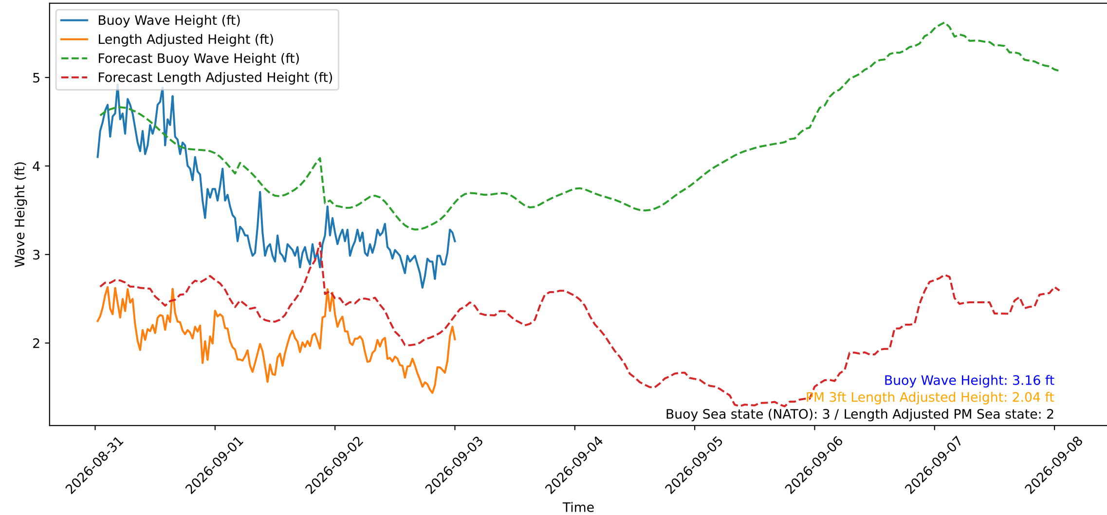
Wave Heights over Time for Oceanside Harbor at 2026-09-03 00:40:30
