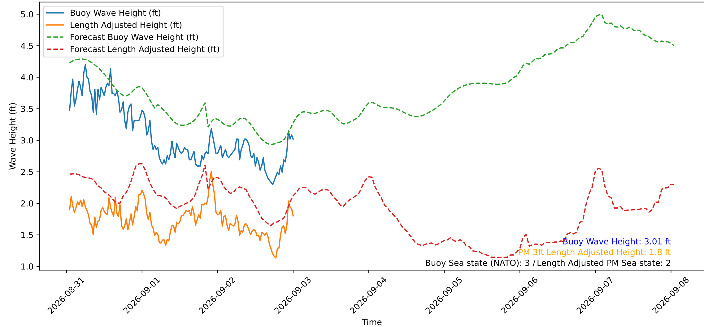
Wave Heights over Time for Red Beach at 2026-09-03 00:40:50
