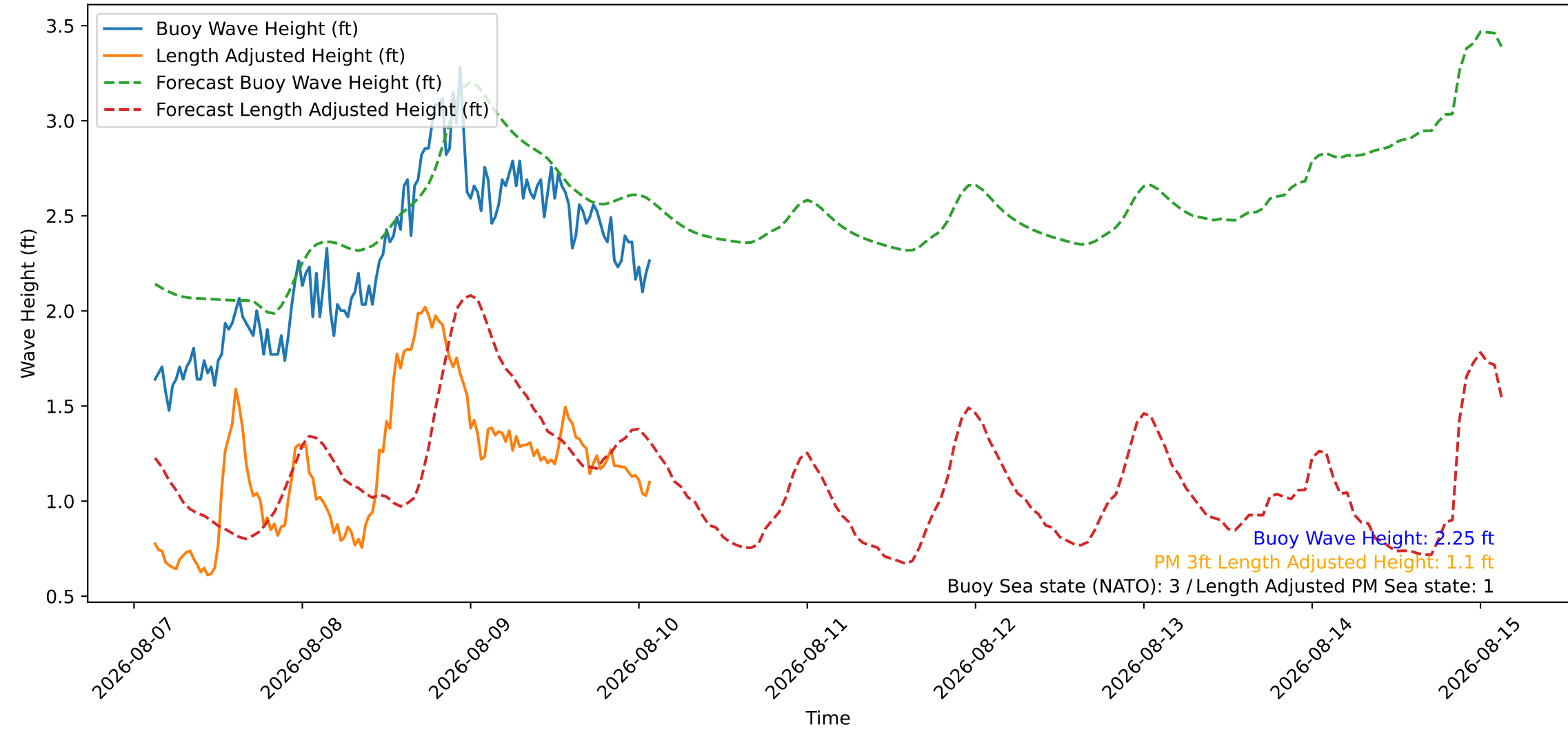
Wave Heights over Time for Red Beach at 2026-08-10 02:30:46
