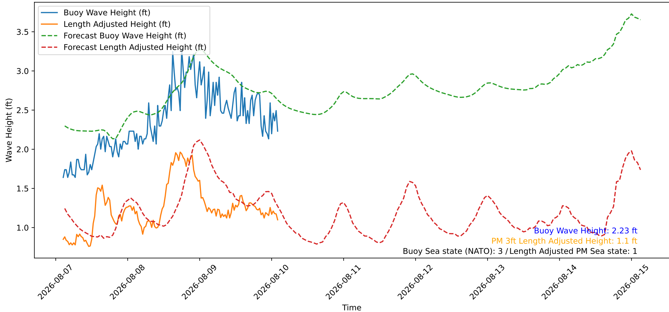
Wave Heights over Time for Oceanside Harbor at 2026-08-10 02:30:26
