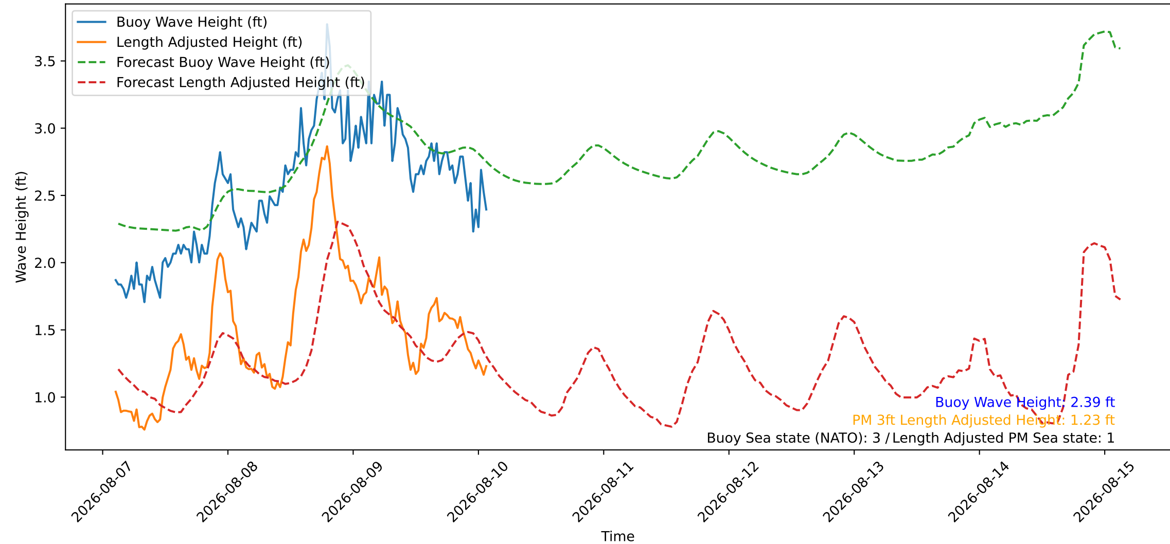
Wave Heights over Time for Green Beach at 2026-08-10 02:31:09
