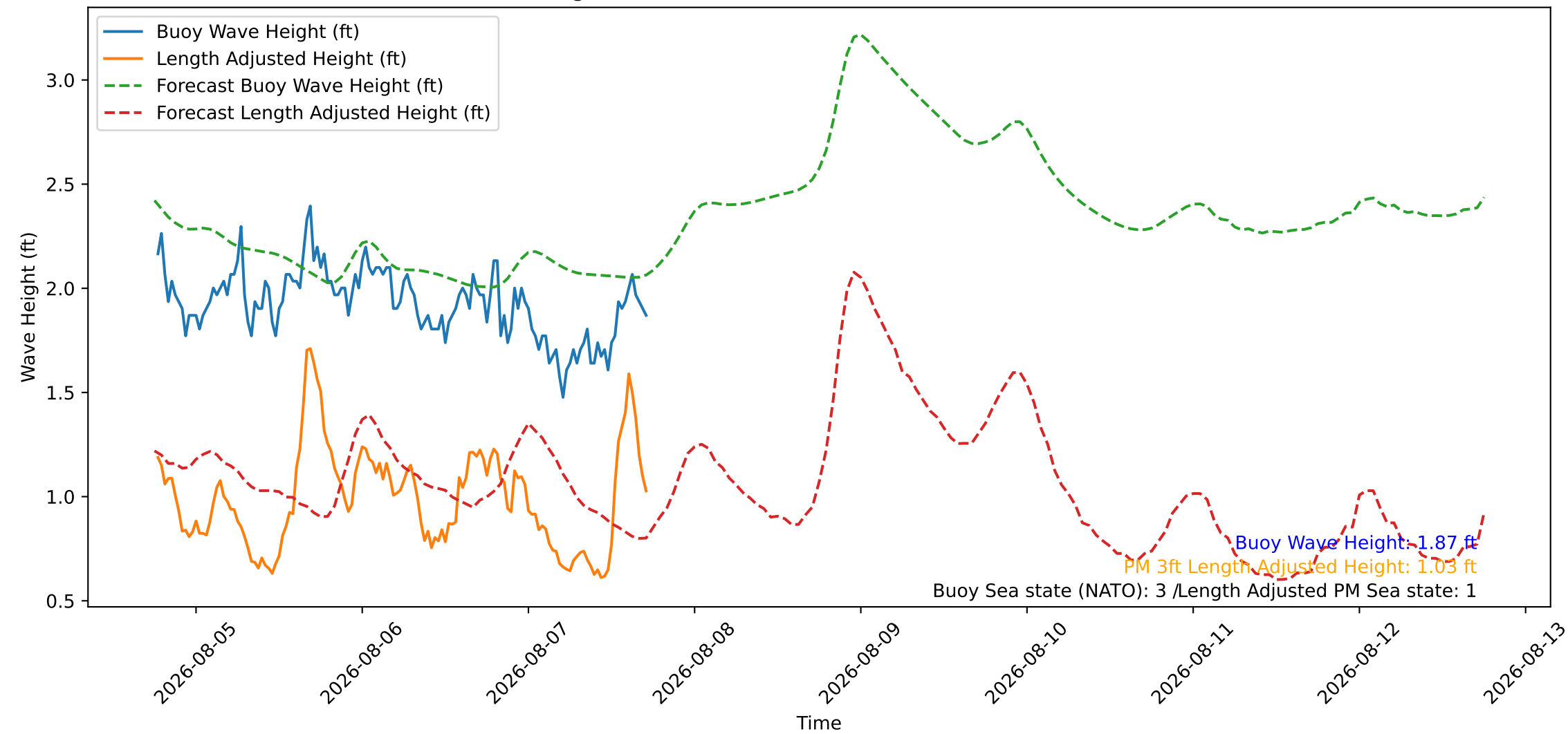
Wave Heights over Time for Red Beach at 2026-08-07 18:00:46
