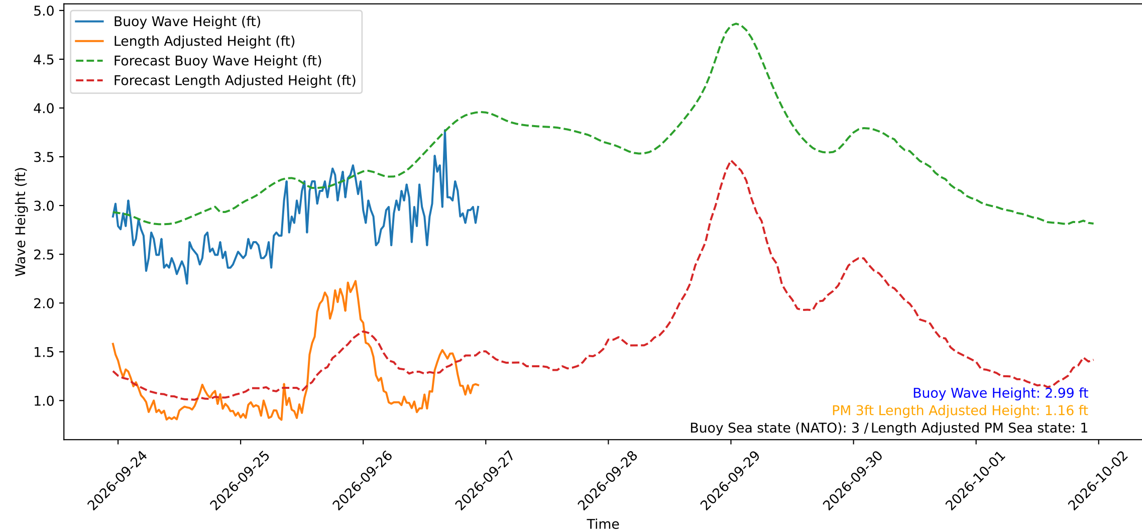
Wave Heights over Time for Oceanside Harbor at 2026-09-26 23:10:30
