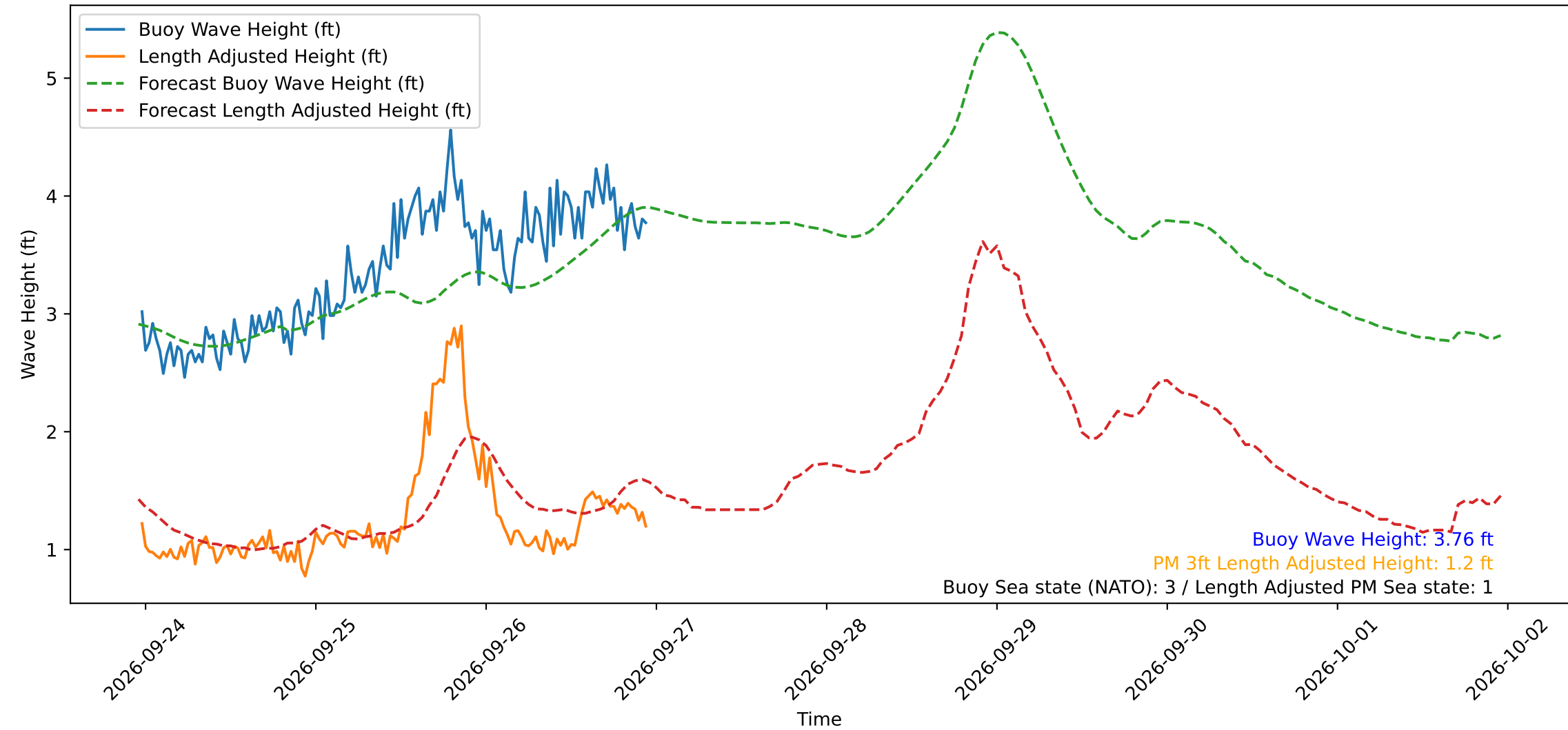
Wave Heights over Time for Green Beach at 2026-09-26 23:11:12
