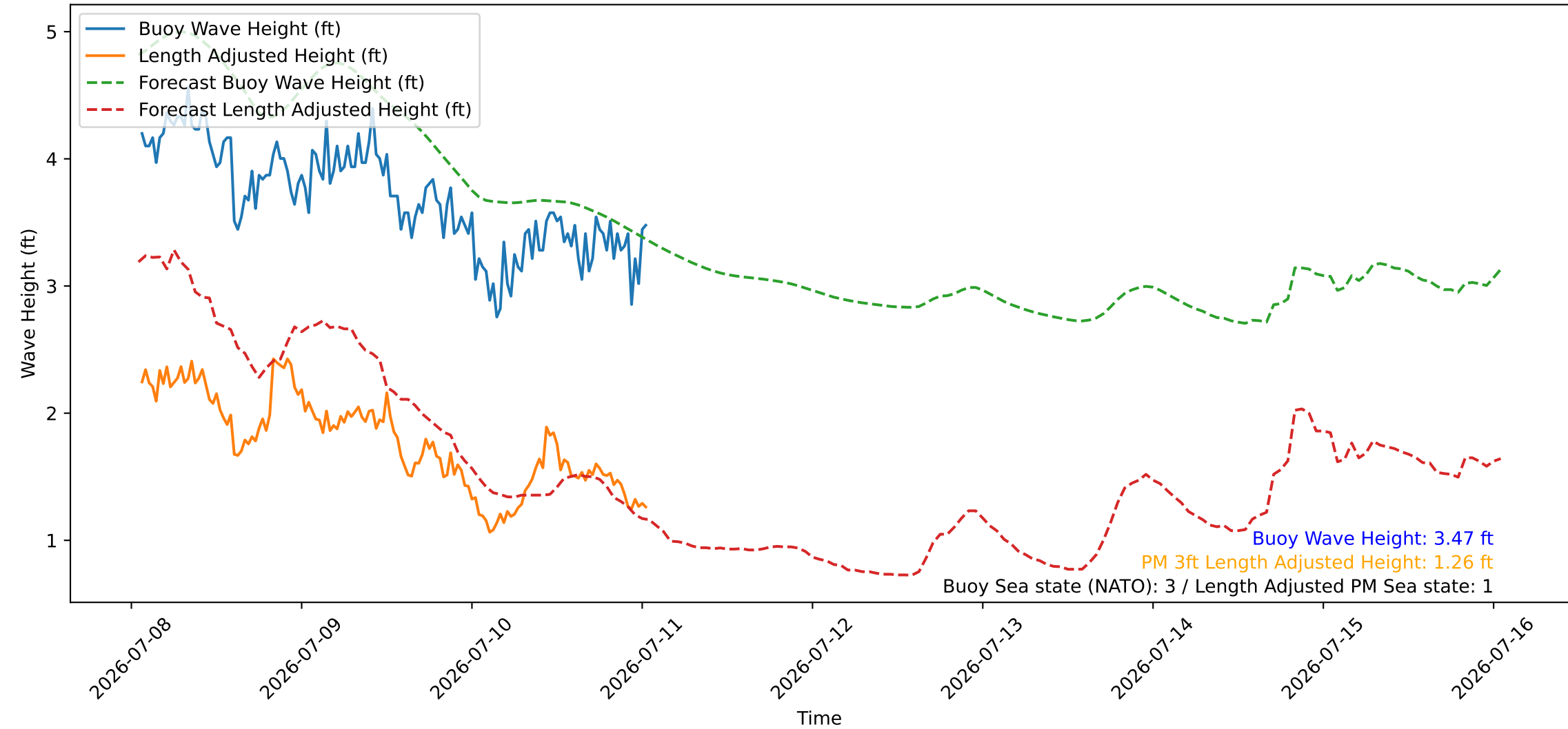
Wave Heights over Time for Green Beach at 2026-07-11 01:21:09
