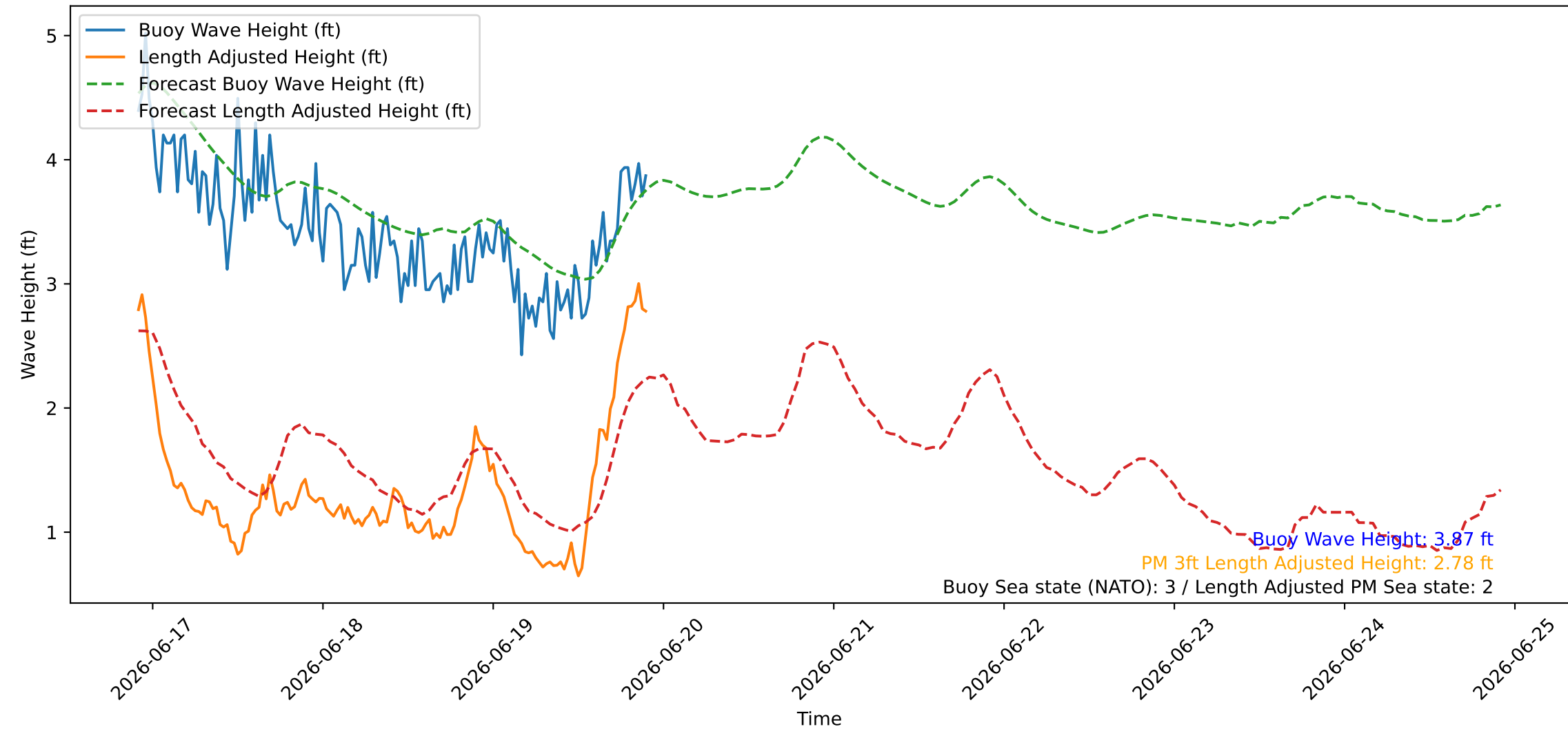
Wave Heights over Time for Green Beach at 2026-06-19 22:11:07
