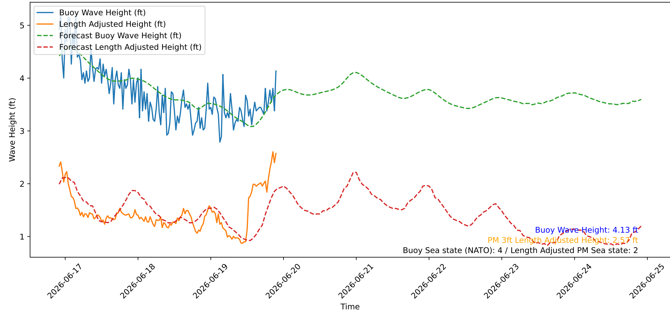
Wave Heights over Time for Oceanside Harbor at 2026-06-19 22:10:26
