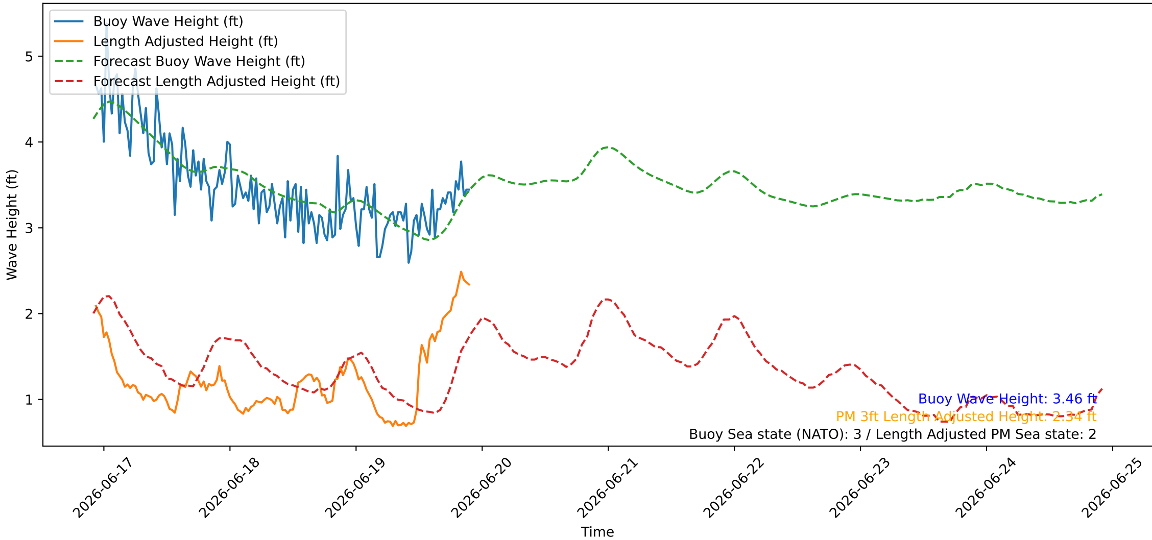
Wave Heights over Time for Red Beach at 2026-06-19 22:10:45
