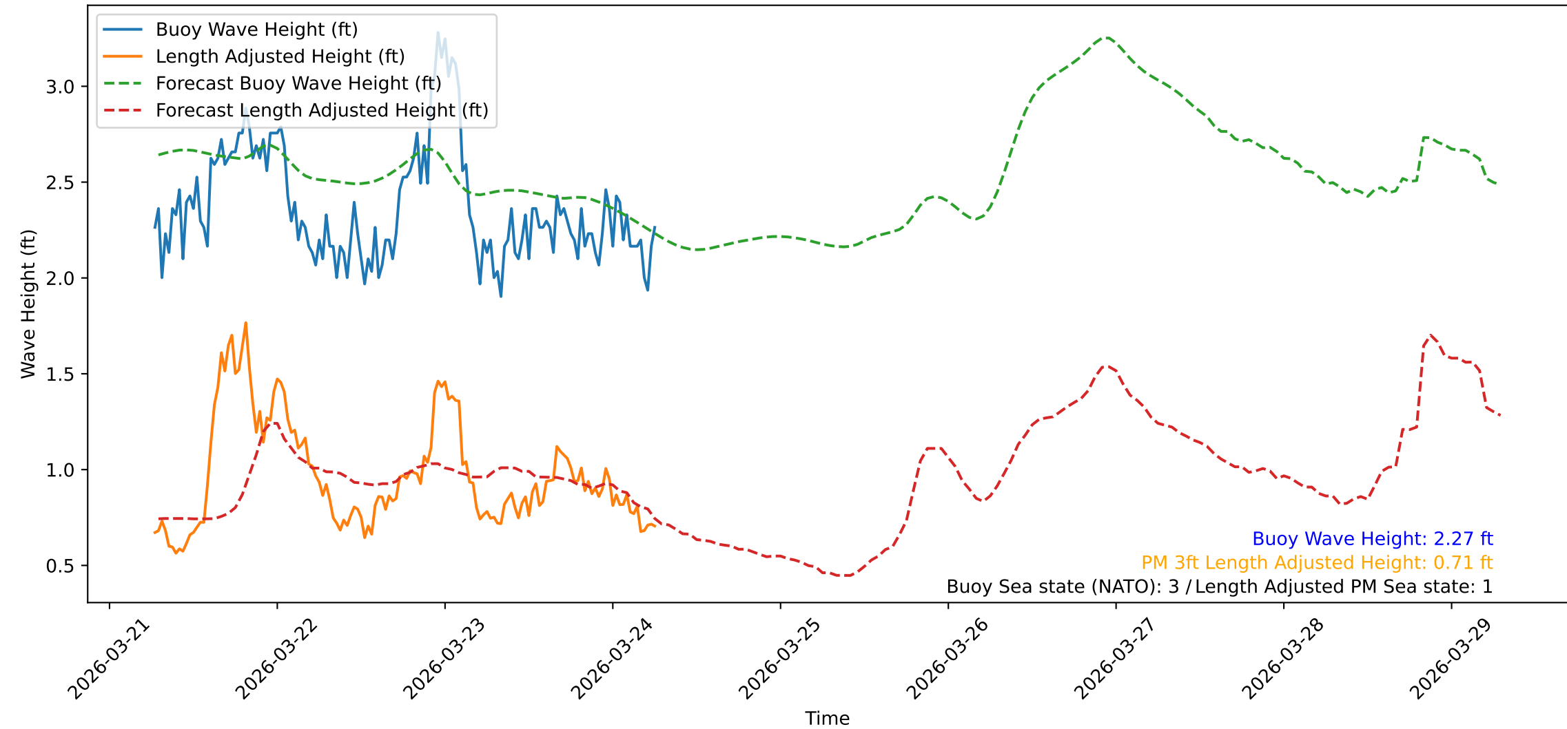
Wave Heights over Time for Green Beach at 2026-03-24 06:41:10
