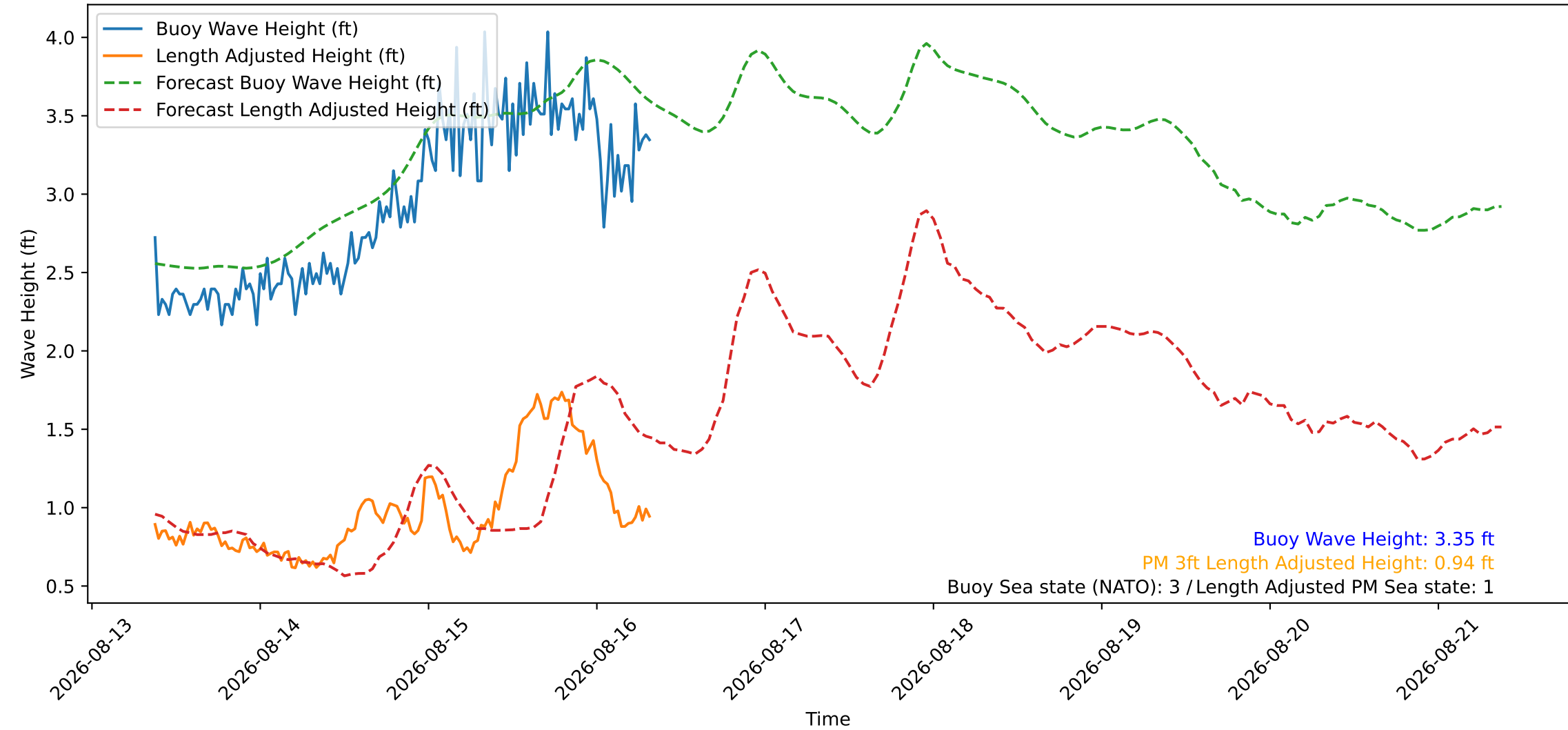
Wave Heights over Time for Red Beach at 2026-08-16 08:30:46
