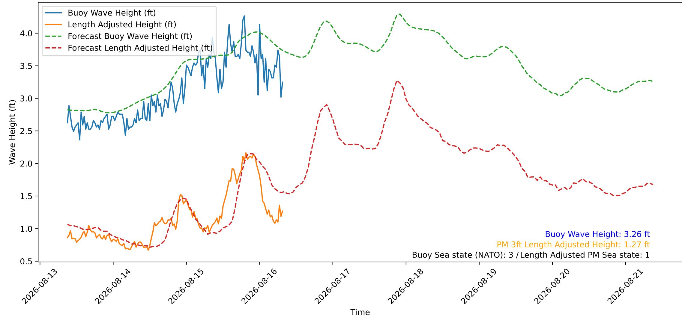
Wave Heights over Time for Green Beach at 2026-08-16 08:31:08
