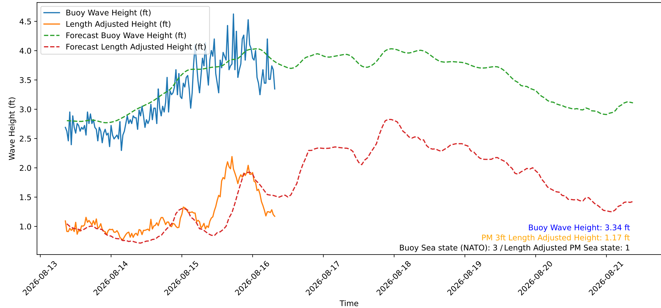
Wave Heights over Time for Oceanside Harbor at 2026-08-16 08:30:27
