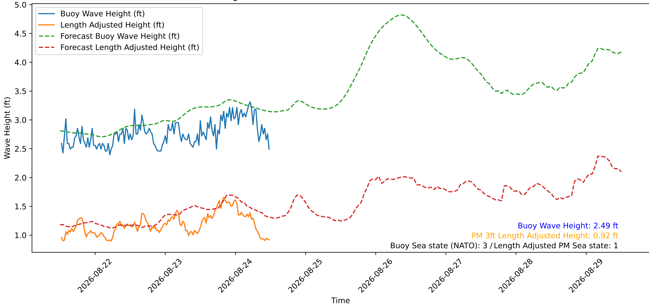
Wave Heights over Time for Green Beach at 2026-08-24 12:21:14
