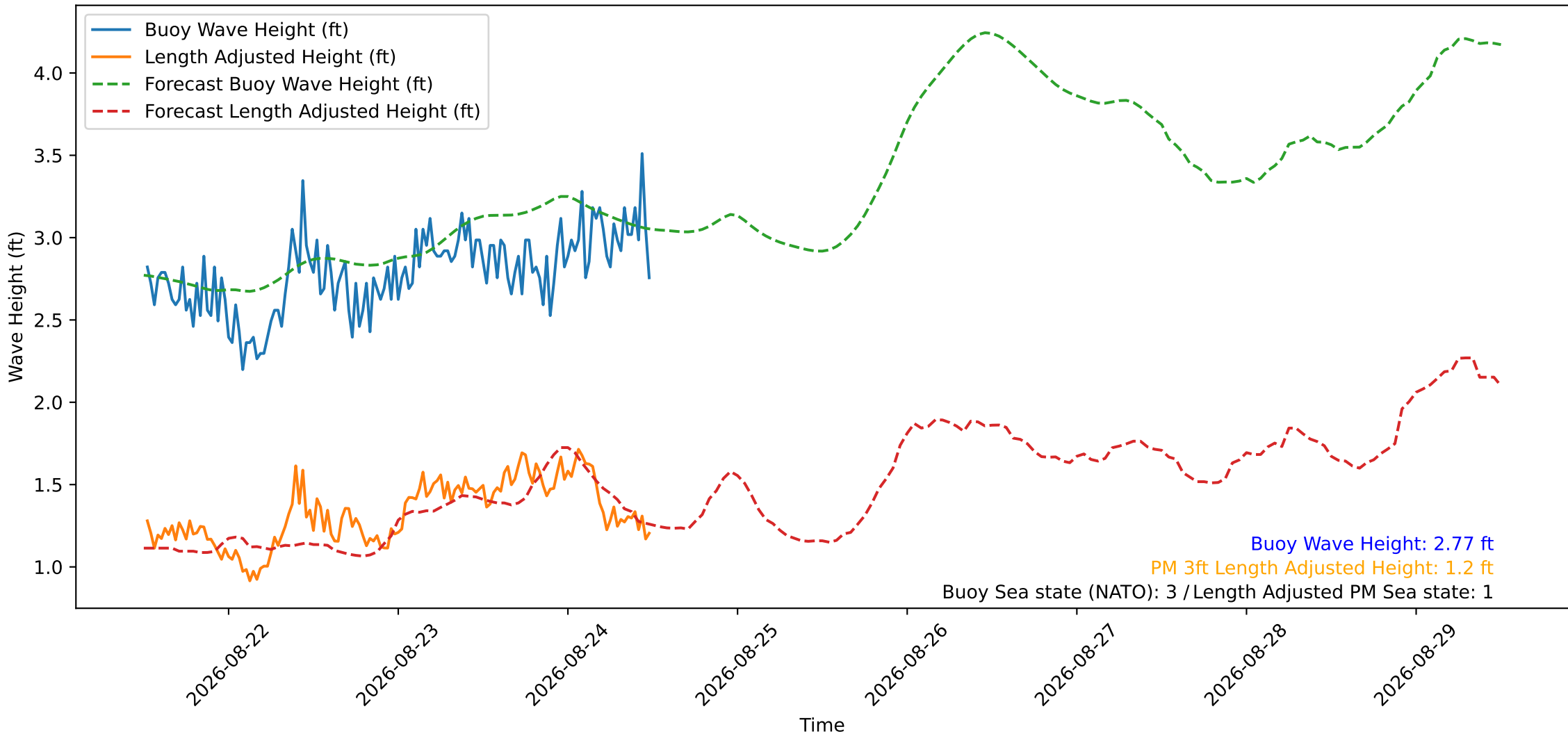
Wave Heights over Time for Oceanside Harbor at 2026-08-24 12:20:29
