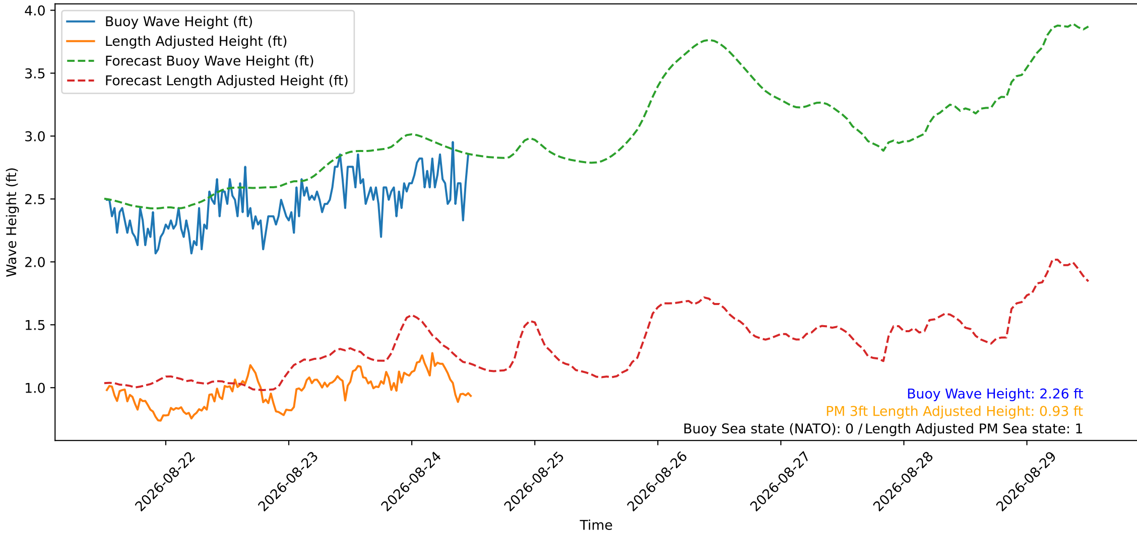
Wave Heights over Time for Red Beach at 2026-08-24 12:20:50
