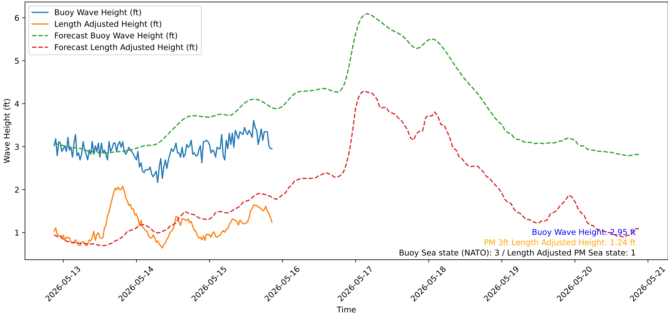
Wave Heights over Time for Oceanside Harbor at 2026-05-15 21:10:32
