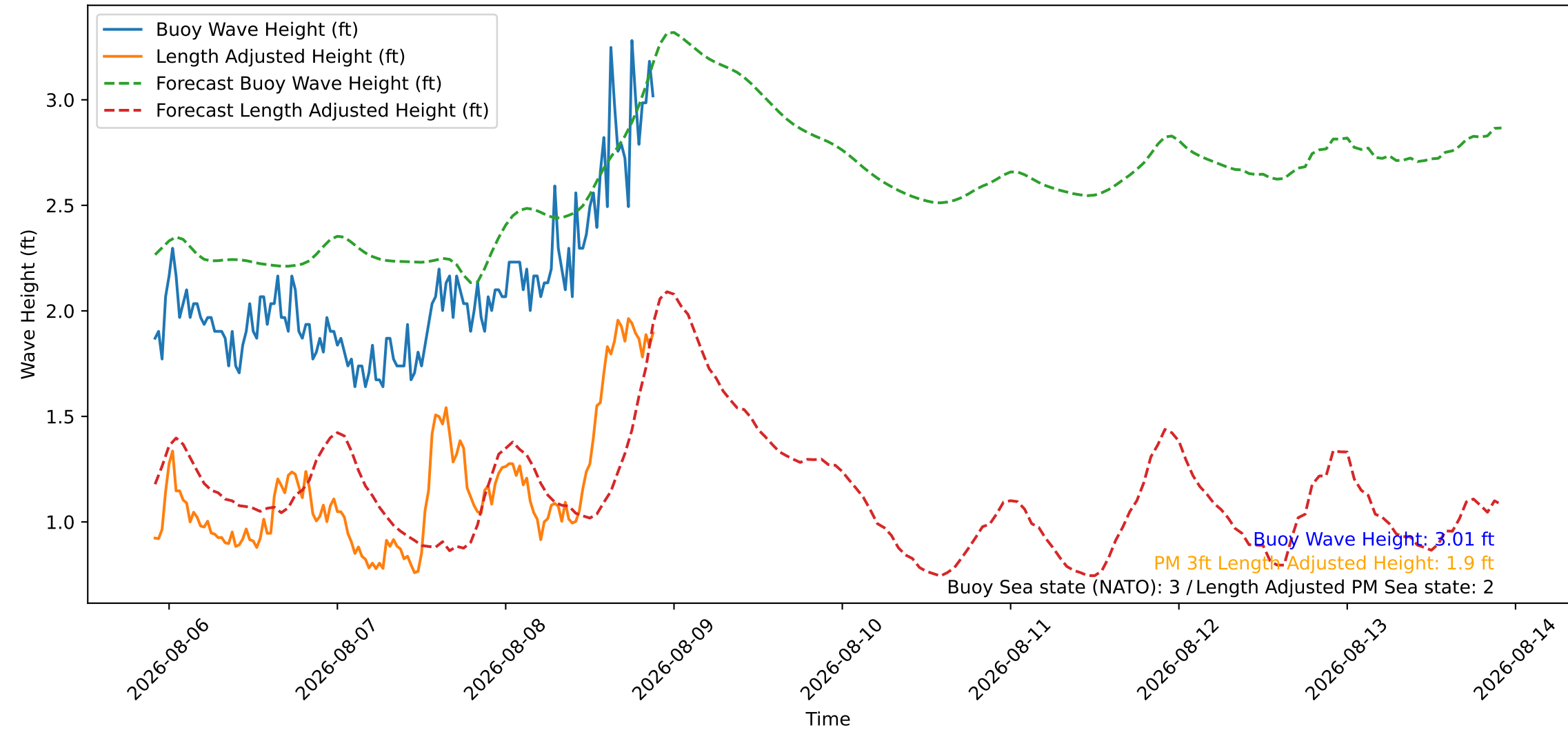
Wave Heights over Time for Oceanside Harbor at 2026-08-08 21:50:27
