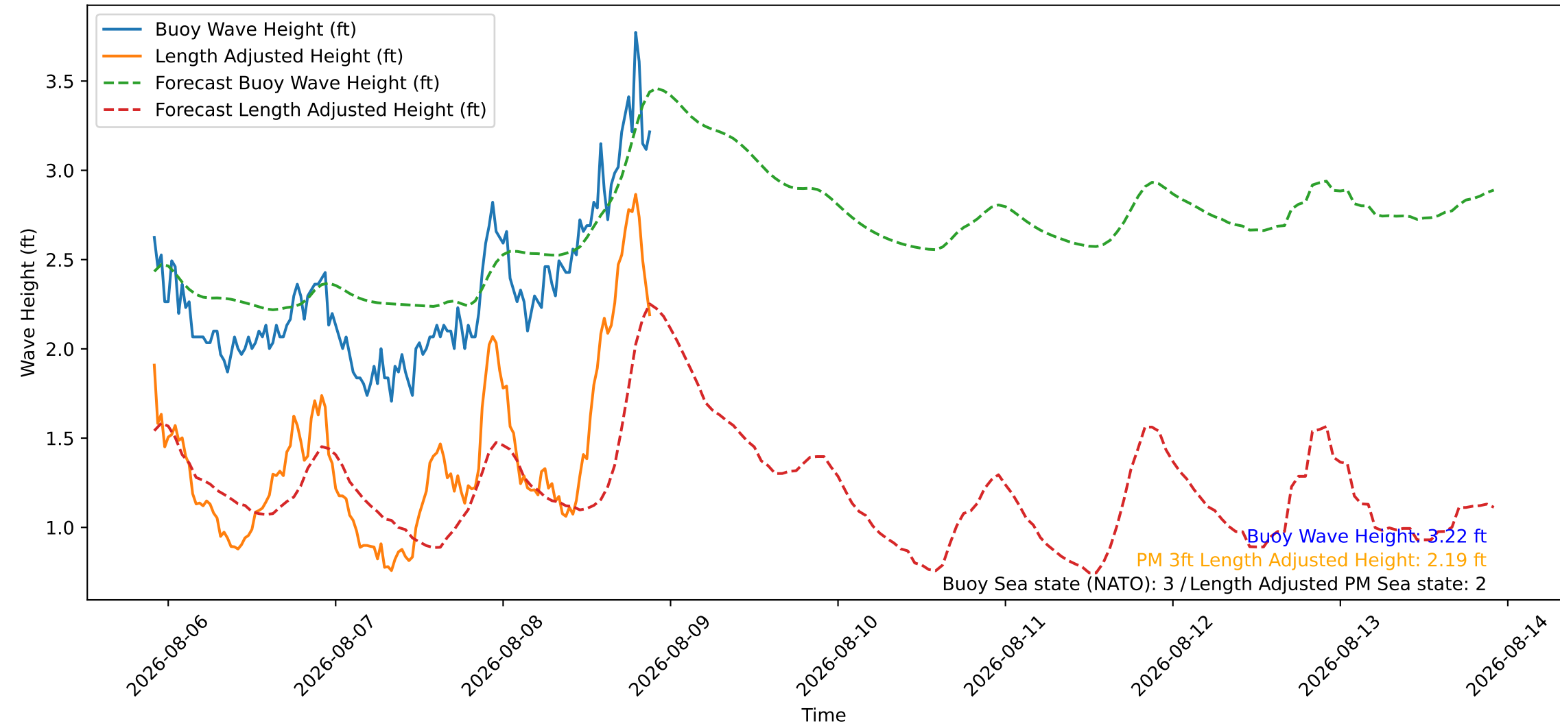
Wave Heights over Time for Green Beach at 2026-08-08 21:51:09
