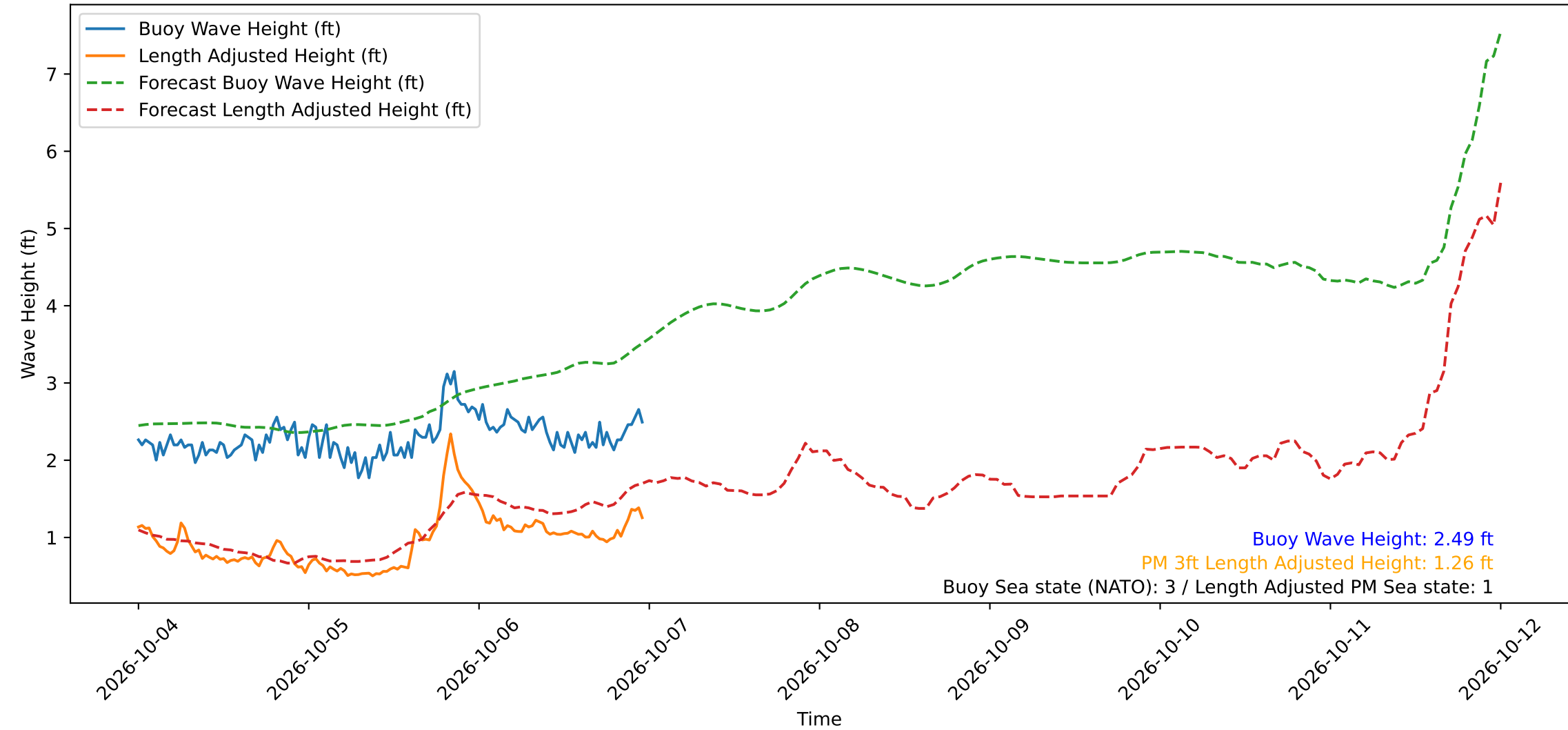
Wave Heights over Time for Green Beach at 2026-10-06 23:51:14
