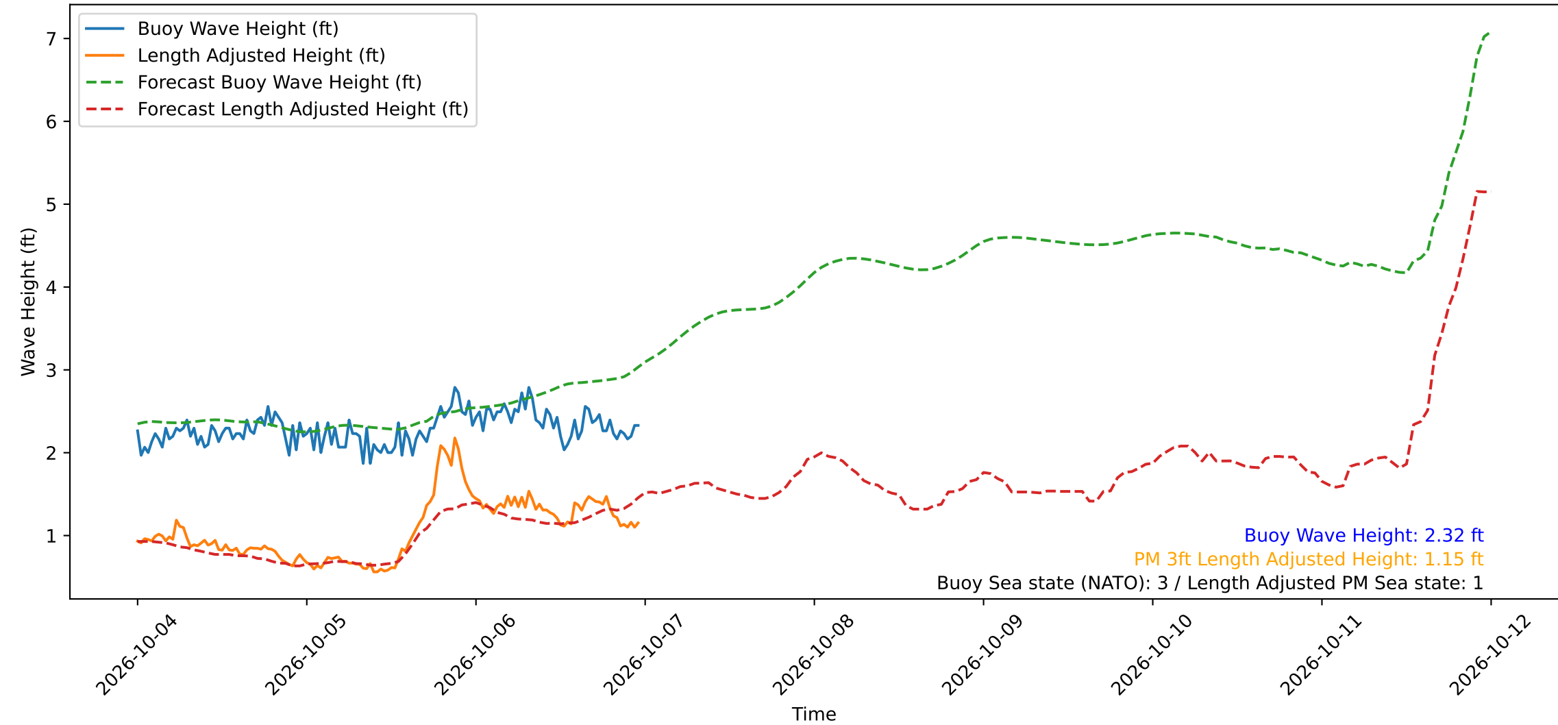
Wave Heights over Time for Oceanside Harbor at 2026-10-06 23:50:29
