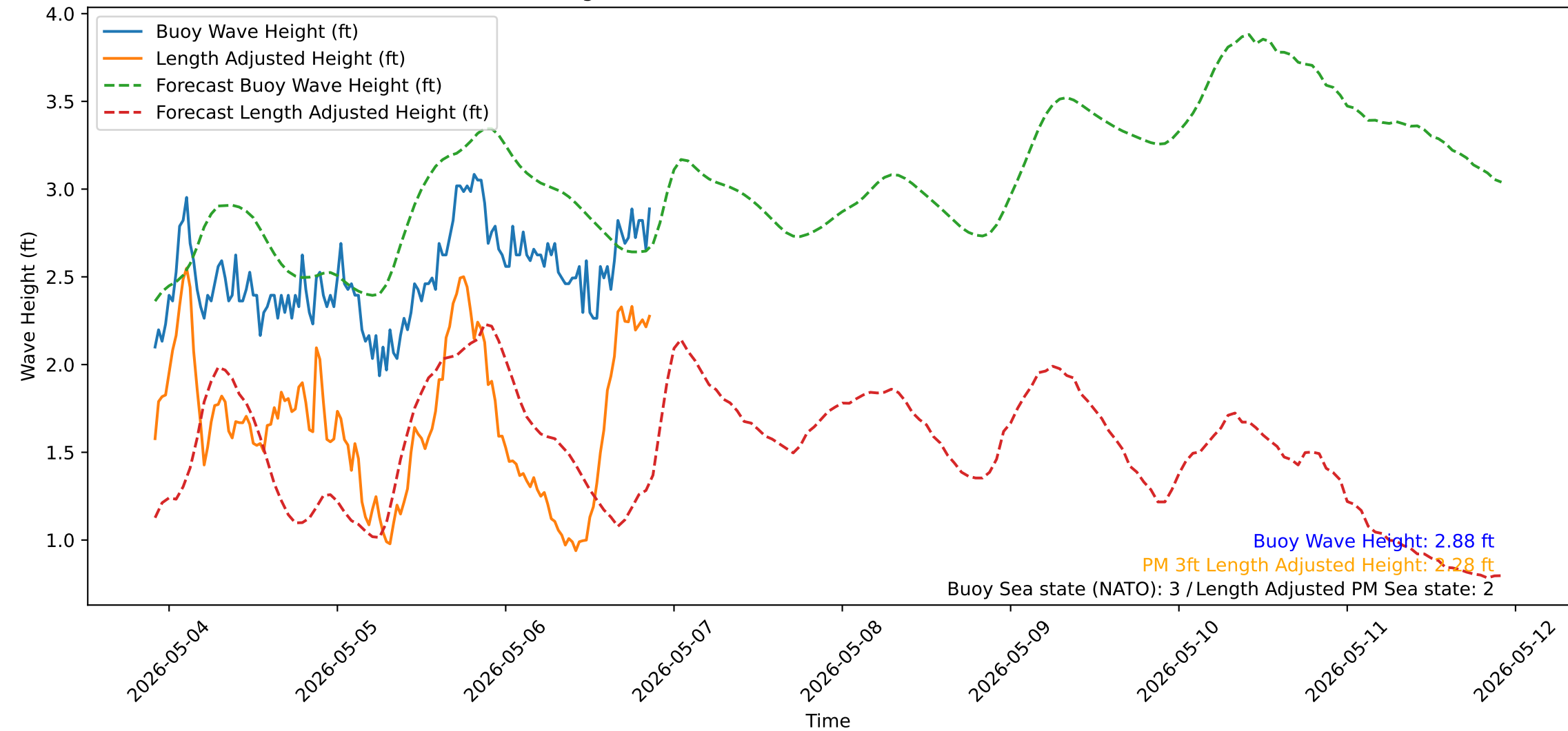
Wave Heights over Time for Red Beach at 2026-05-06 21:50:52
