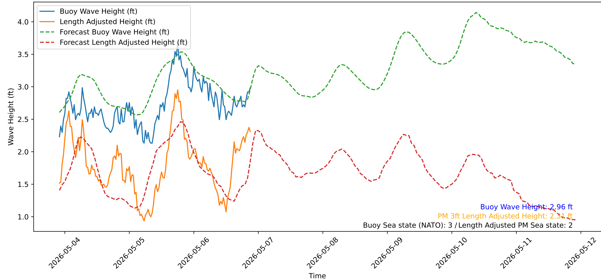
Wave Heights over Time for Green Beach at 2026-05-06 21:51:14
