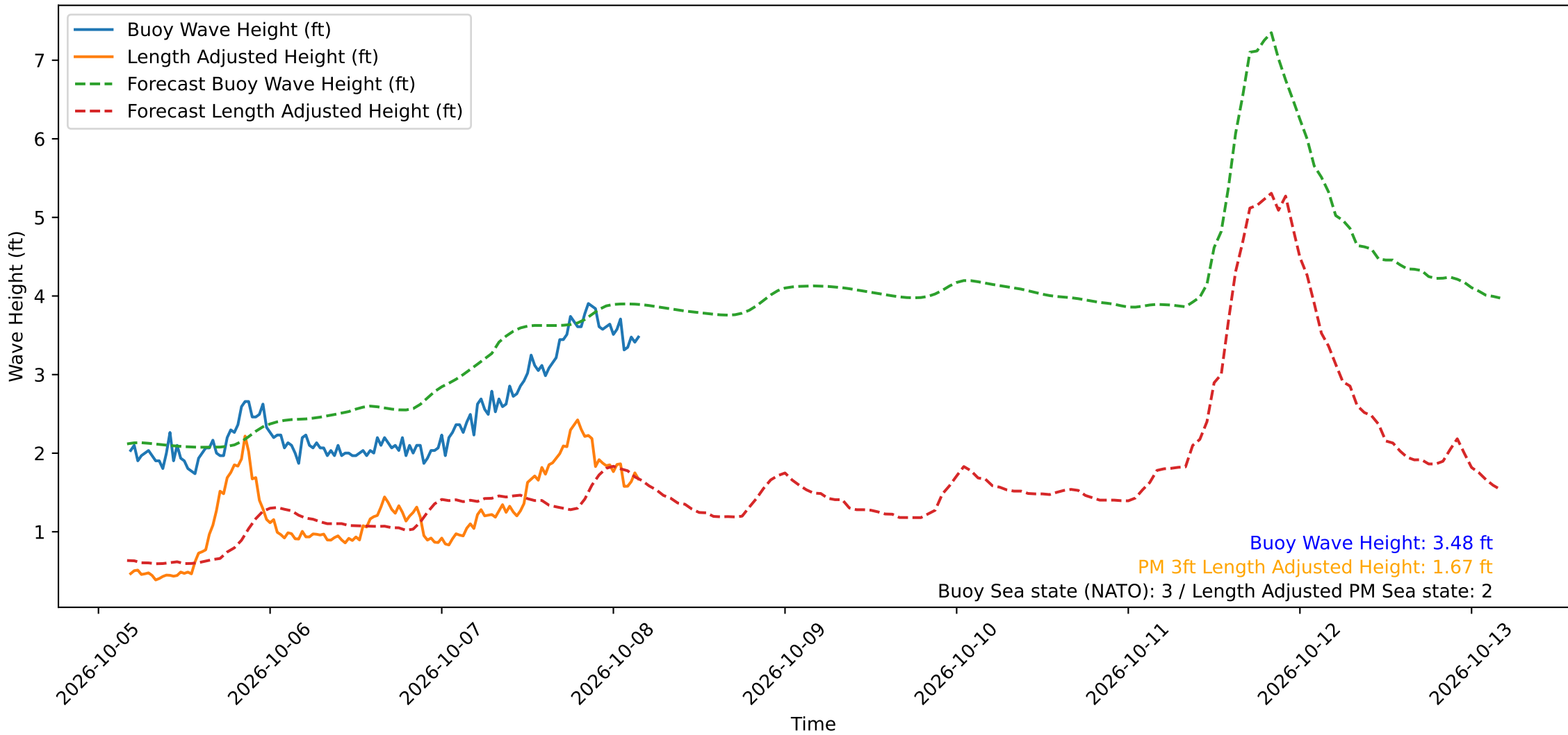
Wave Heights over Time for Red Beach at 2026-10-08 04:10:49
