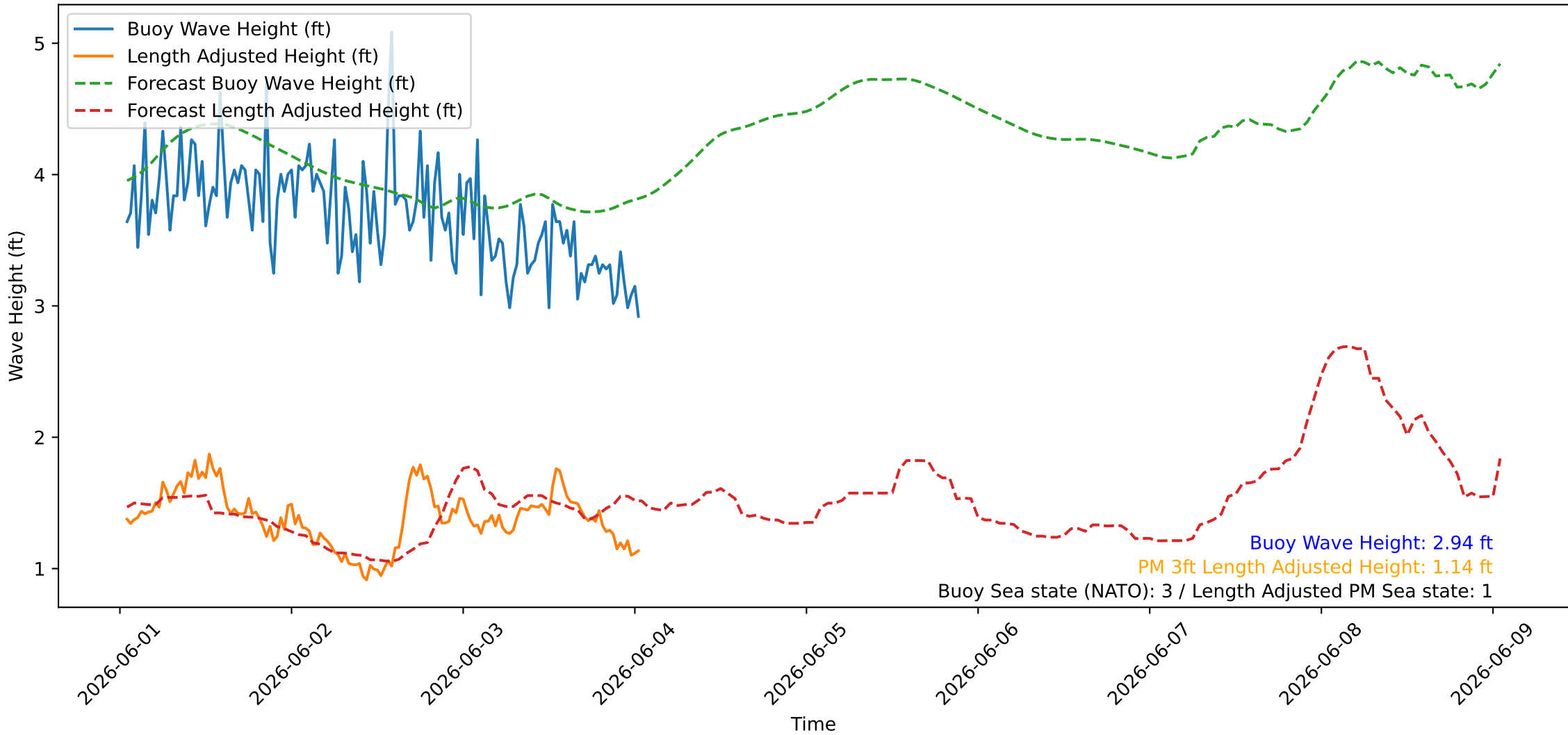
Wave Heights over Time for Oceanside Harbor at 2026-06-04 01:10:26
