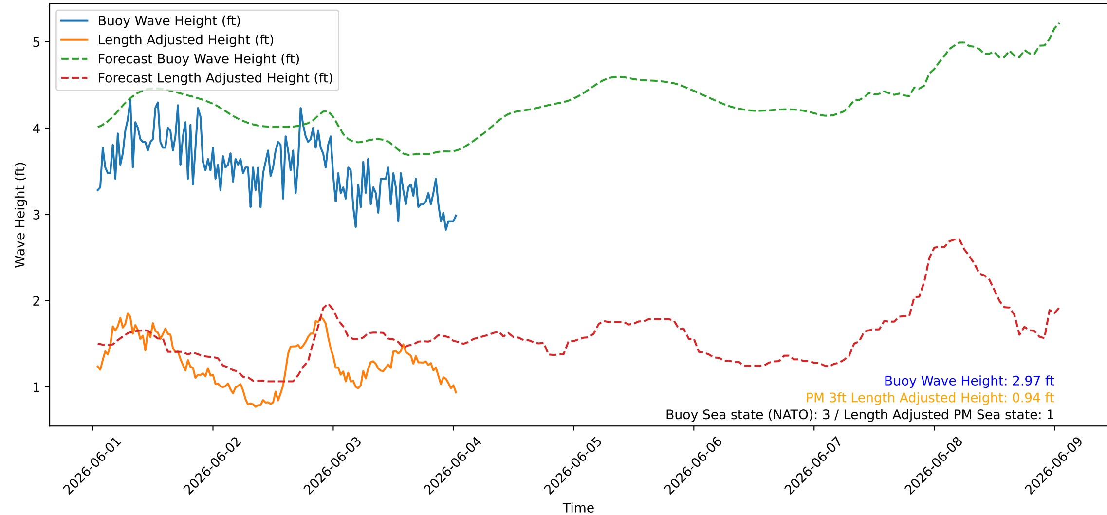
Wave Heights over Time for Green Beach at 2026-06-04 01:11:08
