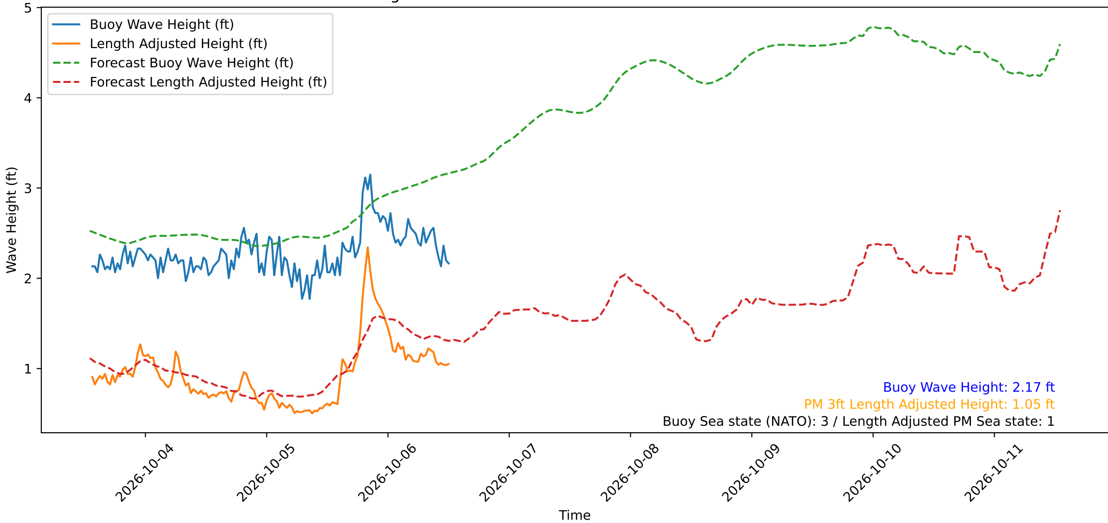
Wave Heights over Time for Green Beach at 2026-10-06 13:01:12
