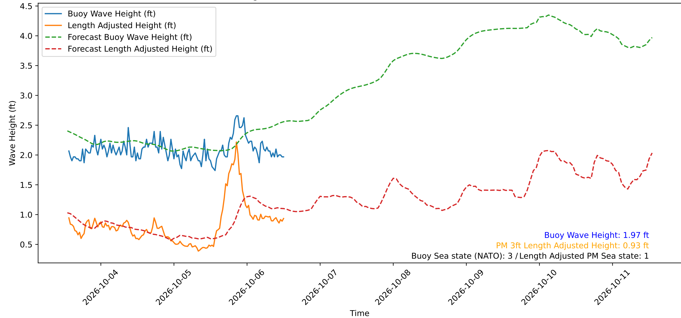
Wave Heights over Time for Red Beach at 2026-10-06 13:00:49
