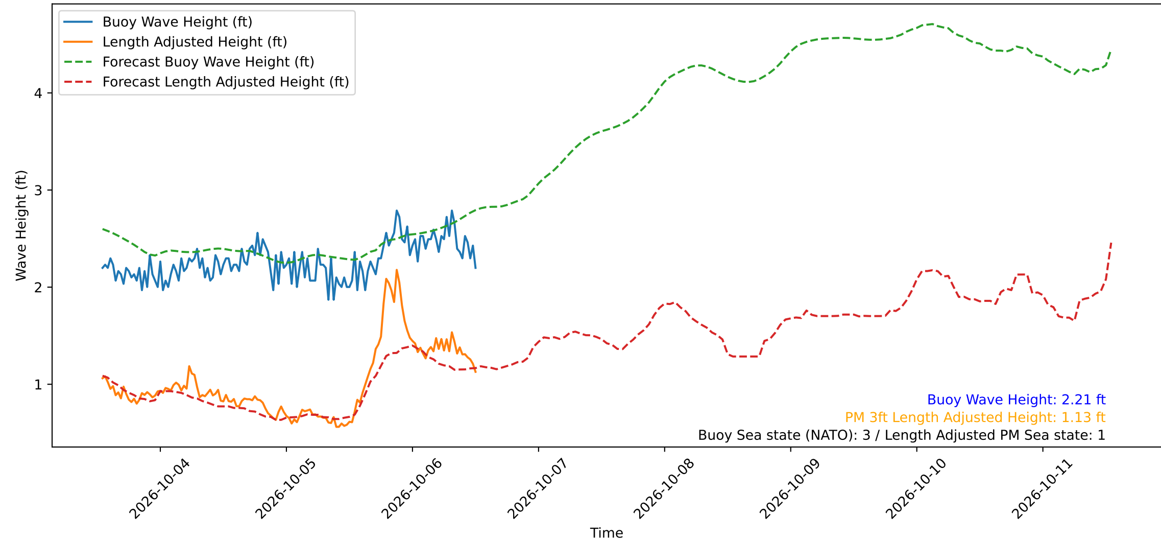
Wave Heights over Time for Oceanside Harbor at 2026-10-06 13:00:30
