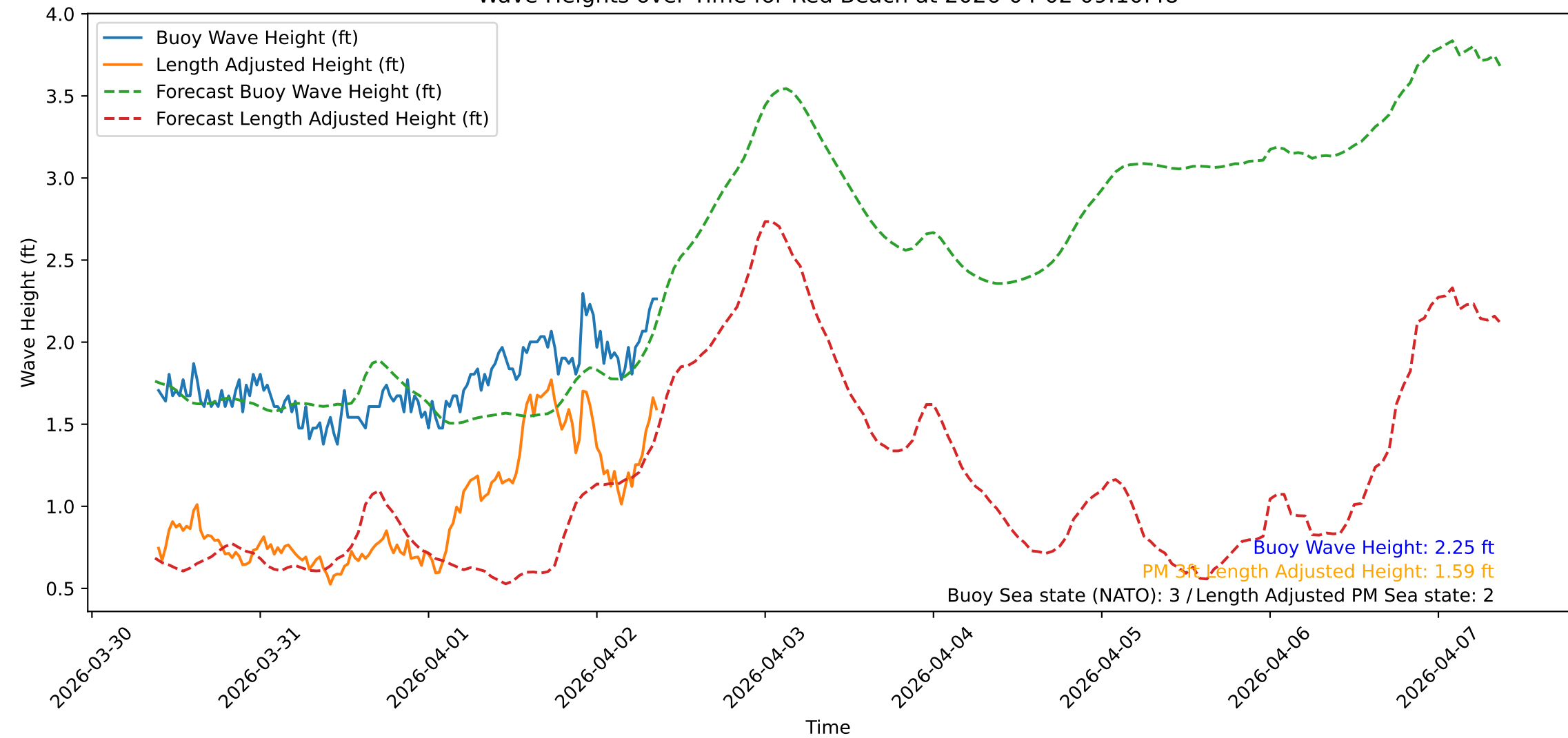
Wave Heights over Time for Red Beach at 2026-04-02 09:10:48
