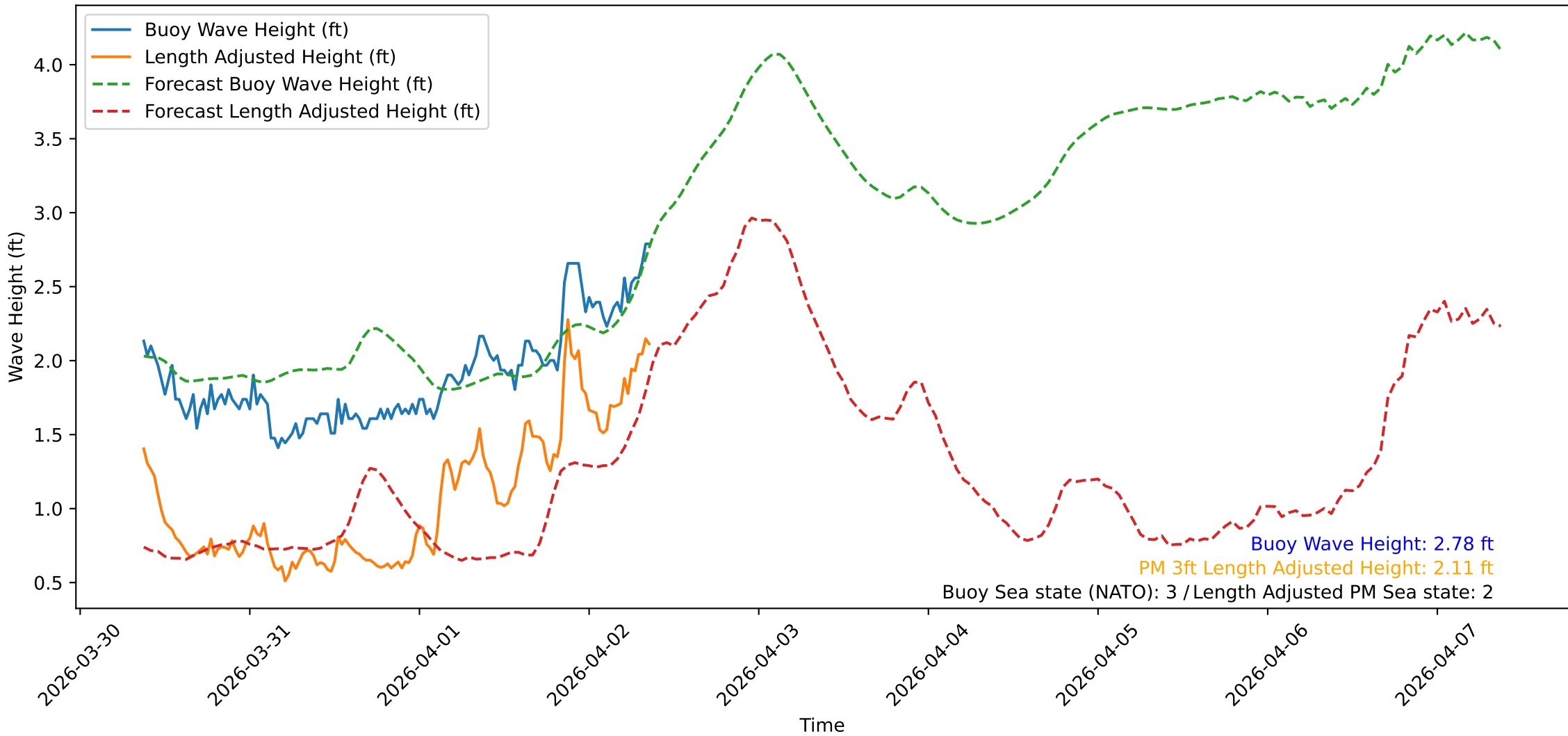
Wave Heights over Time for Green Beach at 2026-04-02 09:11:11
