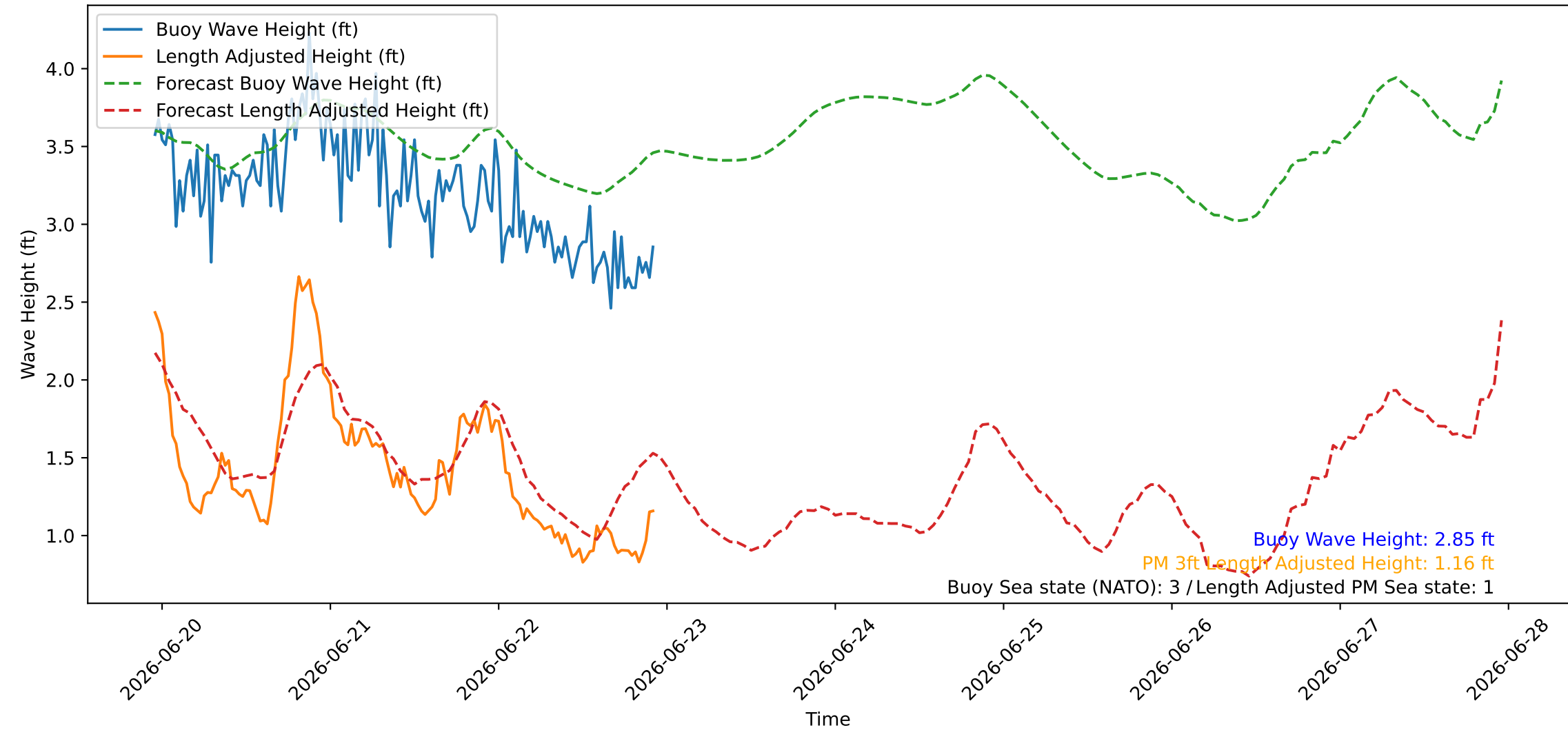
Wave Heights over Time for Green Beach at 2026-06-22 23:01:09
