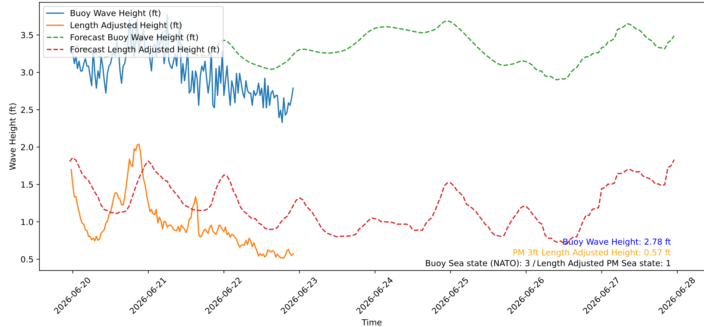
Wave Heights over Time for Red Beach at 2026-06-22 23:00:46
