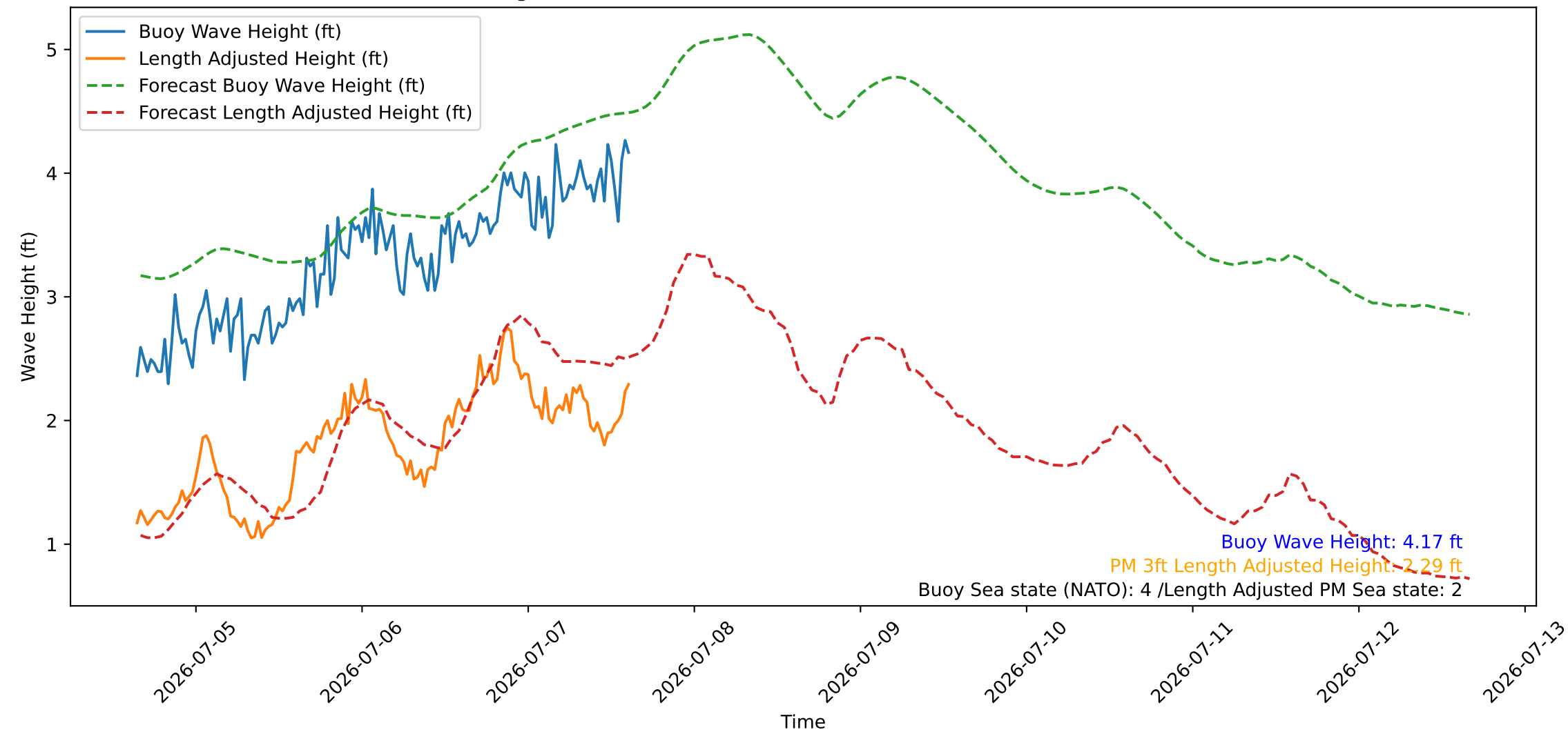
Wave Heights over Time for Oceanside Harbor at 2026-07-07 15:30:26
