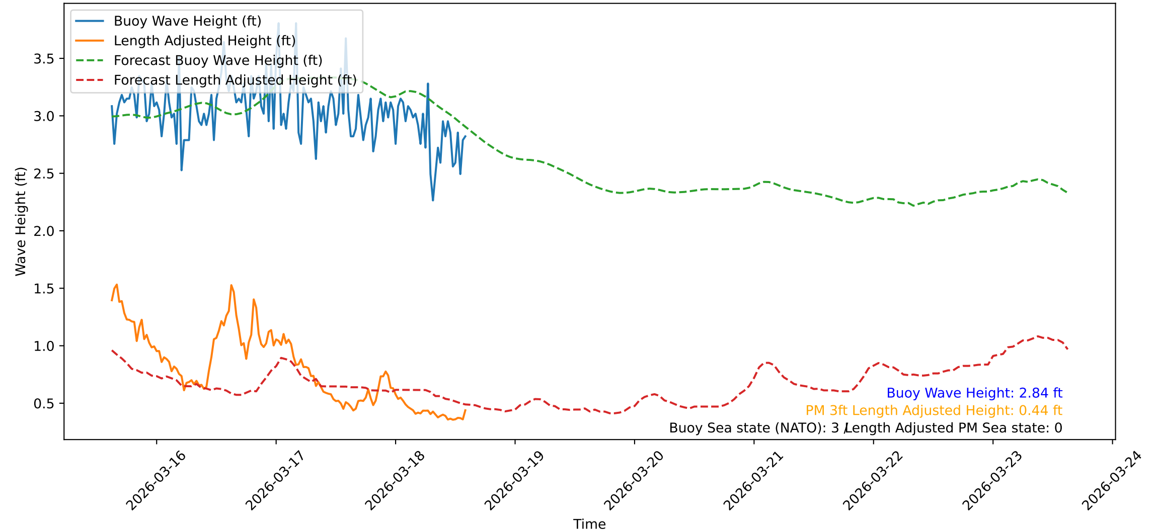
Wave Heights over Time for Red Beach at 2026-03-18 14:40:47
