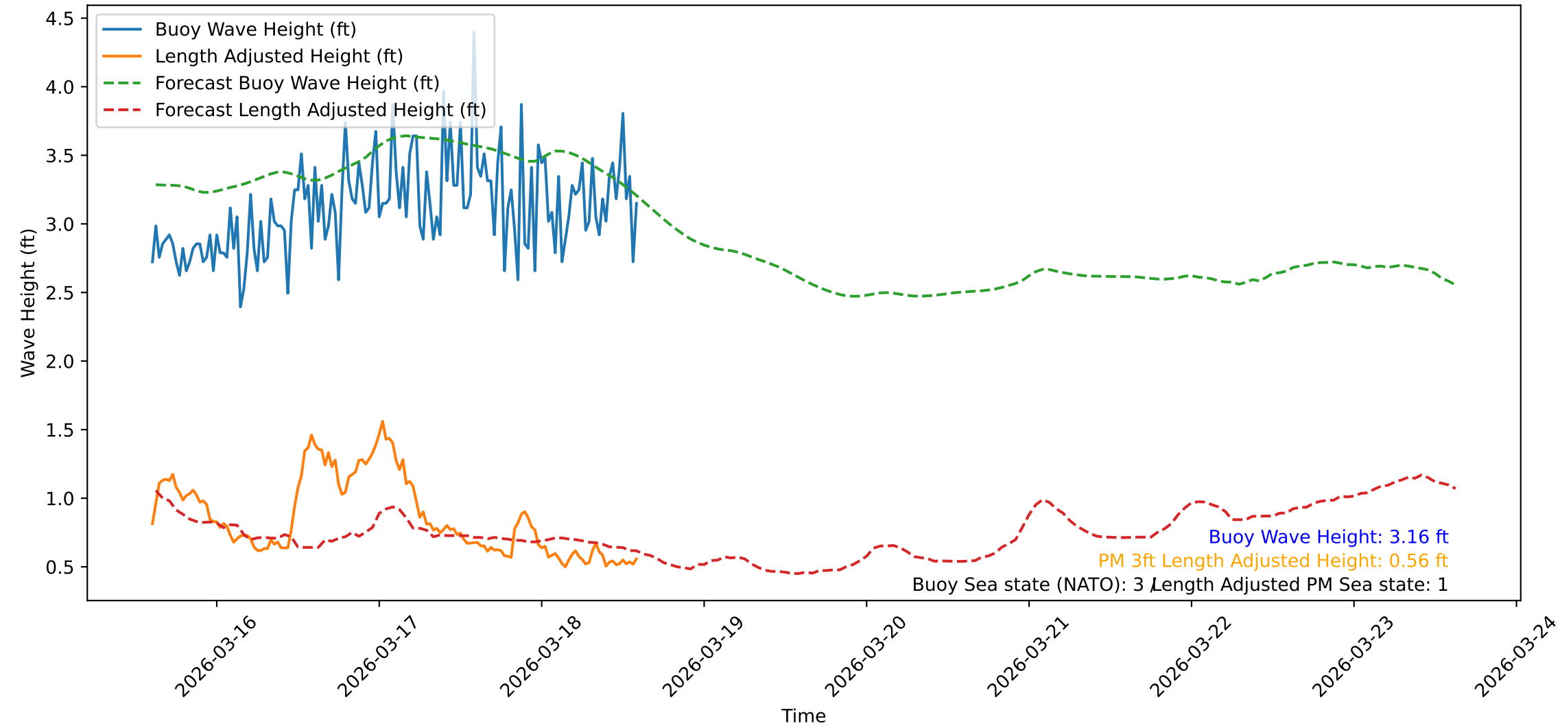
Wave Heights over Time for Oceanside Harbor at 2026-03-18 14:40:31
