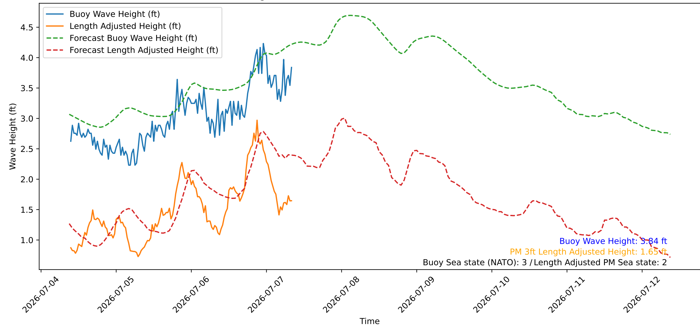
Wave Heights over Time for Red Beach at 2026-07-07 09:10:46
