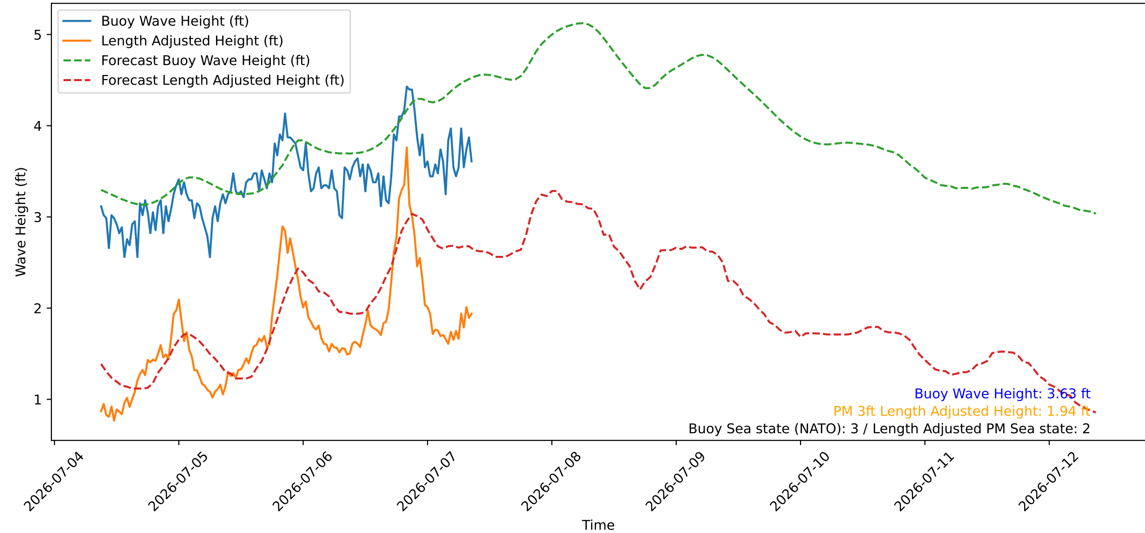
Wave Heights over Time for Green Beach at 2026-07-07 09:11:08
