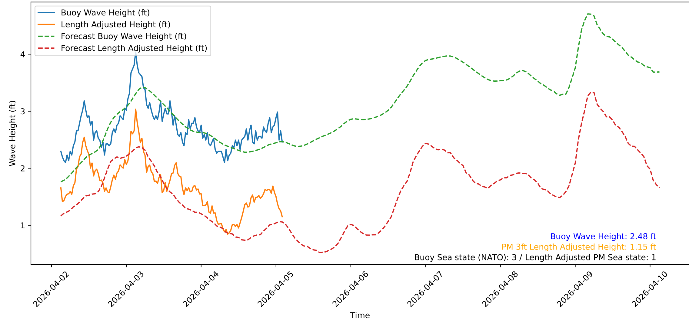
Wave Heights over Time for Oceanside Harbor at 2026-04-05 02:50:31
