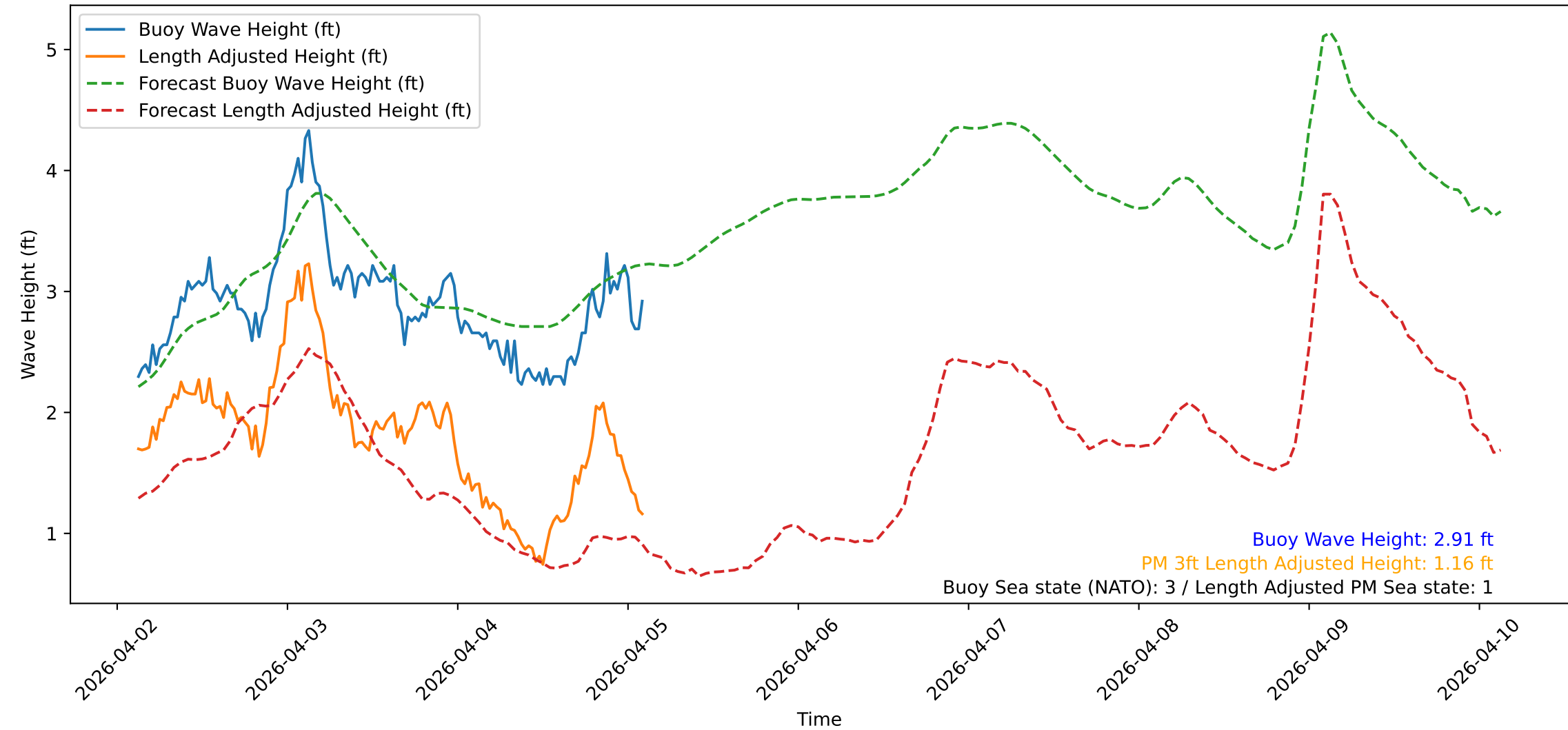
Wave Heights over Time for Green Beach at 2026-04-05 02:51:10
