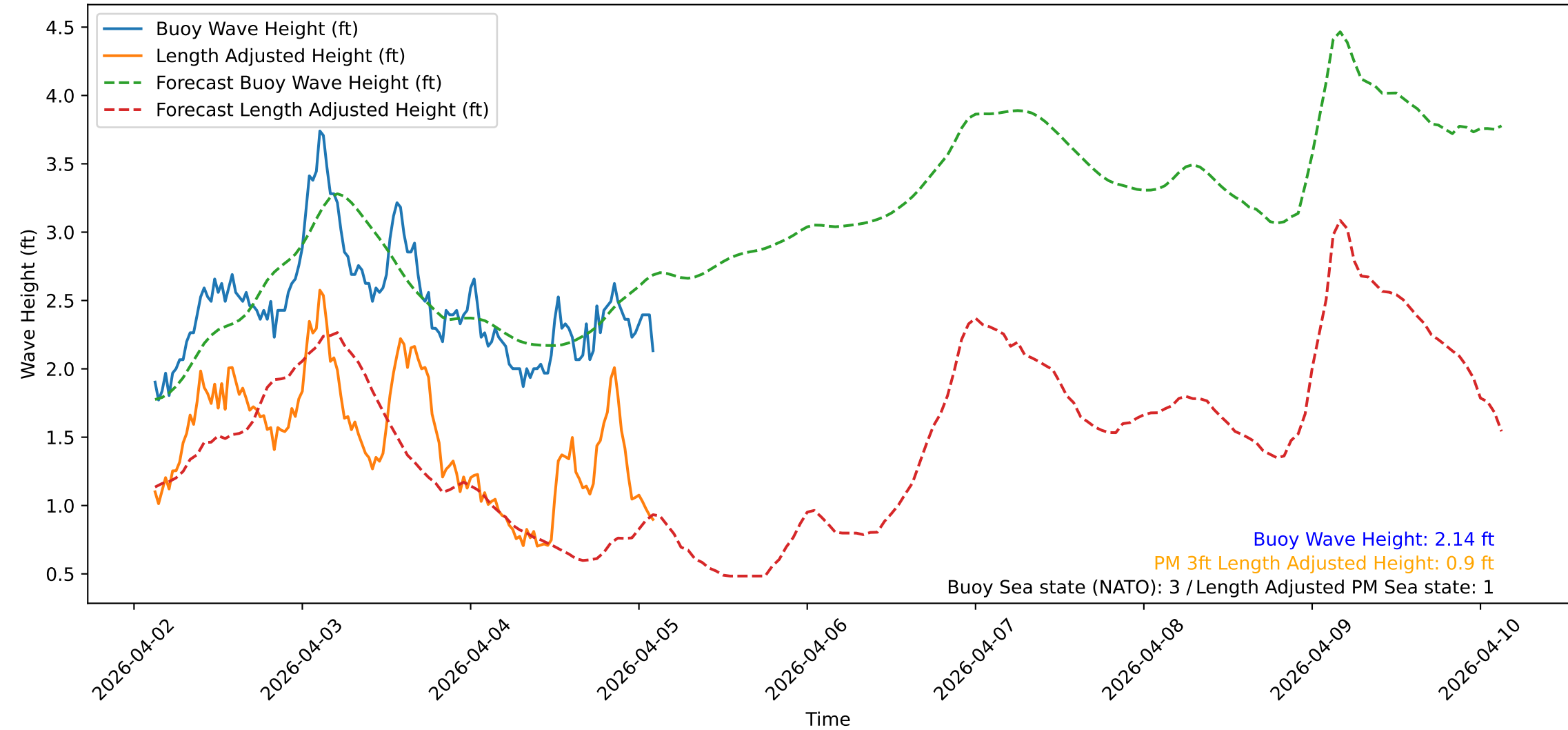
Wave Heights over Time for Red Beach at 2026-04-05 02:50:47
