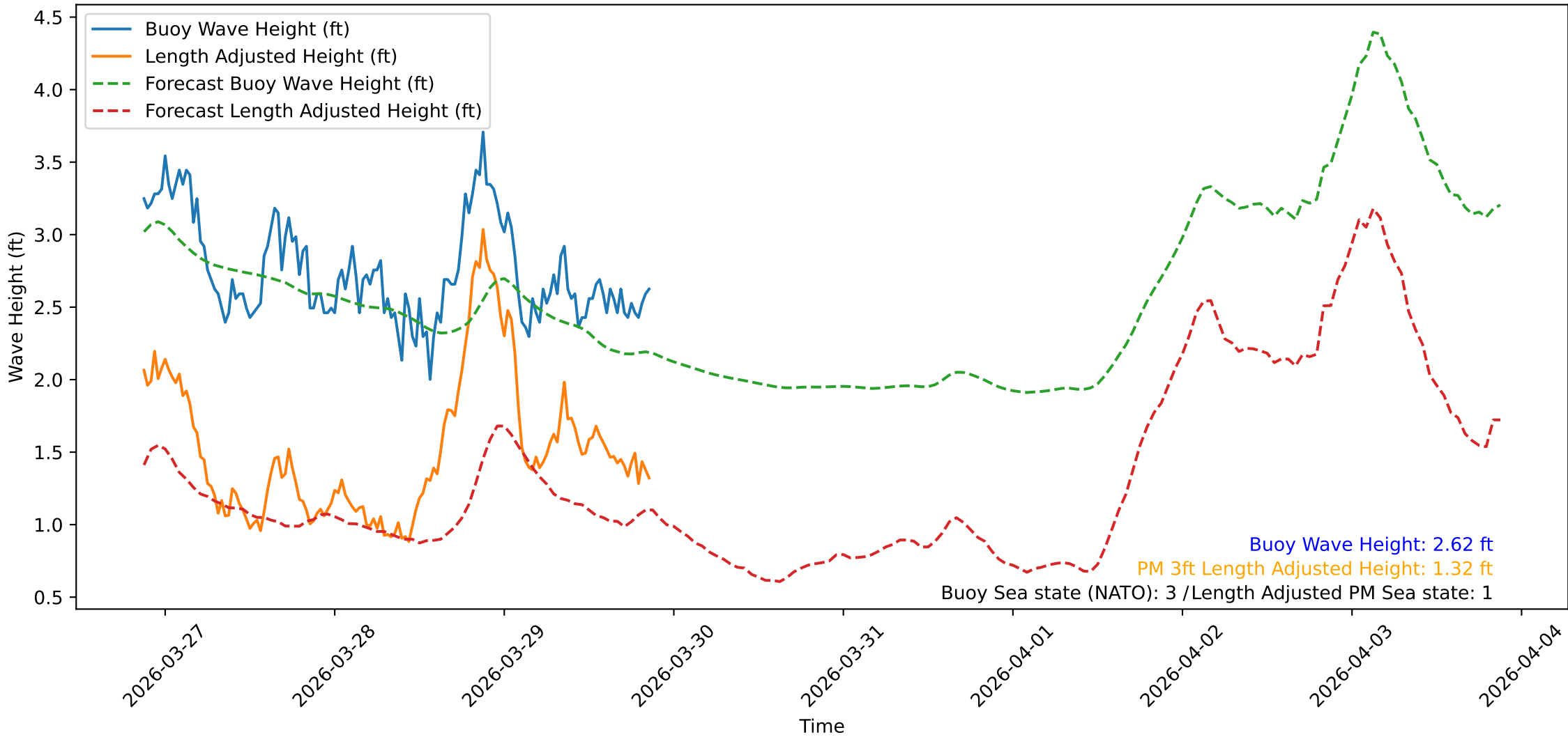
Wave Heights over Time for Green Beach at 2026-03-29 21:11:10
