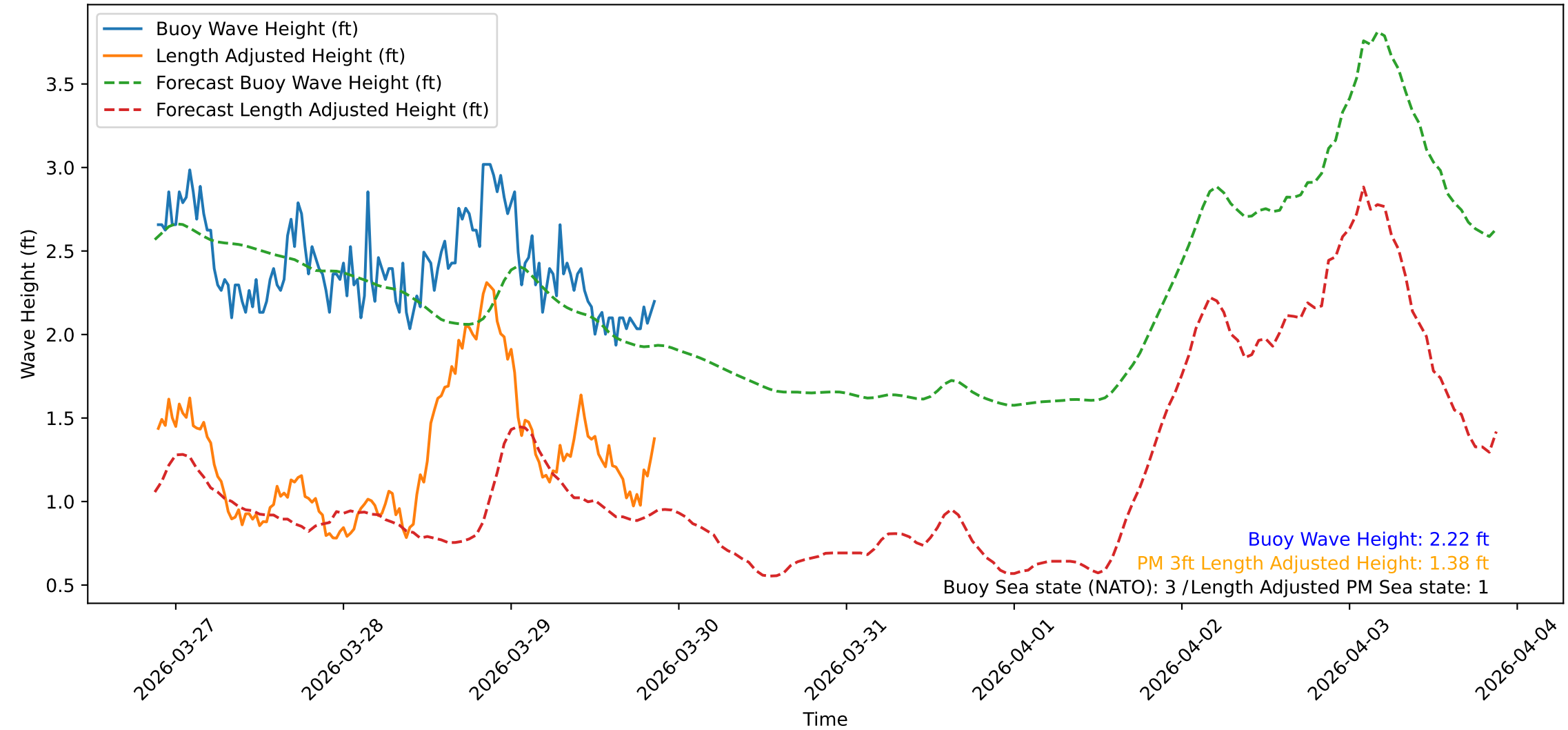
Wave Heights over Time for Red Beach at 2026-03-29 21:10:47
