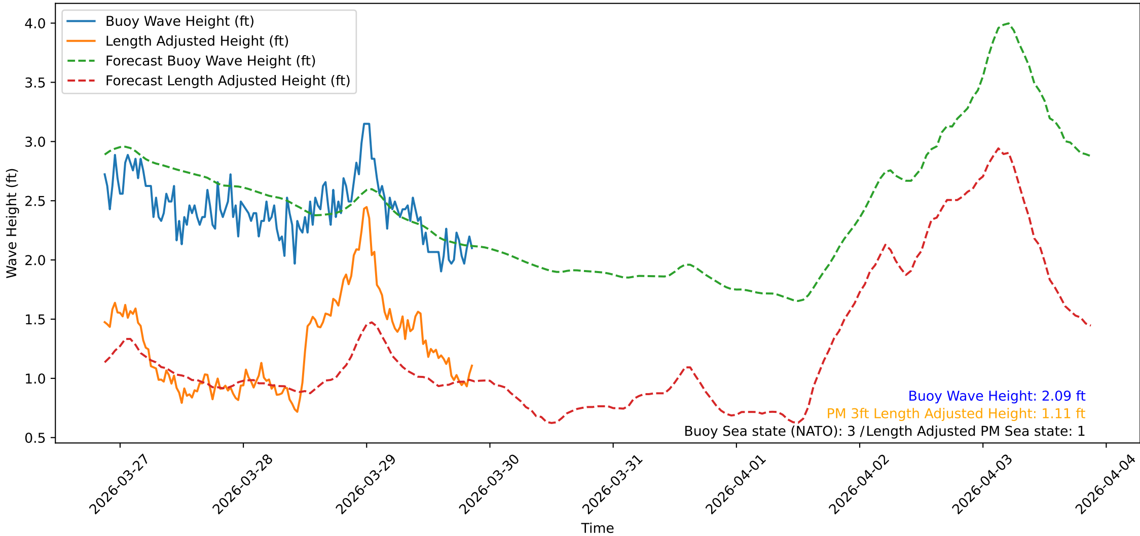
Wave Heights over Time for Oceanside Harbor at 2026-03-29 21:10:32
