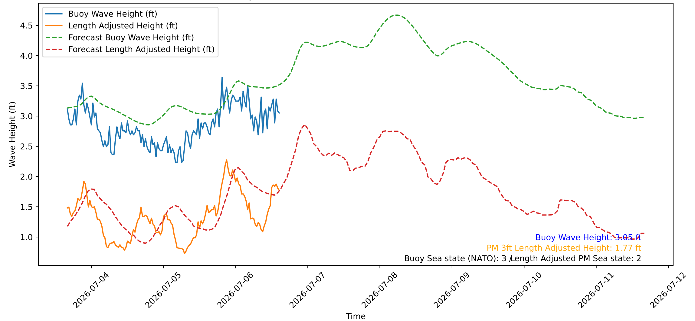
Wave Heights over Time for Red Beach at 2026-07-06 15:30:46
