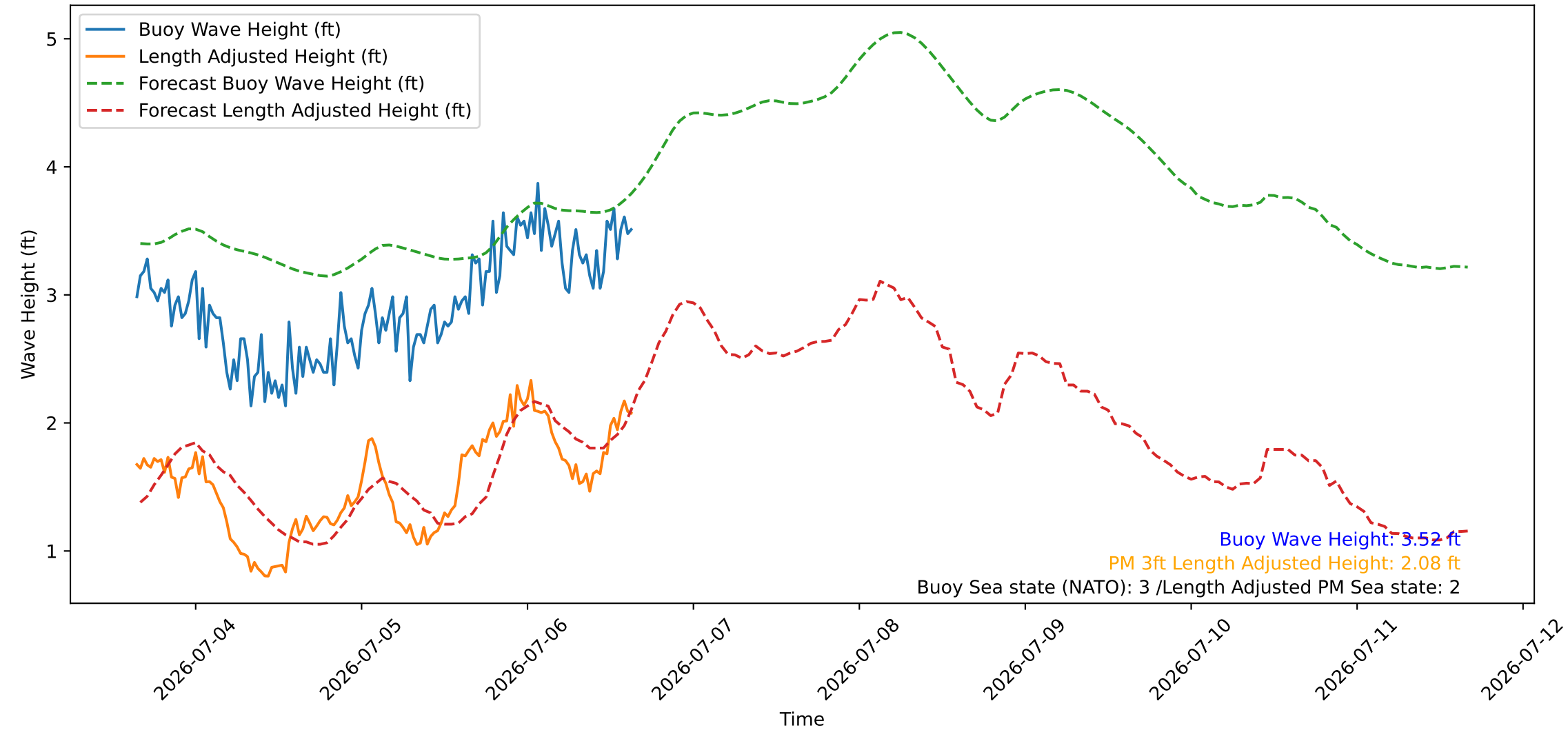
Wave Heights over Time for Oceanside Harbor at 2026-07-06 15:30:26
