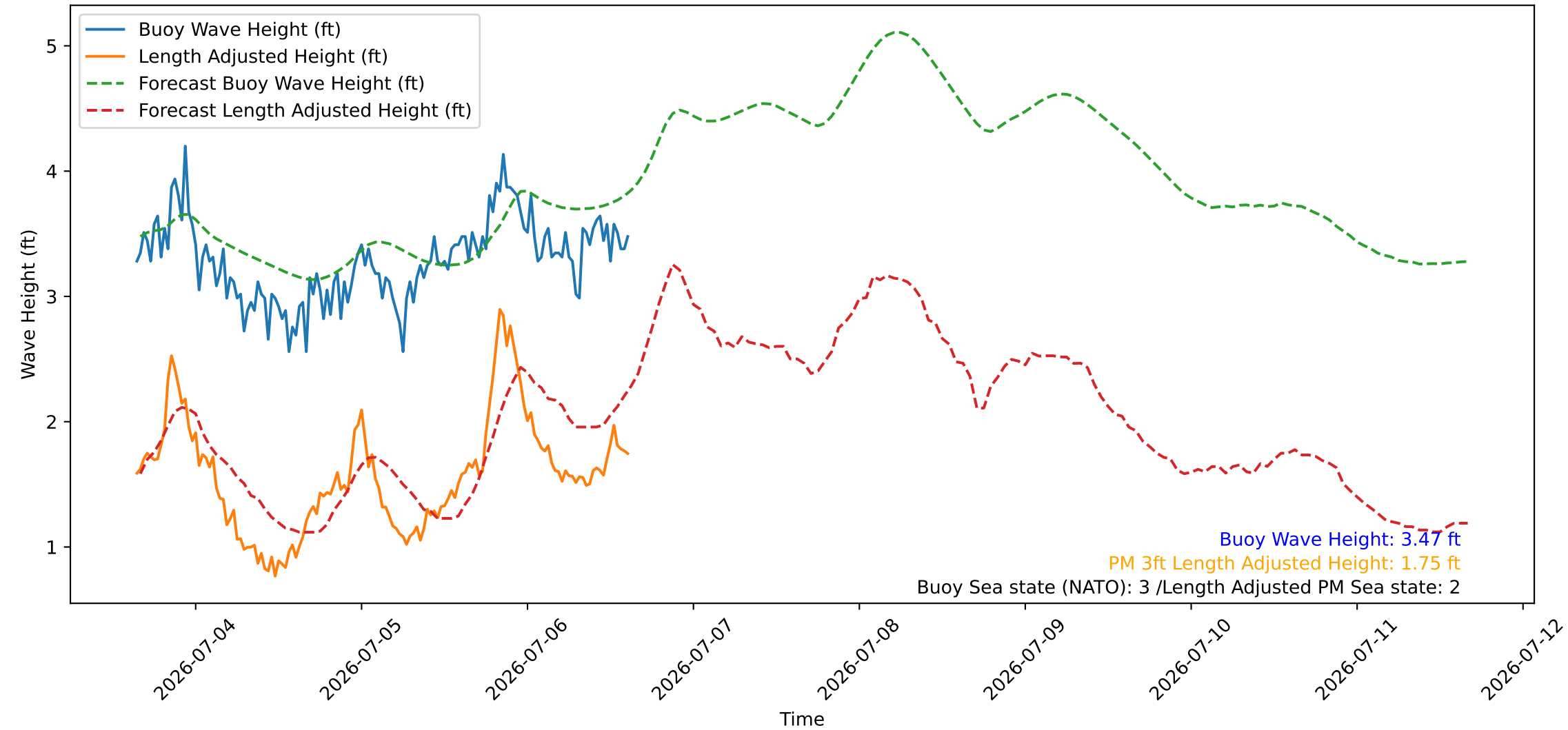
Wave Heights over Time for Green Beach at 2026-07-06 15:31:09
