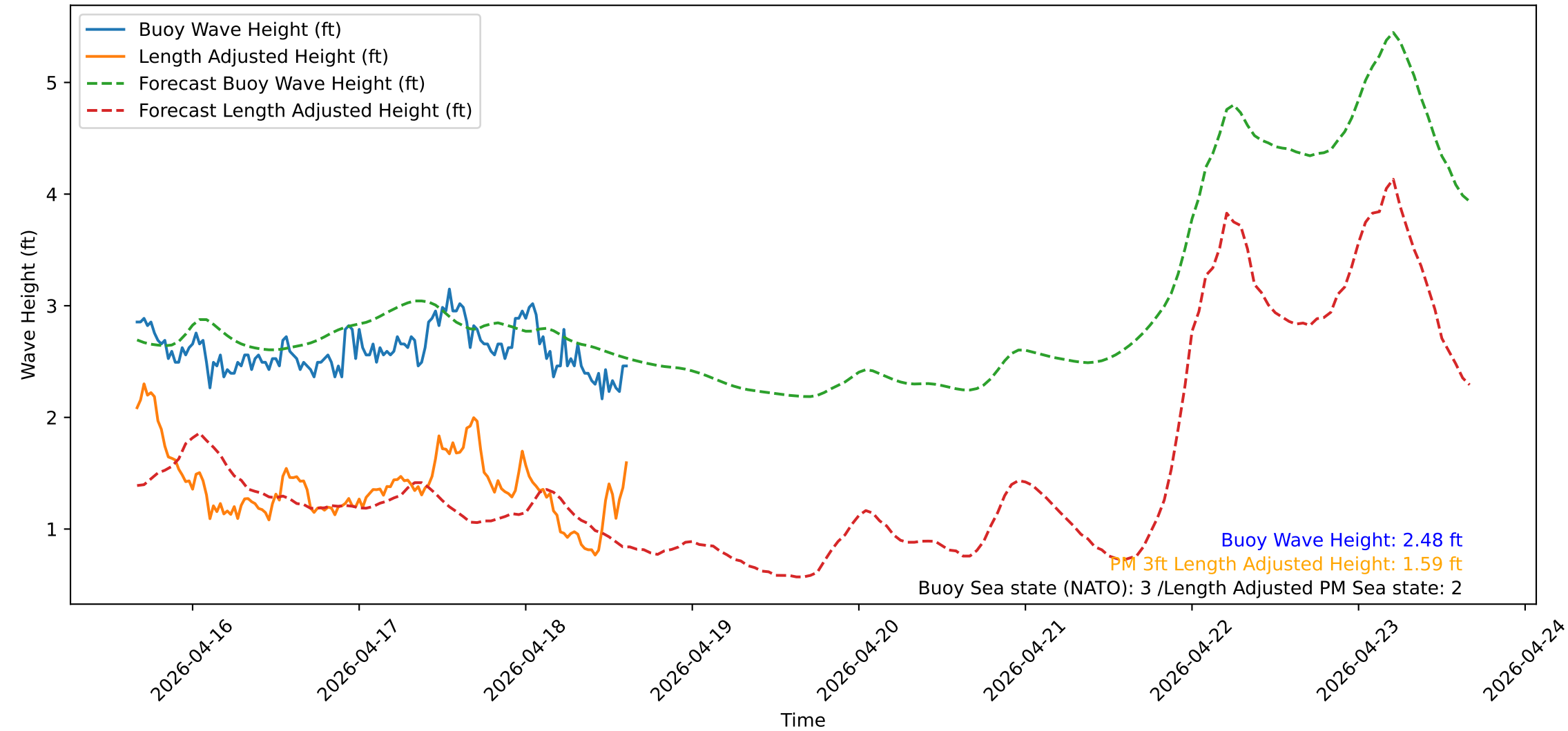
Wave Heights over Time for Red Beach at 2026-04-18 15:30:50
