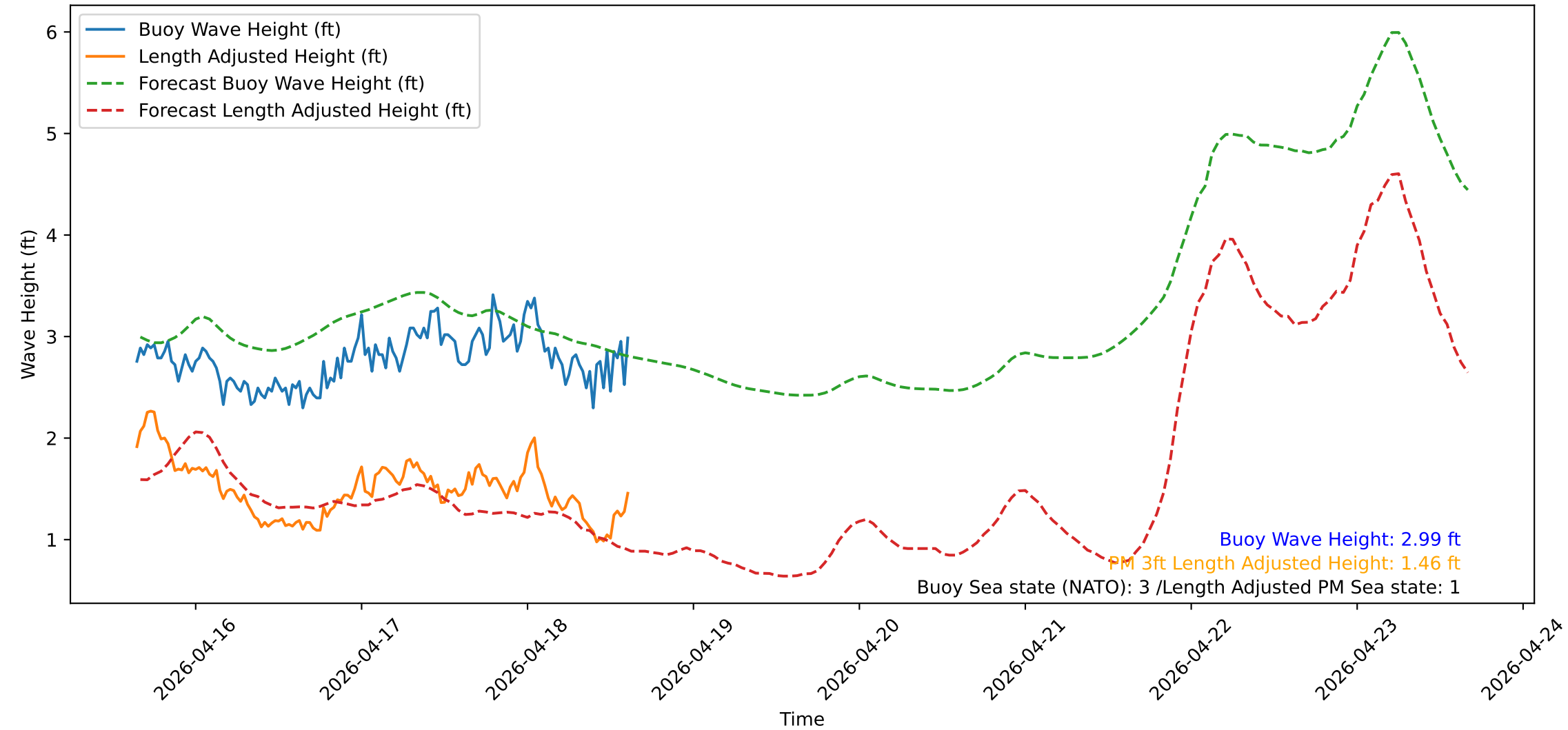
Wave Heights over Time for Oceanside Harbor at 2026-04-18 15:30:32
