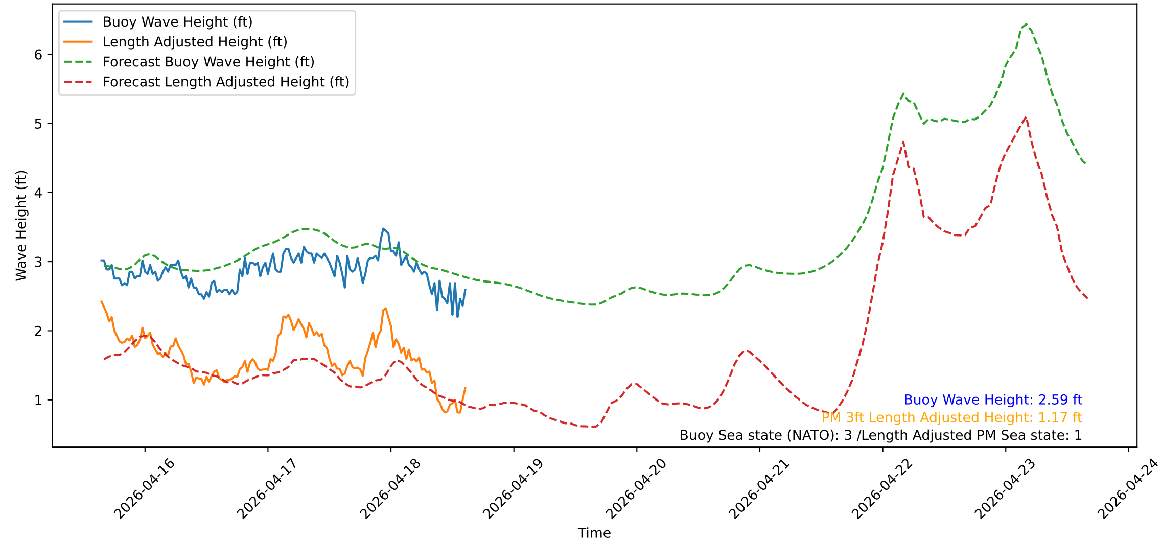
Wave Heights over Time for Green Beach at 2026-04-18 15:31:12
