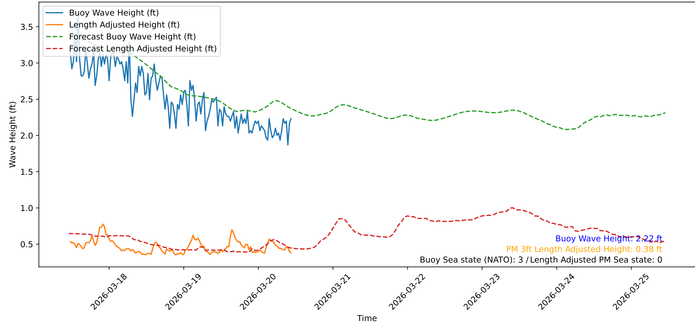
Wave Heights over Time for Red Beach at 2026-03-20 11:10:47
