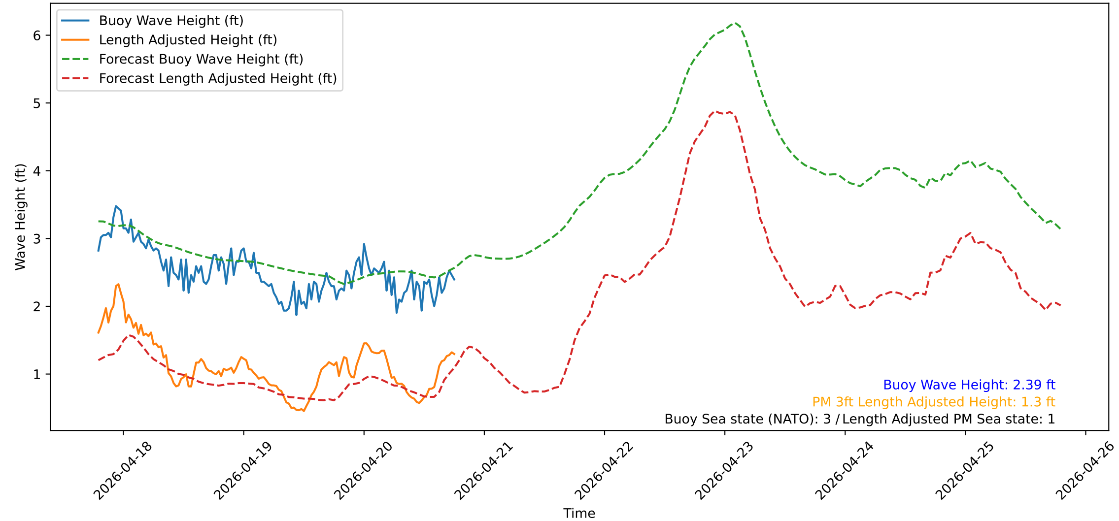
Wave Heights over Time for Green Beach at 2026-04-20 19:01:13
