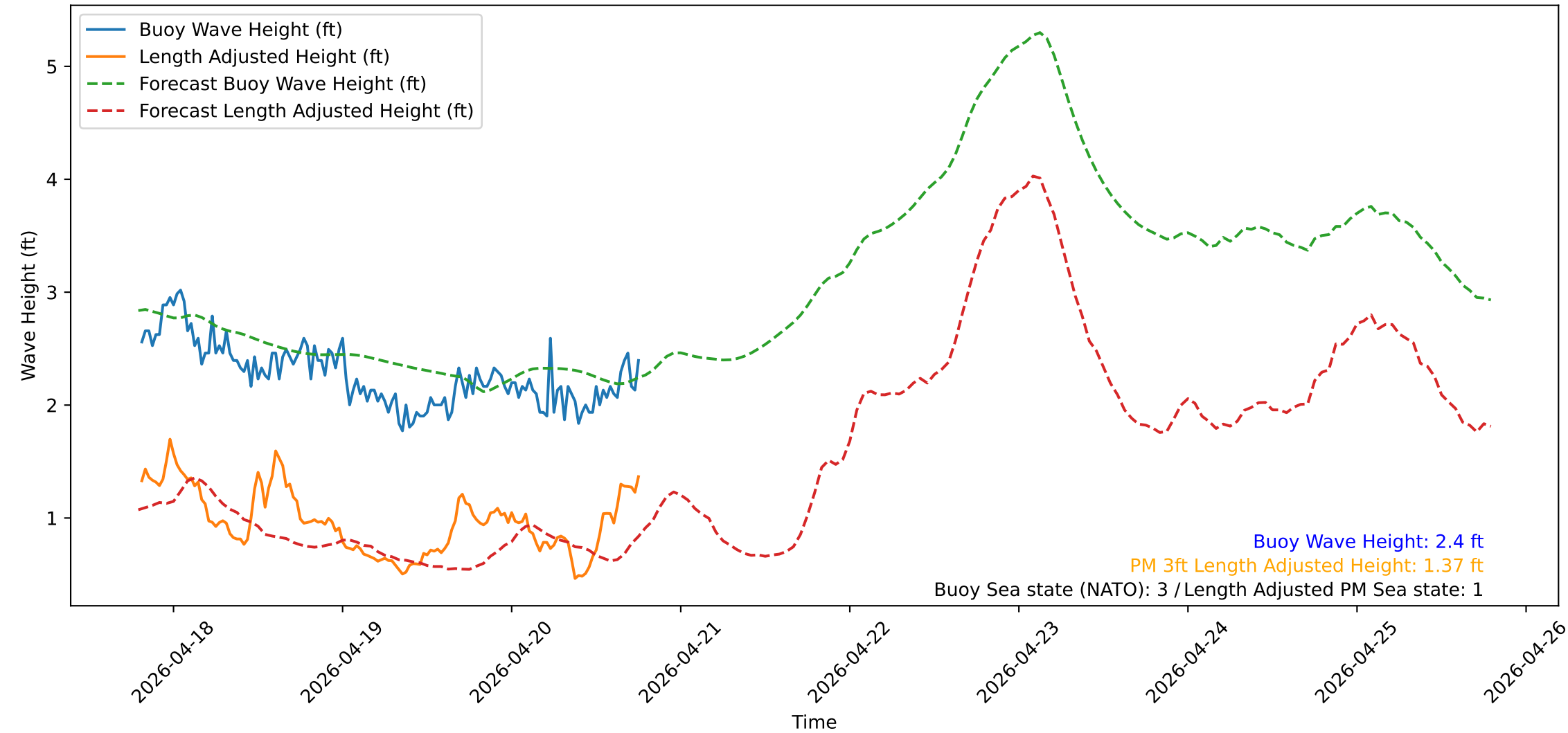
Wave Heights over Time for Red Beach at 2026-04-20 19:00:51
