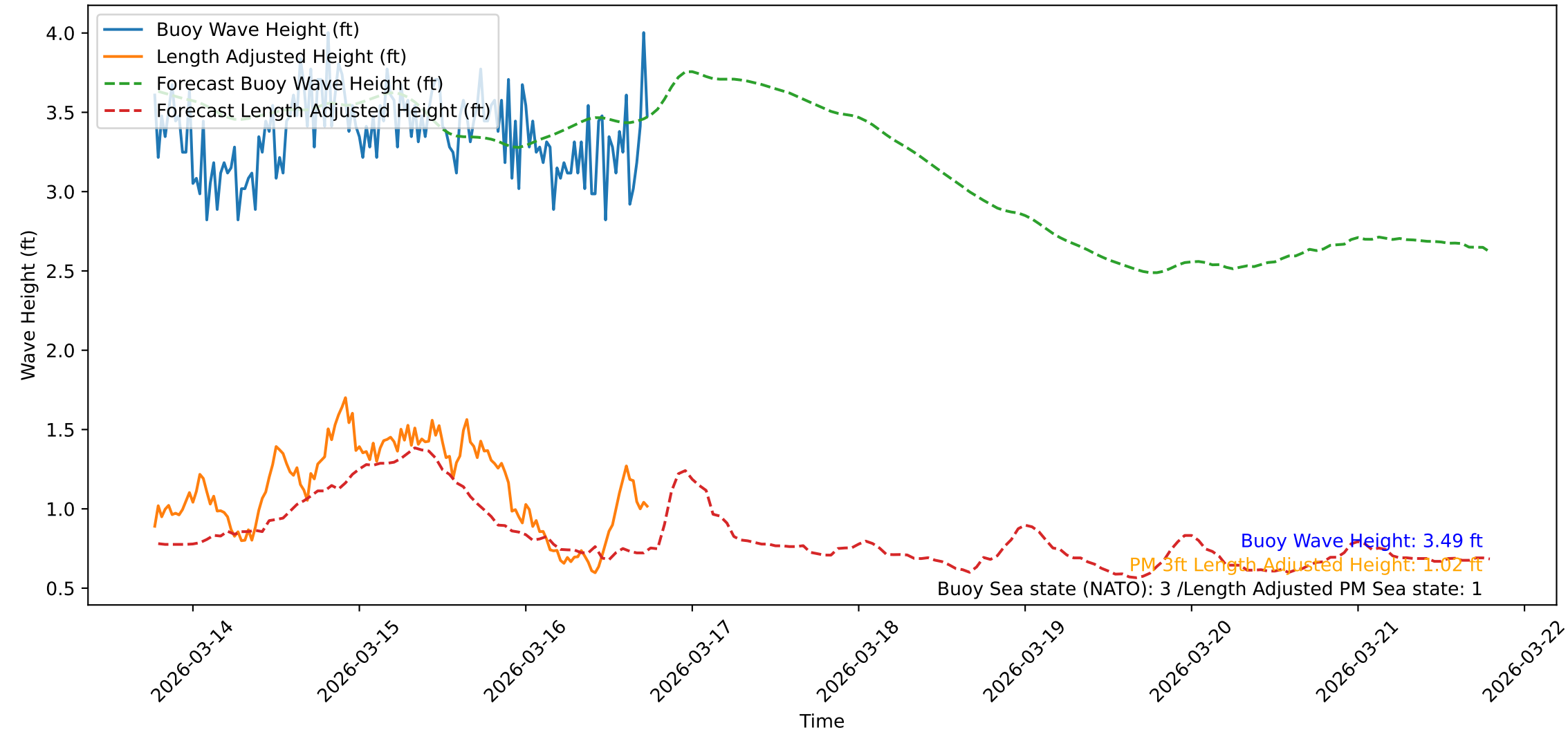
Wave Heights over Time for Green Beach at 2026-03-16 18:31:40
