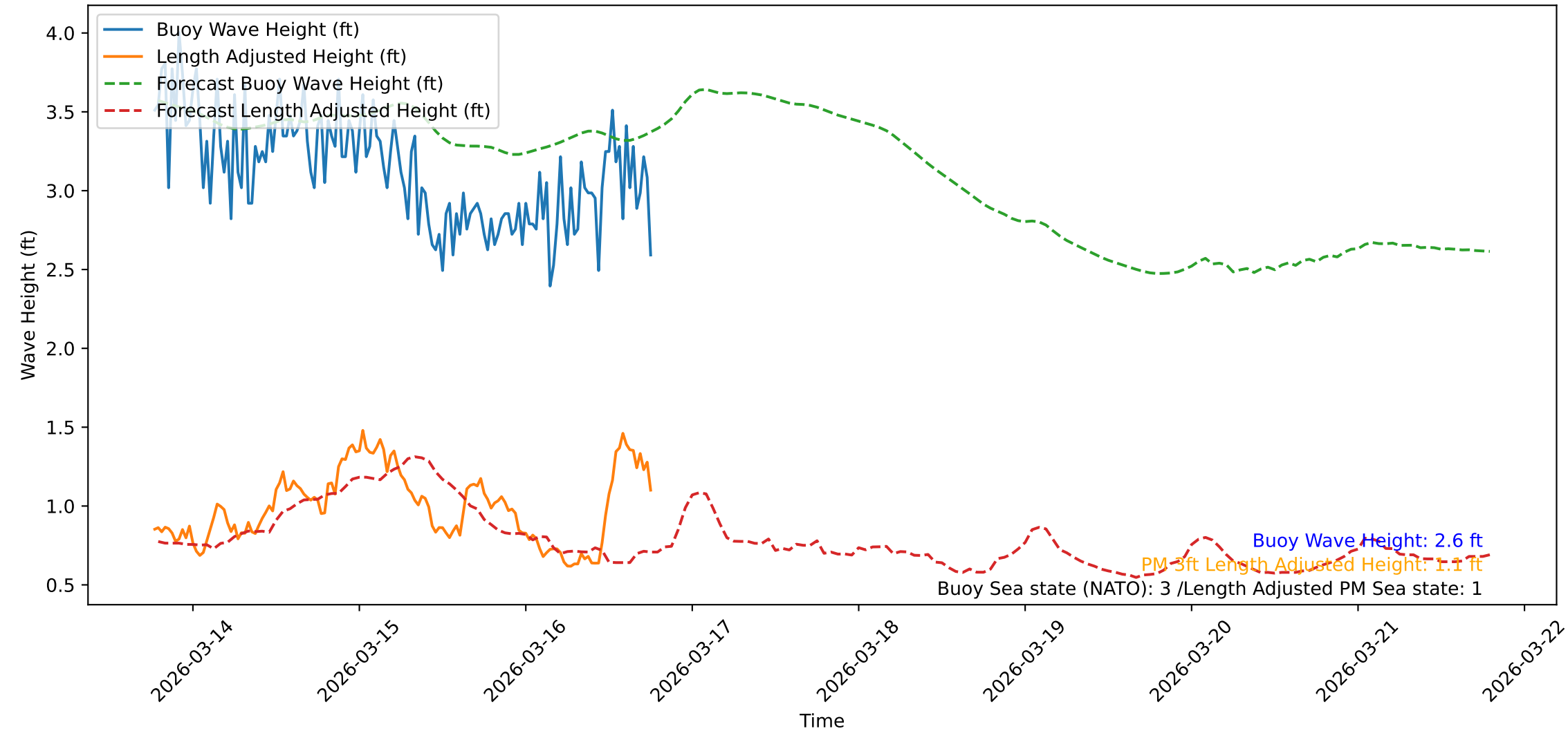
Wave Heights over Time for Oceanside Harbor at 2026-03-16 18:30:44
