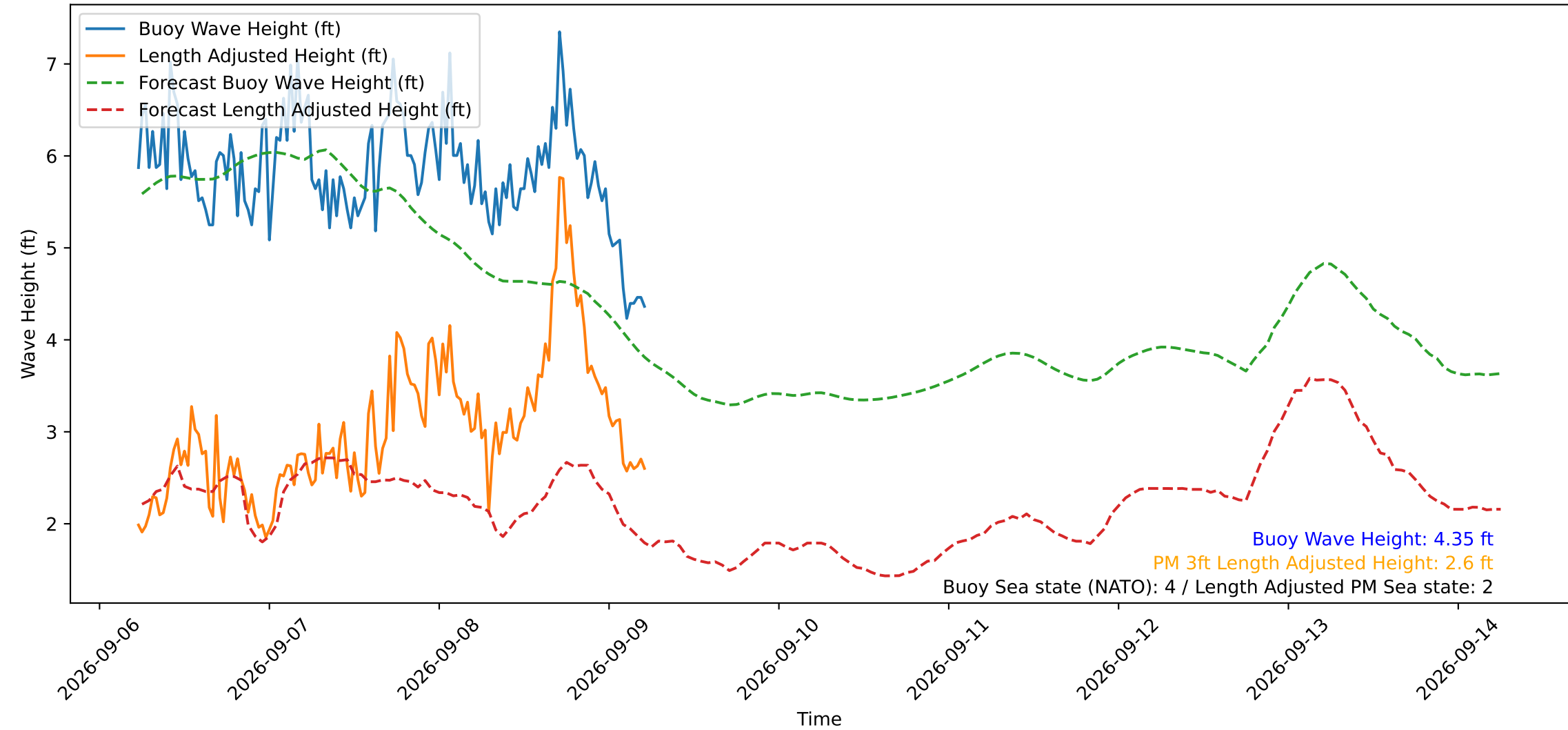
Wave Heights over Time for Oceanside Harbor at 2026-09-09 05:30:29
