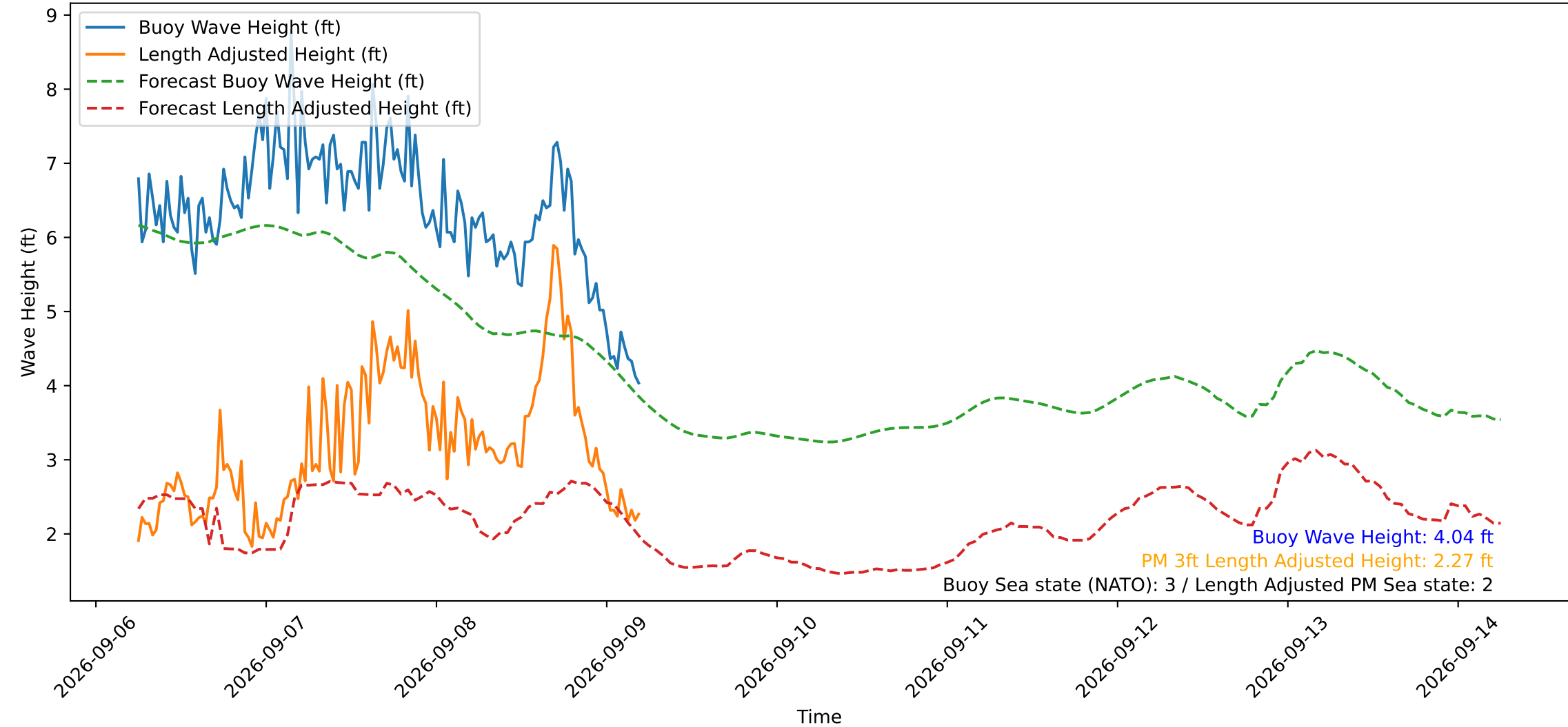
Wave Heights over Time for Green Beach at 2026-09-09 05:31:10
