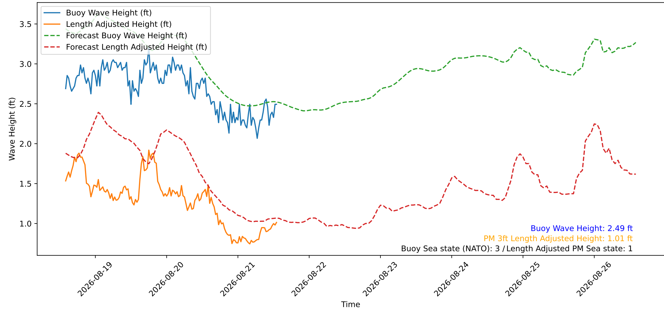
Wave Heights over Time for Red Beach at 2026-08-21 13:50:47
