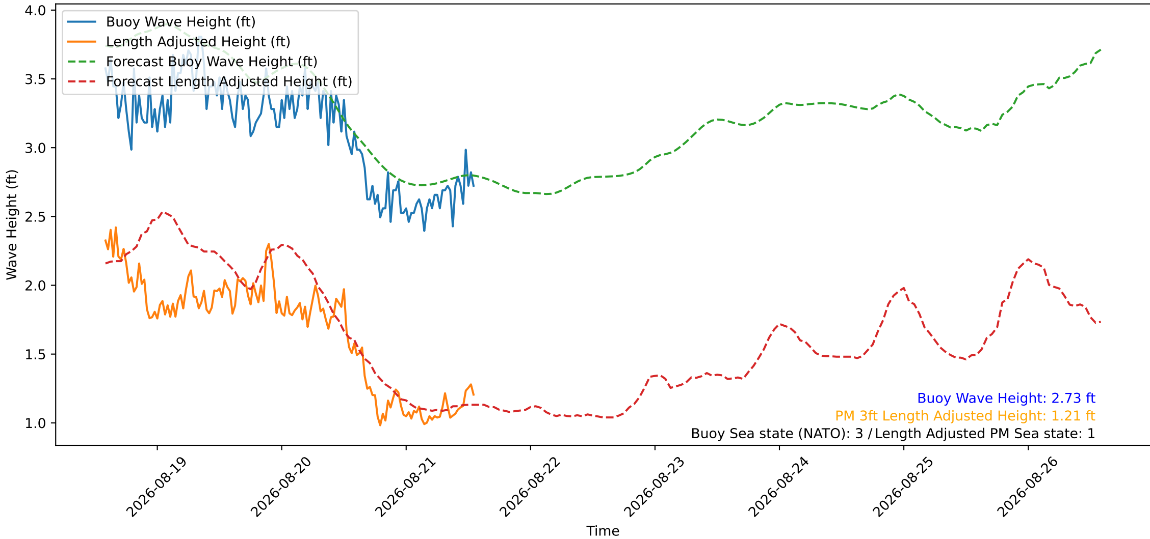
Wave Heights over Time for Oceanside Harbor at 2026-08-21 13:50:26
