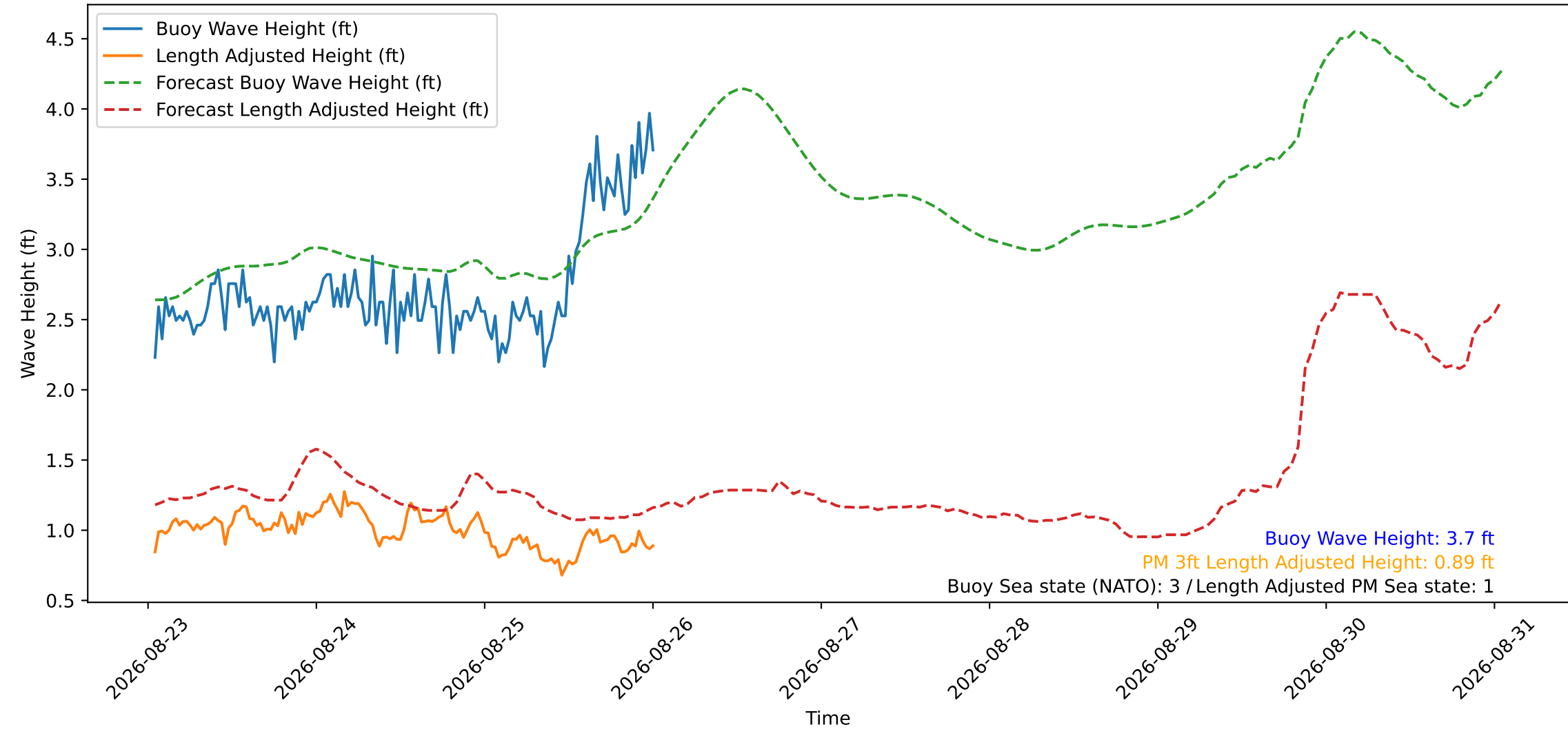
Wave Heights over Time for Red Beach at 2026-08-26 00:40:50
