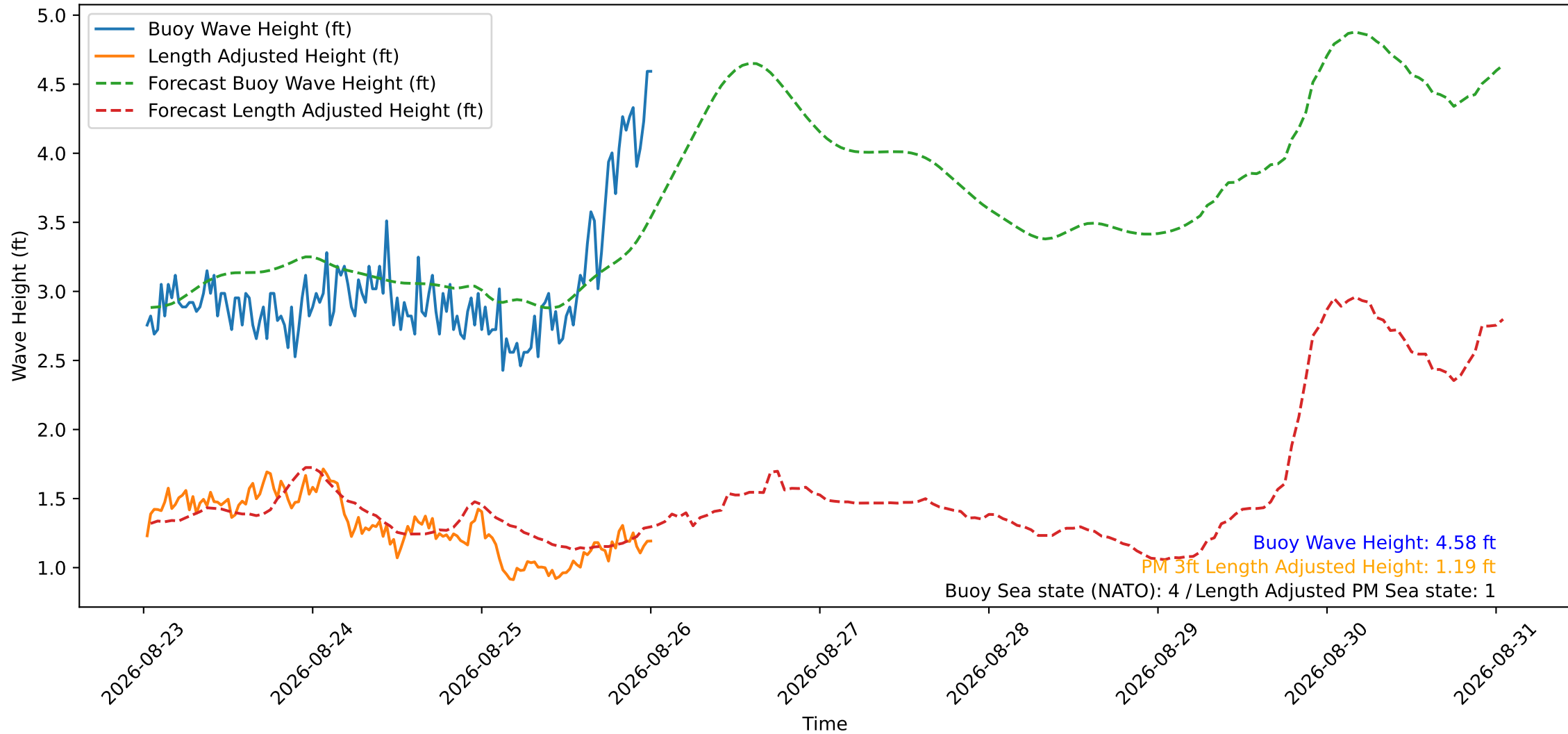
Wave Heights over Time for Oceanside Harbor at 2026-08-26 00:40:30
