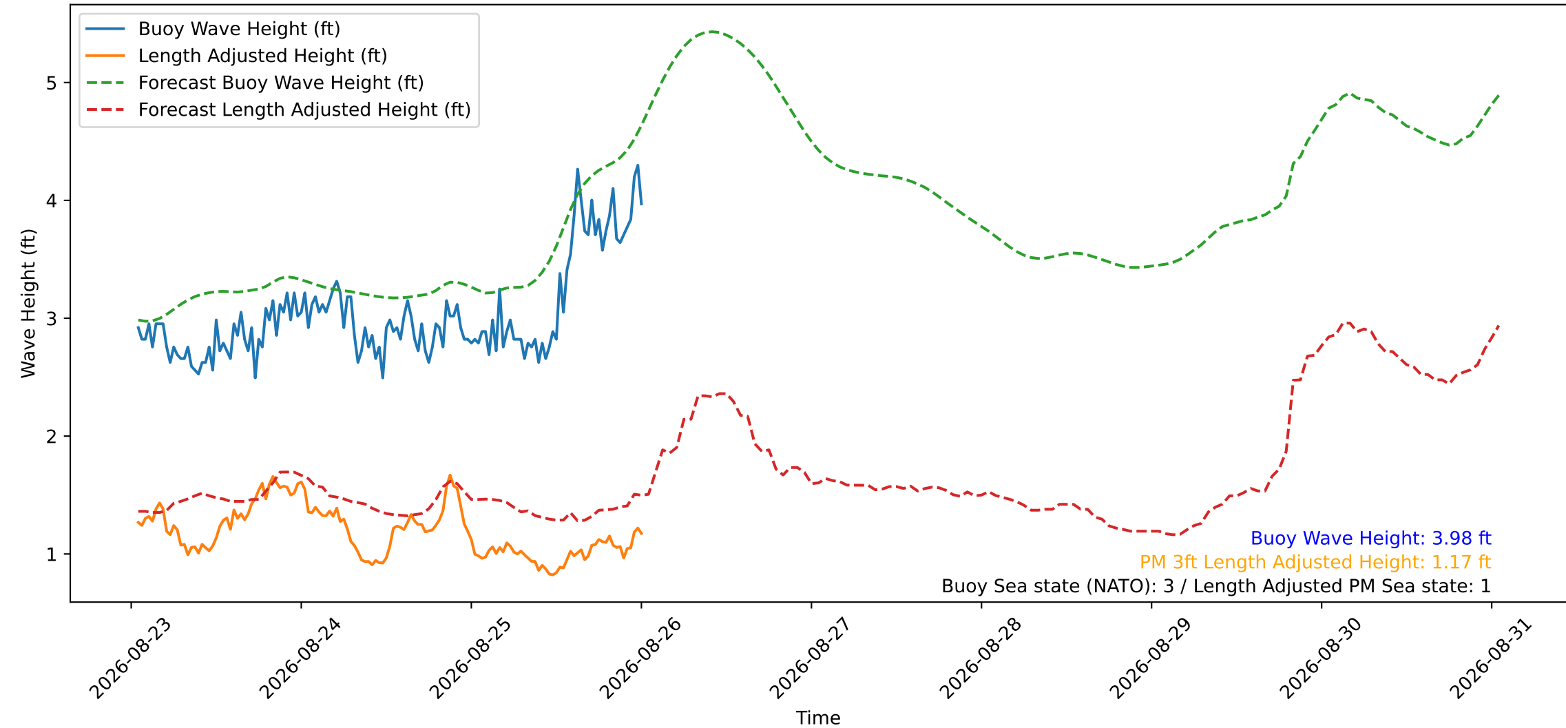
Wave Heights over Time for Green Beach at 2026-08-26 00:41:12
