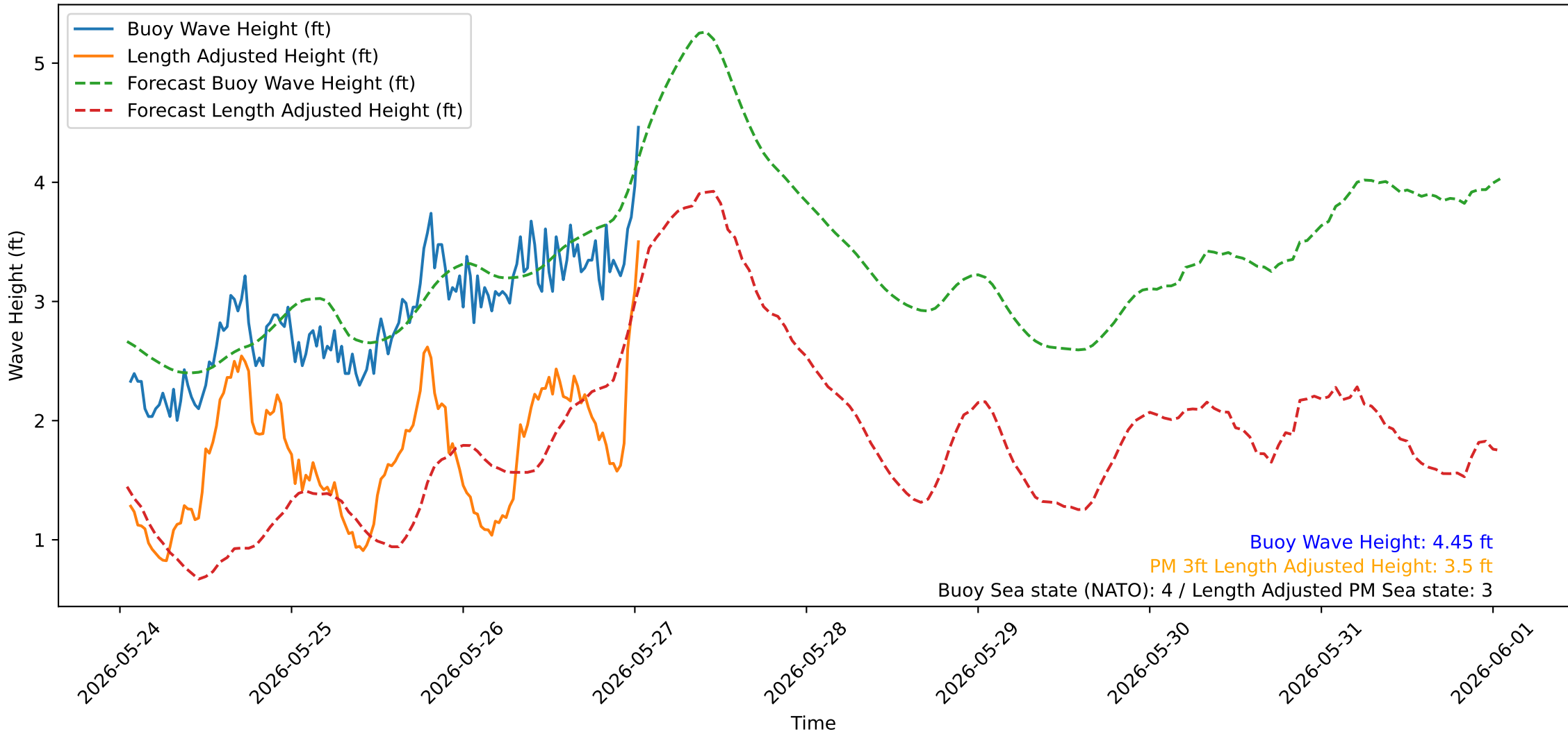
Wave Heights over Time for Red Beach at 2026-05-27 01:20:52
