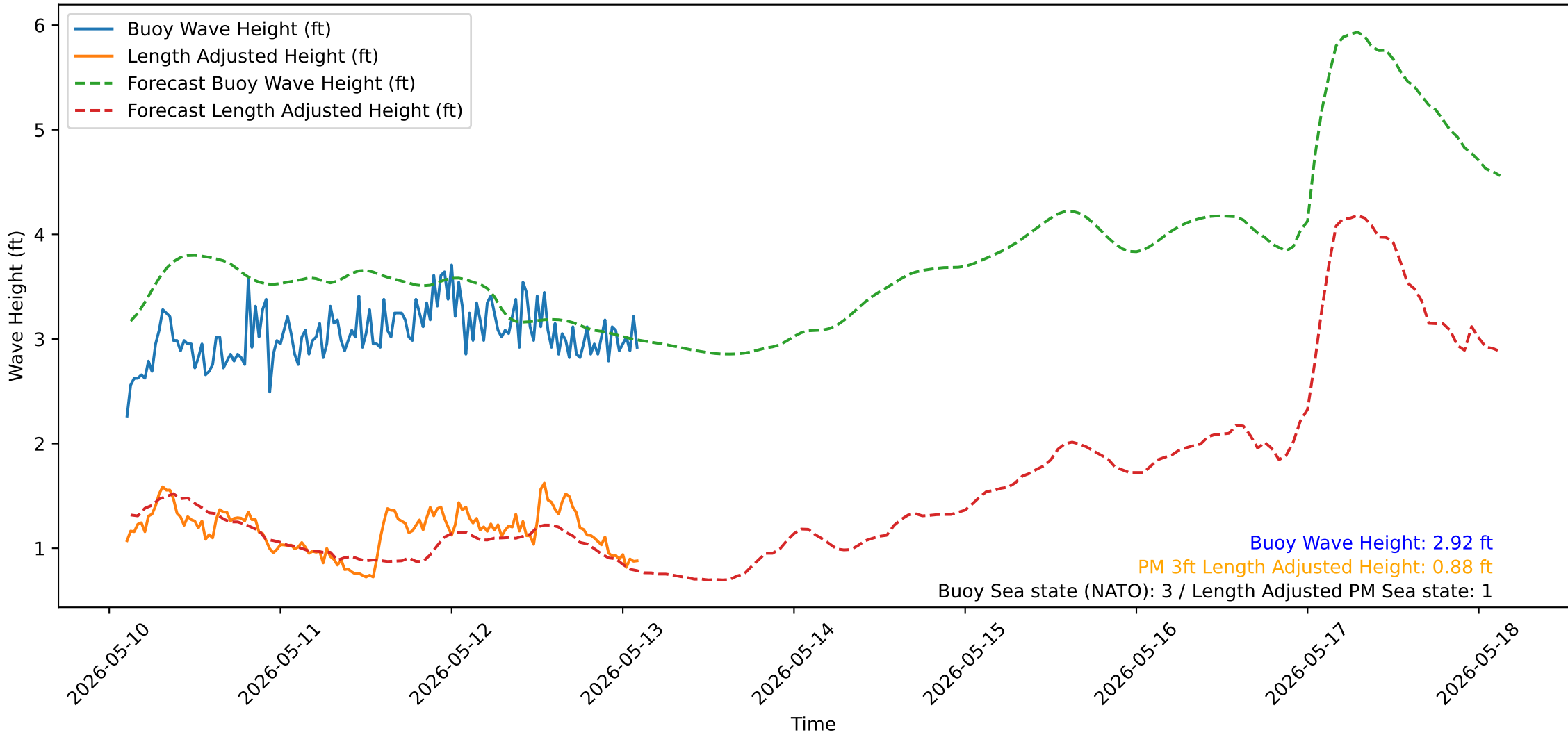
Wave Heights over Time for Oceanside Harbor at 2026-05-13 02:40:31
