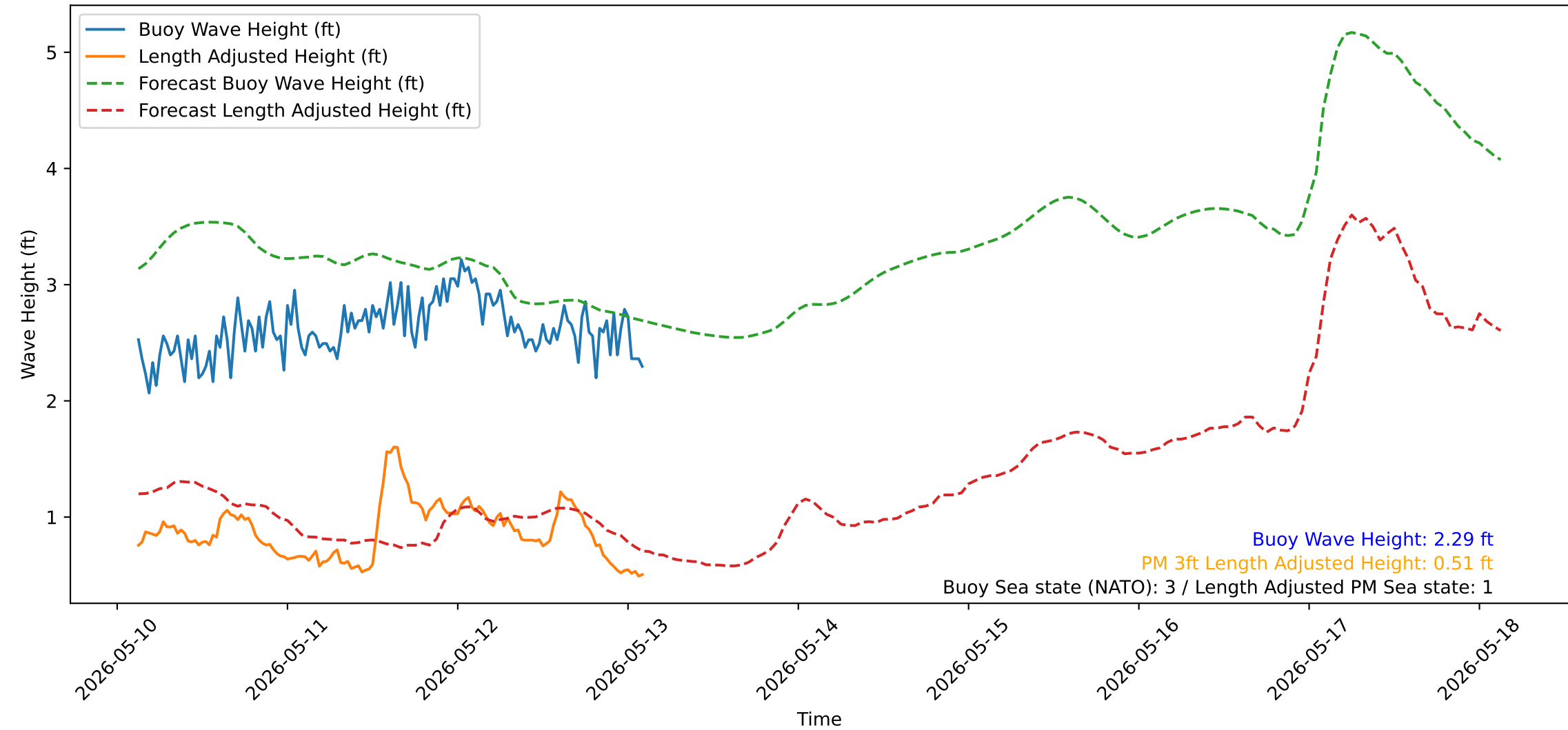
Wave Heights over Time for Red Beach at 2026-05-13 02:40:51
