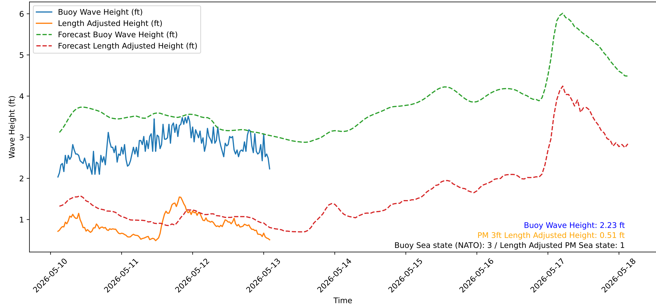
Wave Heights over Time for Green Beach at 2026-05-13 02:41:13
