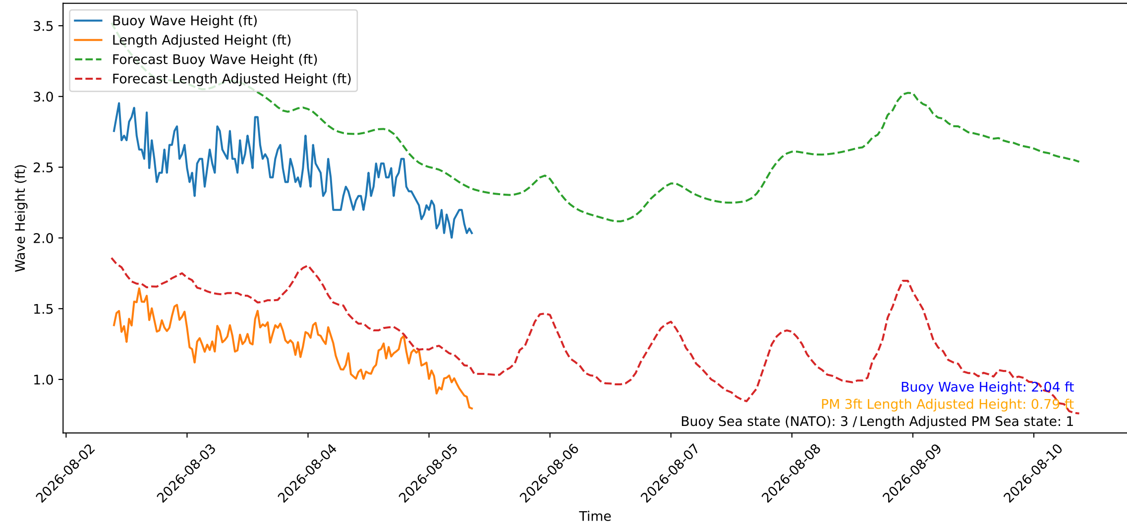
Wave Heights over Time for Oceanside Harbor at 2026-08-05 09:20:26
