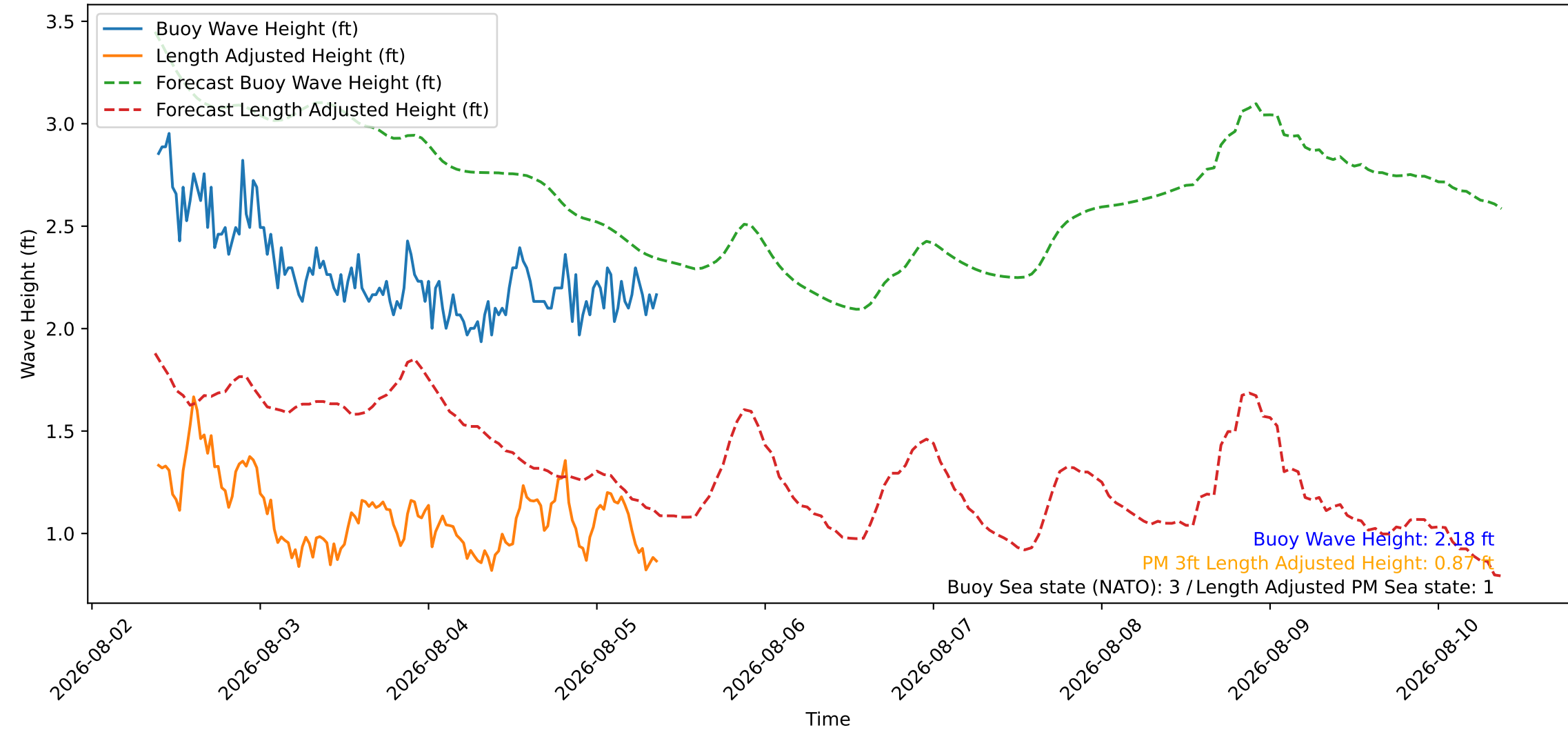
Wave Heights over Time for Green Beach at 2026-08-05 09:21:09
