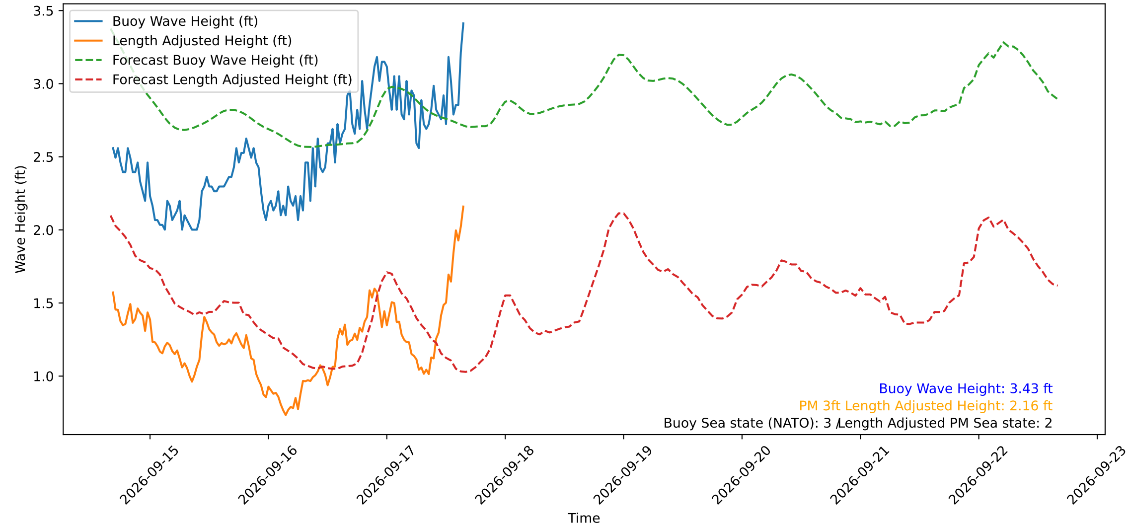
Wave Heights over Time for Red Beach at 2026-09-17 16:10:50
