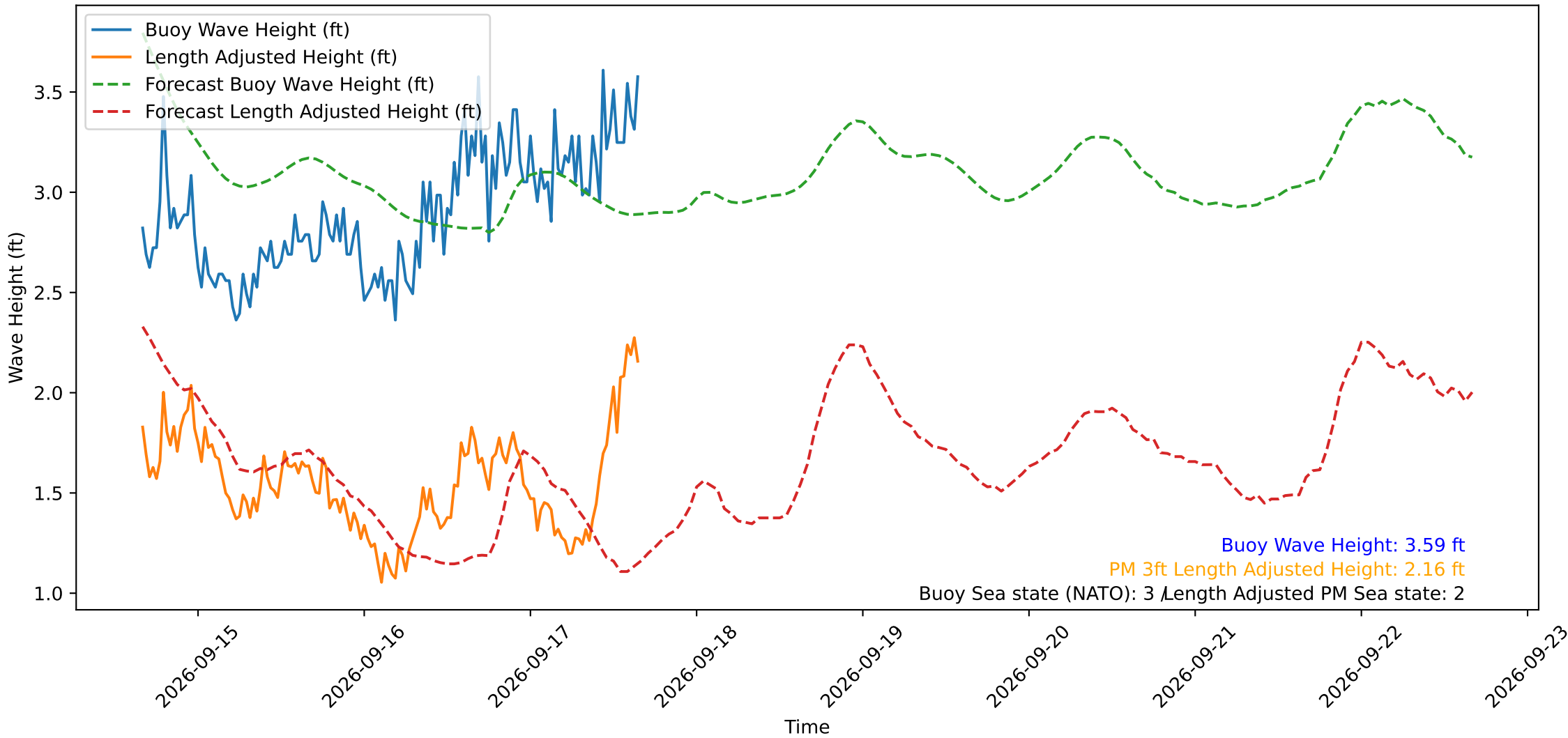
Wave Heights over Time for Oceanside Harbor at 2026-09-17 16:10:29
