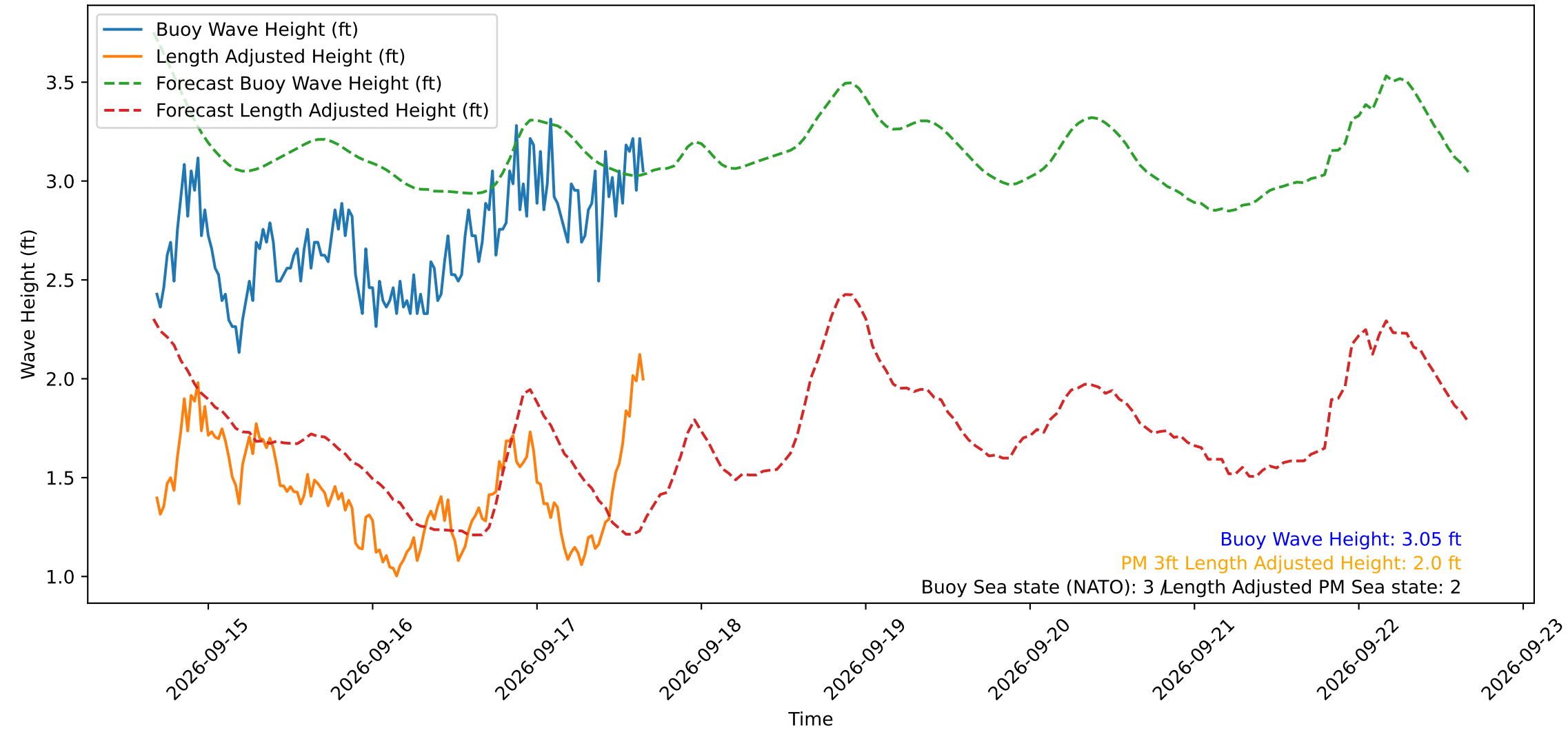
Wave Heights over Time for Green Beach at 2026-09-17 16:11:12
