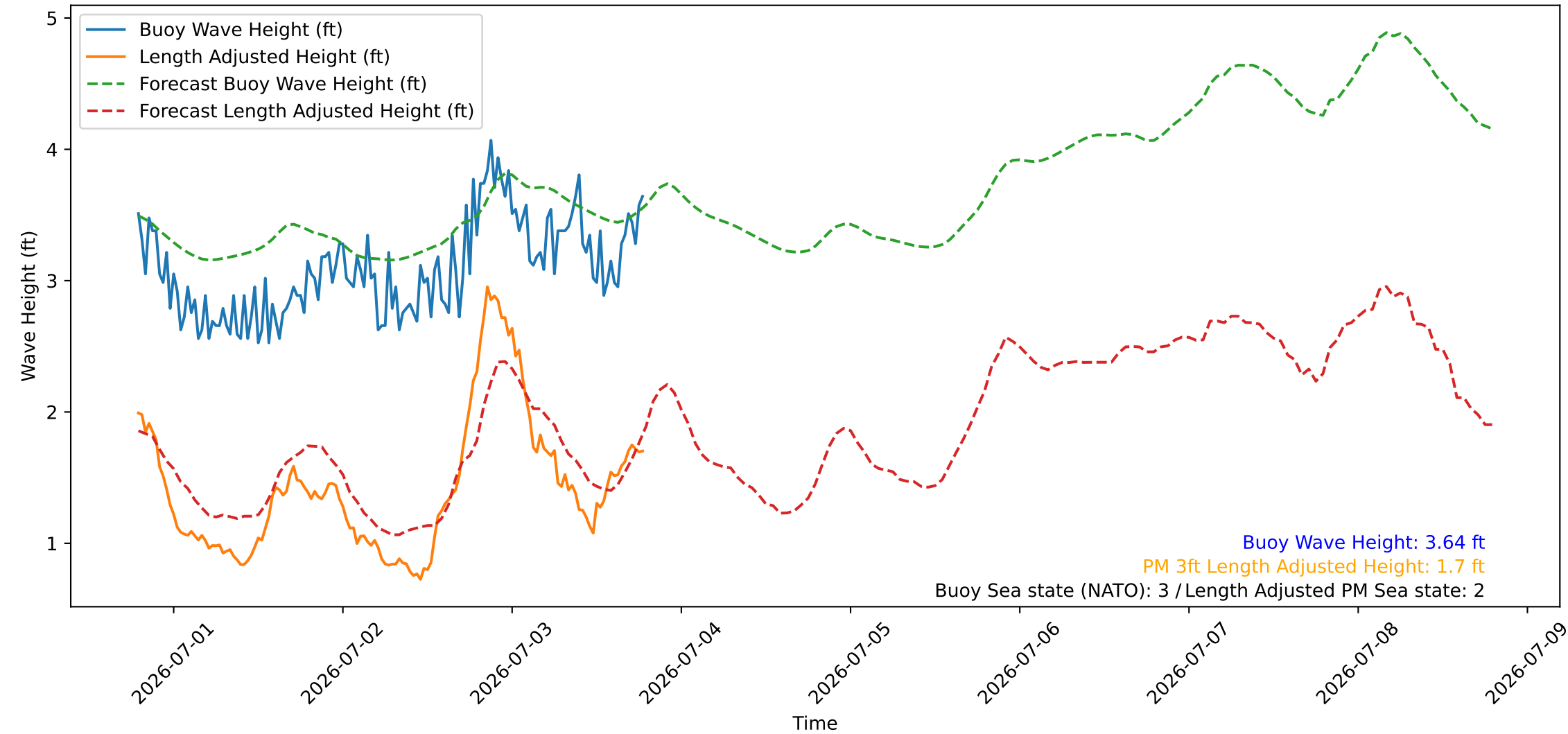
Wave Heights over Time for Green Beach at 2026-07-03 19:11:08
