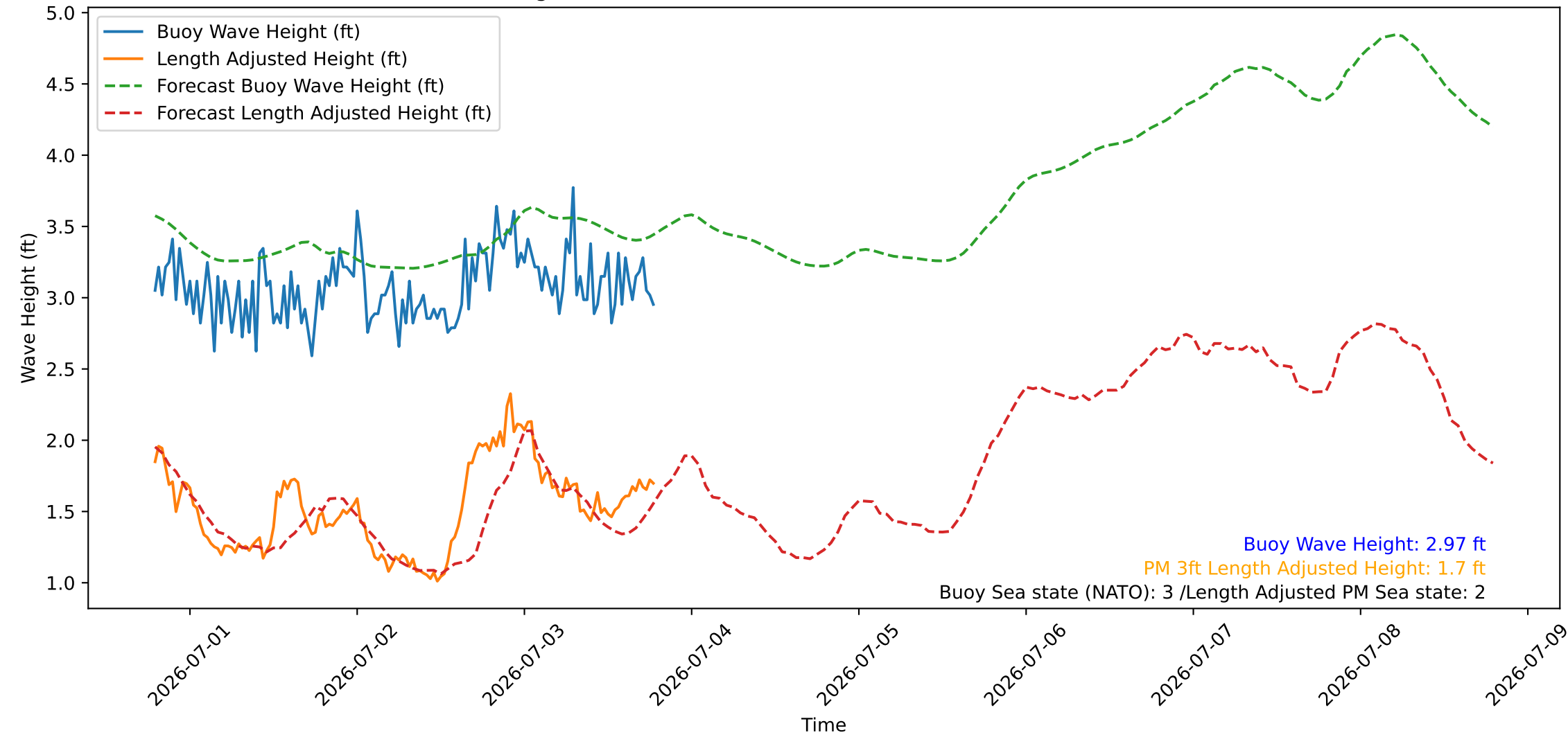
Wave Heights over Time for Oceanside Harbor at 2026-07-03 19:10:26
